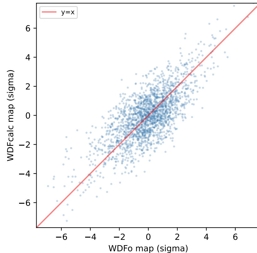
selection Scatter (CC=0.735)
