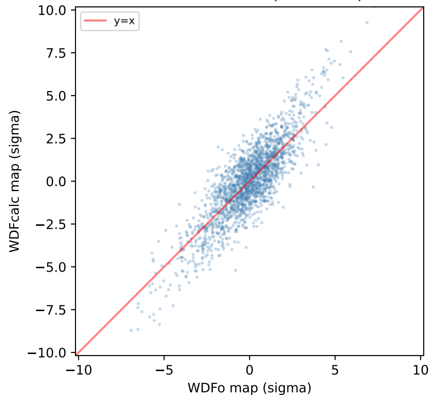
selection Scatter (CC=0.849)
