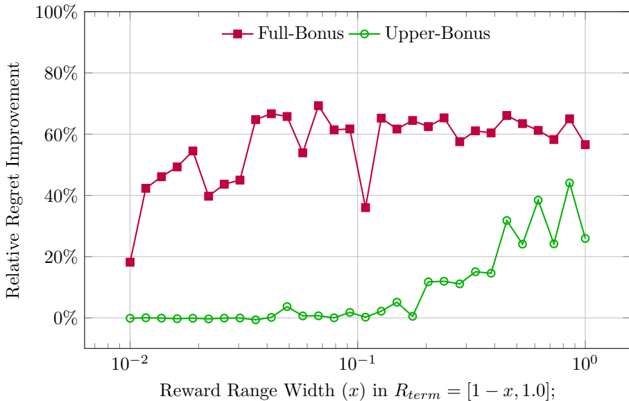
Expanding Reward: Bonus Shaping Comparison
