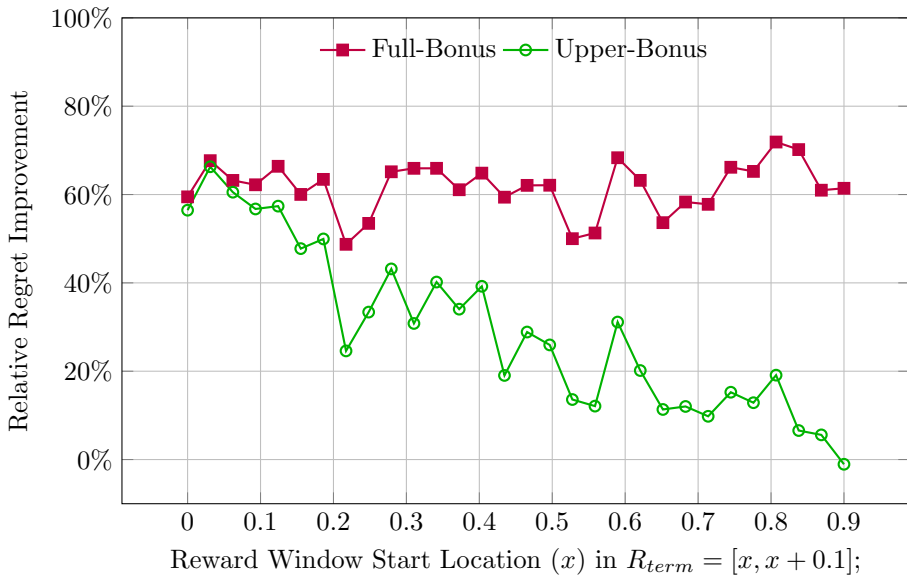
Sliding Window: Bonus Shaping Comparison
