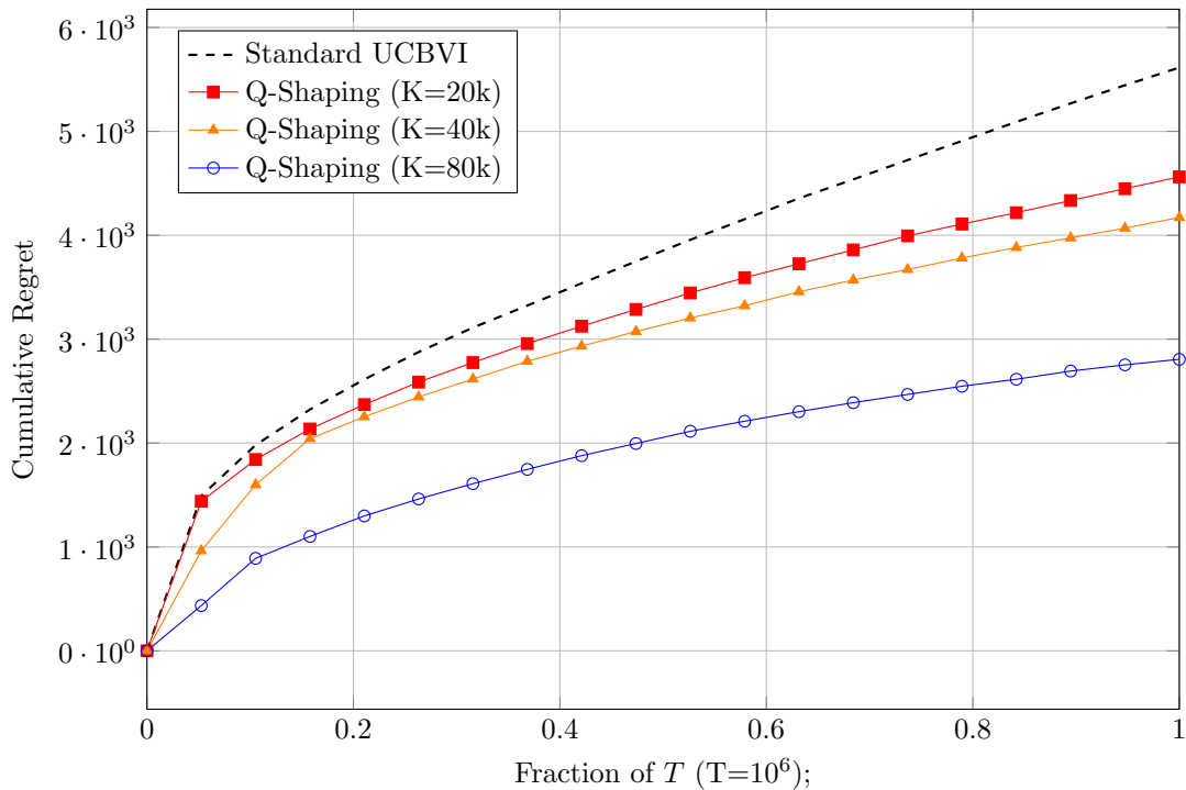
Q-Shaping Performance vs. Offline Data Size (K)
