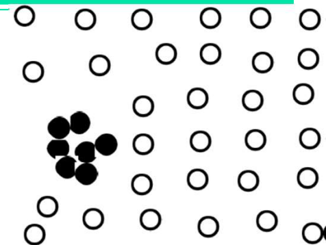
Collective Outlier
