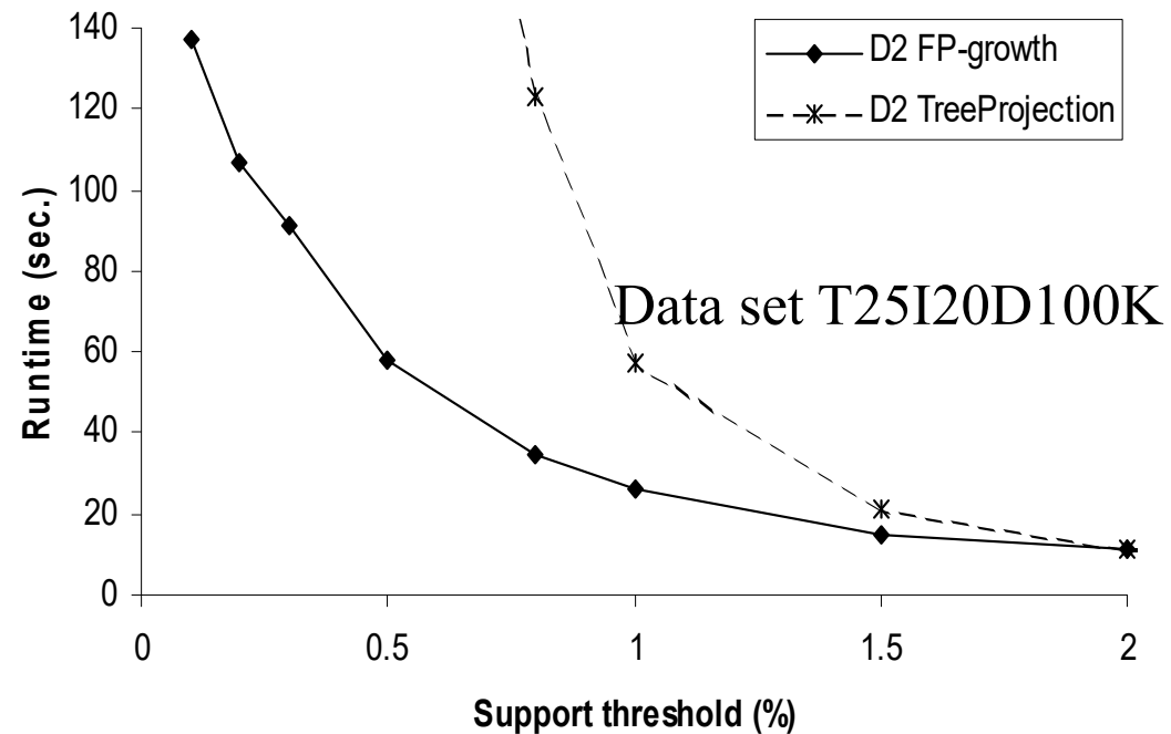
FP-Growth vs. Tree-Projection
