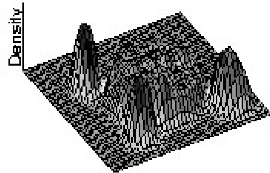
(c) Gaussian
