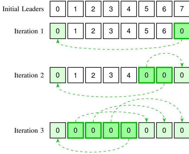
Fig. 7: Convergence of the Parallel Pointer Jumping algorithm on an 8-element cycle. The diagram illustrates label propagation ( L ) where the minimum identifier (0) is distributed across the array. Highlighted cells indicate nodes that adopted the leader’s index during the current iteration.
