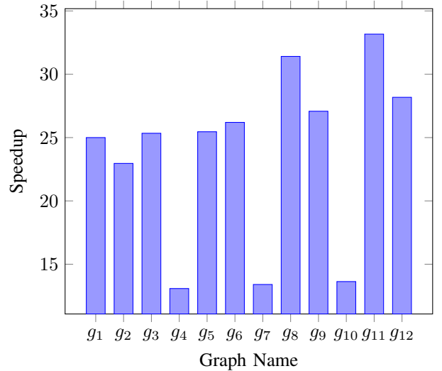
Fig. 11: Speedup between our CPU and the GPU HE-based implementations on different graphs
