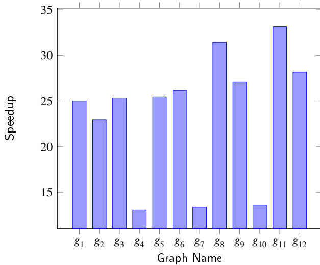
Figure 11: Speedup between our CPU and the GPU HE-based implementations on different graphs
