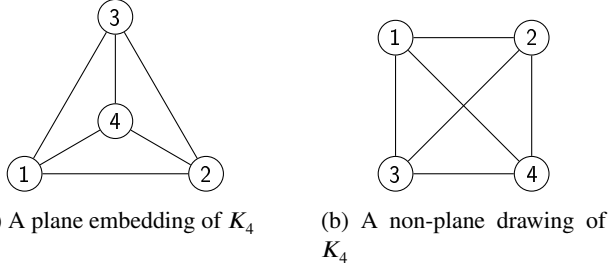
Figure 2: Verification of the planarity of K_4 : (a) provides a valid plane embedding, while (b) illustrates a drawing with a crossing that does not alter the graph's underlying planarity.
