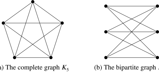
Figure 1: The two minimal non-planar graphs shown with unavoidable edge crossings.
