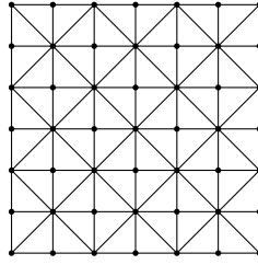
Figure 8: Pattern 1 of graphs for a grid of 7 \times 7 vertices
