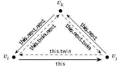
Figure 4: An illustration of half-edges and their twin edges of a triangle
