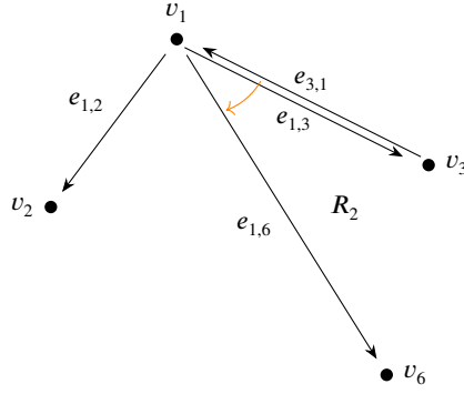
Figure 6: Next Edge Linking. The next edge of e_{3,1} points to the half-edge e_{1,6} based on the angular order around v_1 .
