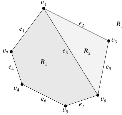
Figure 3: Plane graph with seven edges forming three regions.
