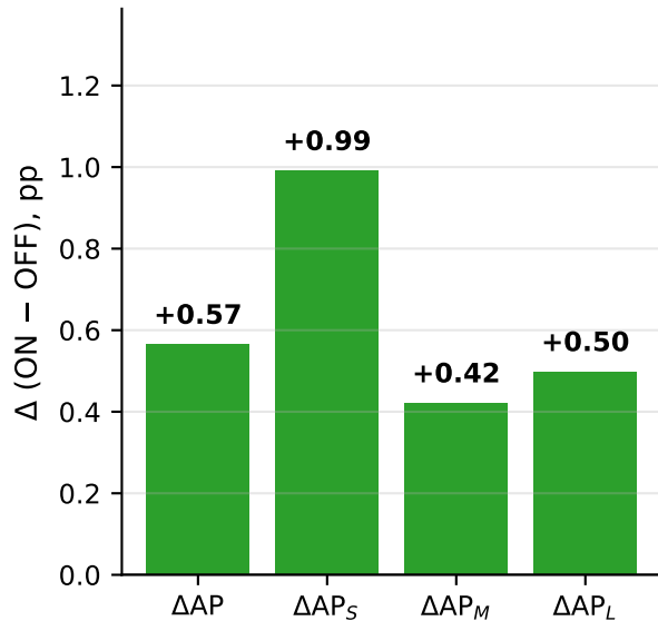
Causal contribution
