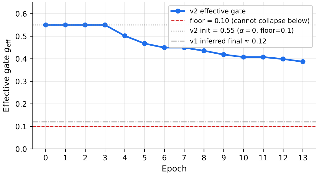
Gate trajectory: v2 stays meaningful, v1 collapses
