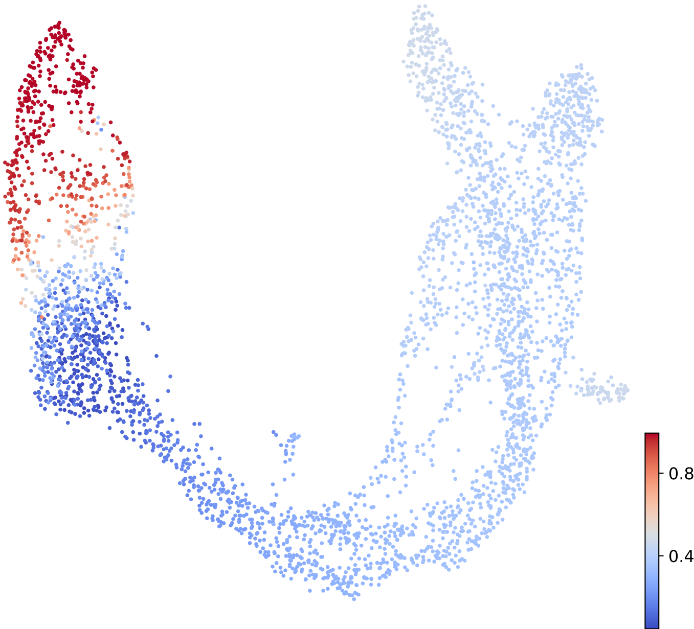
velocity pseudotime
