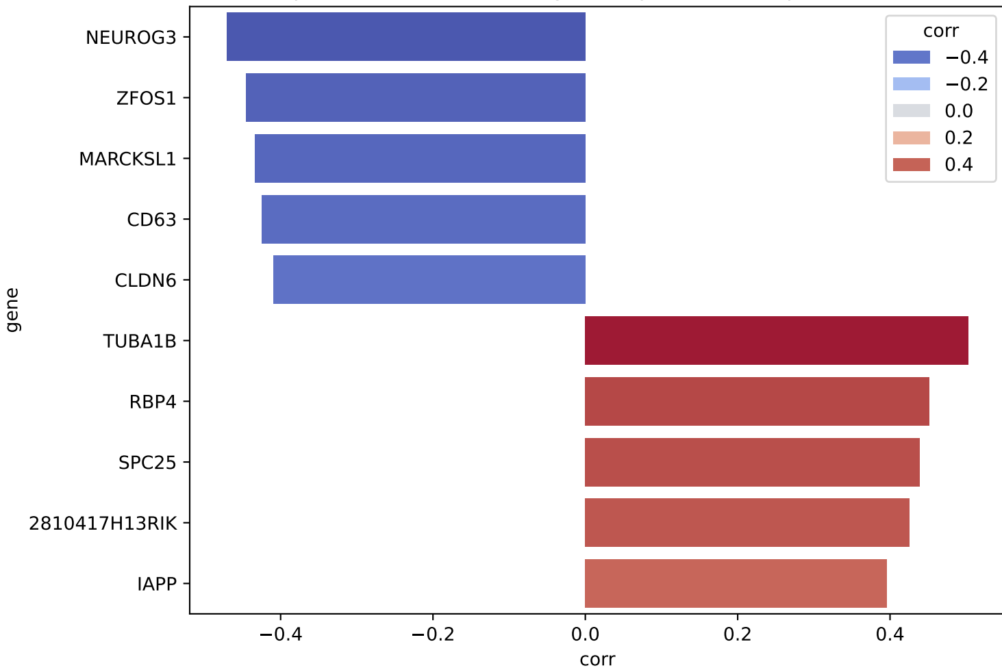
Spearman correlation of gene expression and pseudotime
