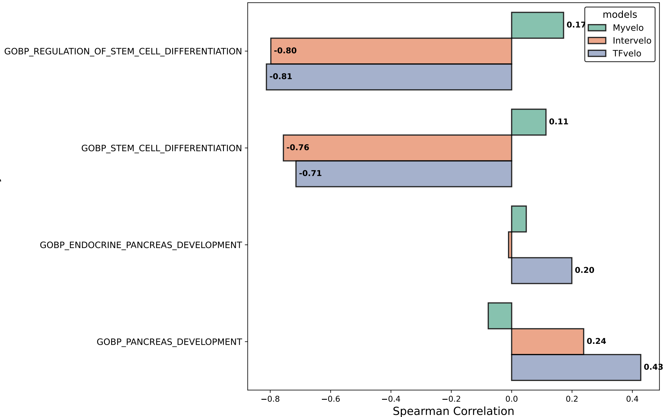
Correlation of GSVA Pathway Score with Pseudotime
