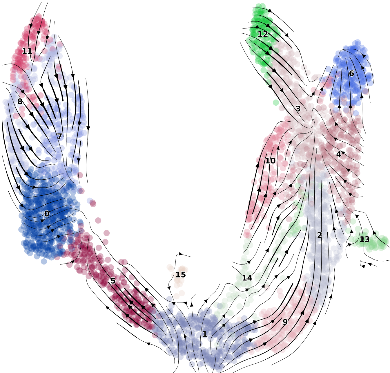
RNA Velocity Trajectory
