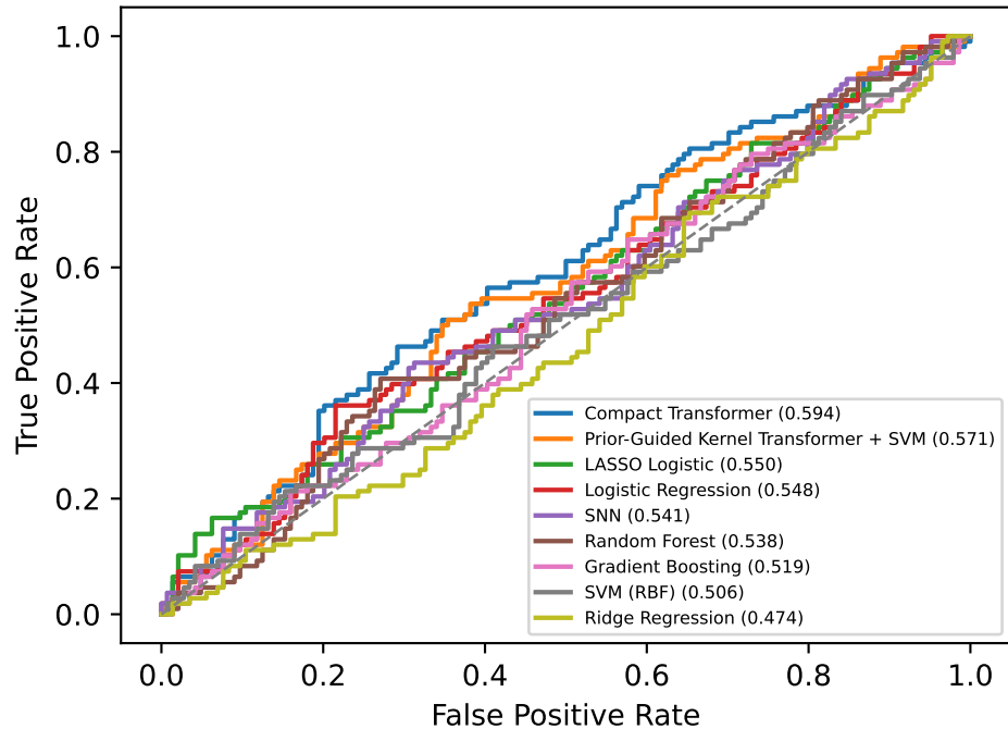
External ROC (1Y)
