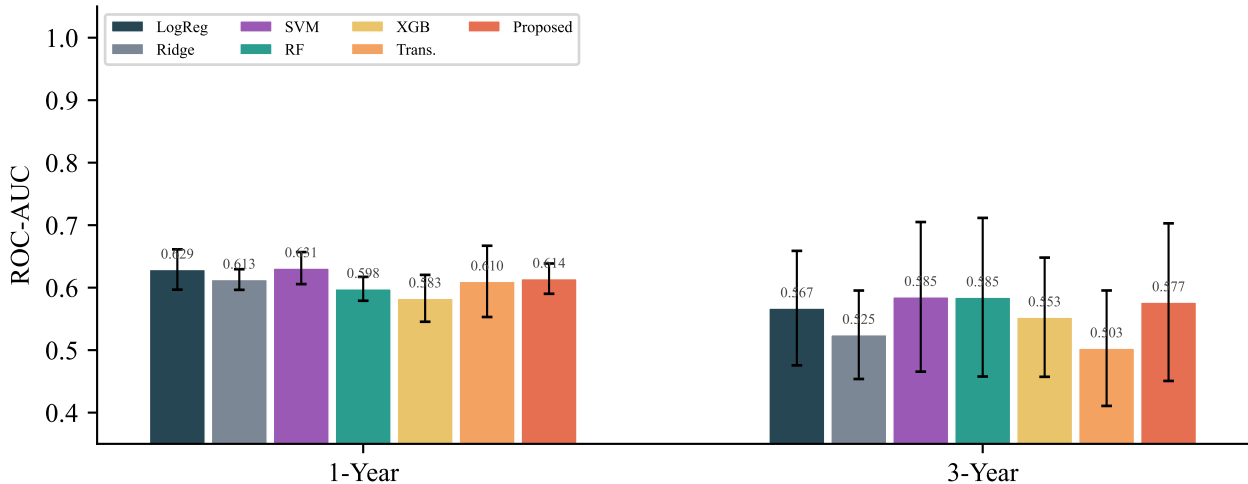
GBM Survival Benchmark (CPTAC+TCGA)
