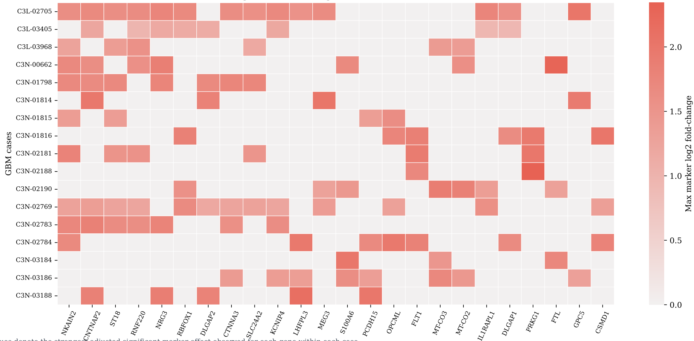
Recurrent GBM single-cell marker genes across the 17-case scRNA cohort
