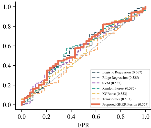
3-Year Survival ROC
