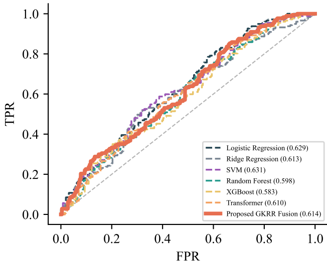
1-Year Survival ROC
