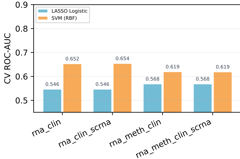
CPTAC Ablation 1Y
