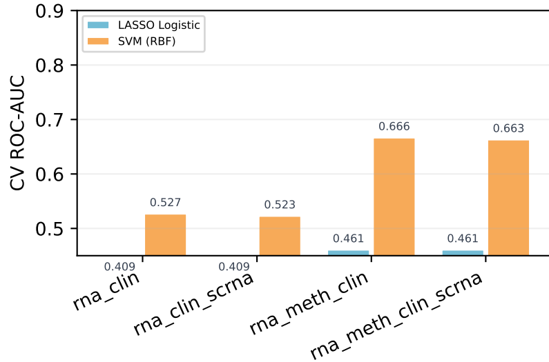
CPTAC Ablation 3Y
