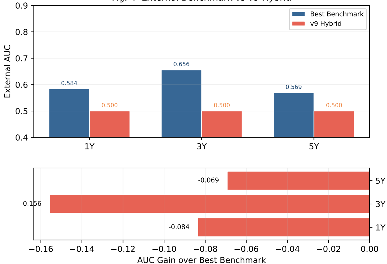
Fig. 4 External Benchmark vs v9 Hybrid
