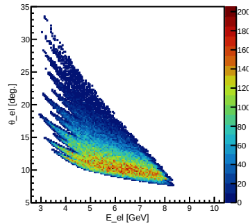
Data: 123 bins: 0.3 < \cos\theta_{pq}
