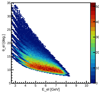
Data: 123 bins: Full range
