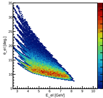
Data: 123 bins: -0.3 < \cos\theta_{pq} < 0.3
