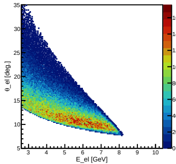
Data: 123 bins: \cos\theta_{pq} < -0.3
