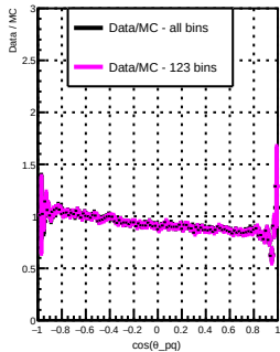
\cos\theta_{pq} : full range
