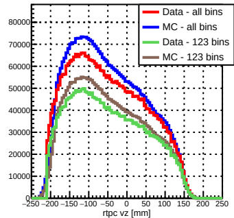
No cut
