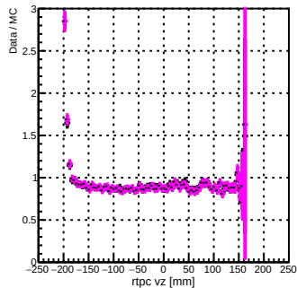
-0.3 < \cos\theta_{pq} < 0.3
