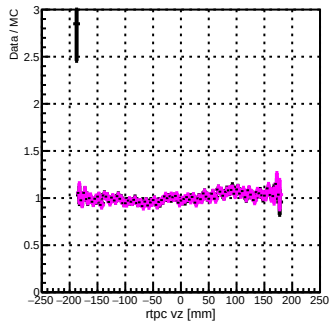
\cos\theta_{pq} < -0.3
