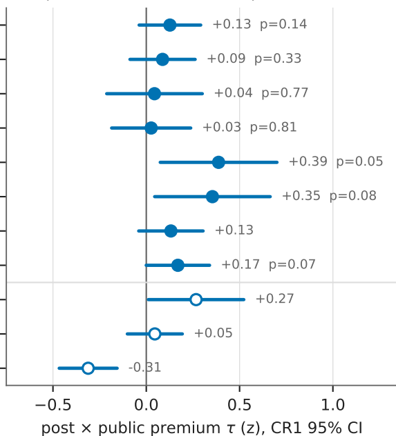
(b) Specifications (filled) and placebo cutoffs (open)
