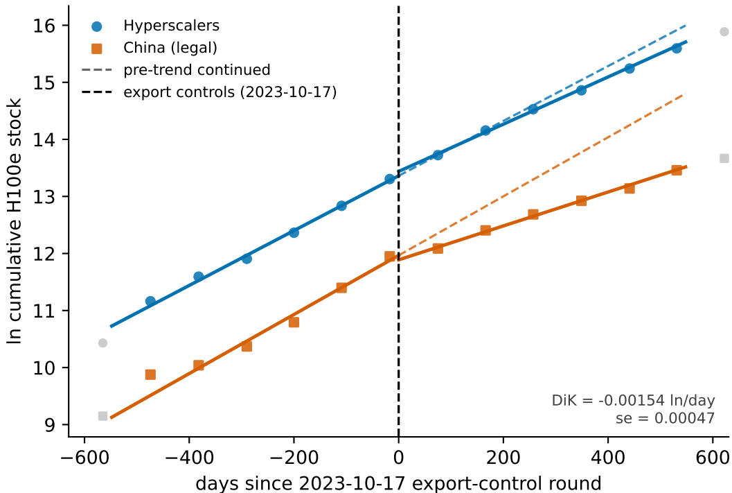
China vs hyperscalers: group difference-in-kinks (bw 548 d, triangular)
