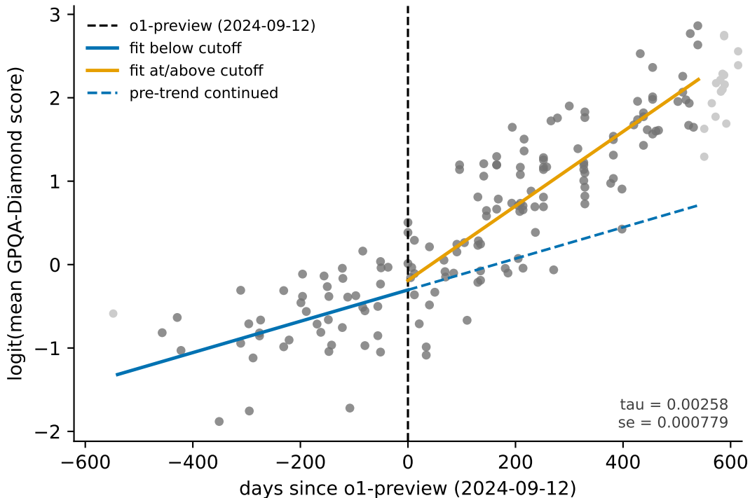
GPQA-Diamond: sharp RKD in calendar time (bw 540 d, triangular)
