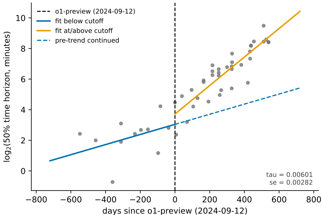
METR 50% time horizon: sharp RKD in calendar time (bw 720 d, triangular)
