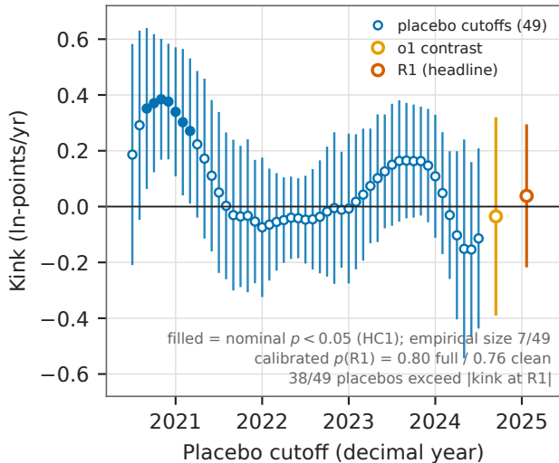
(b) R1 kink vs. placebo distribution
