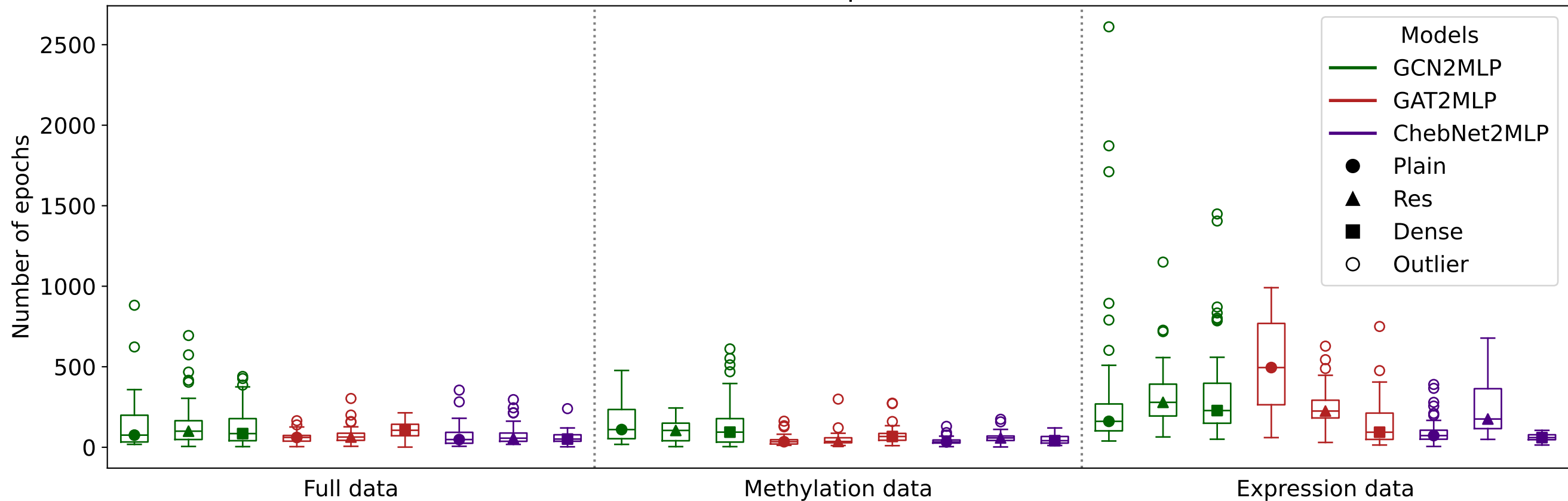
Test results over all outer splits - ONLY NEW MODELS
