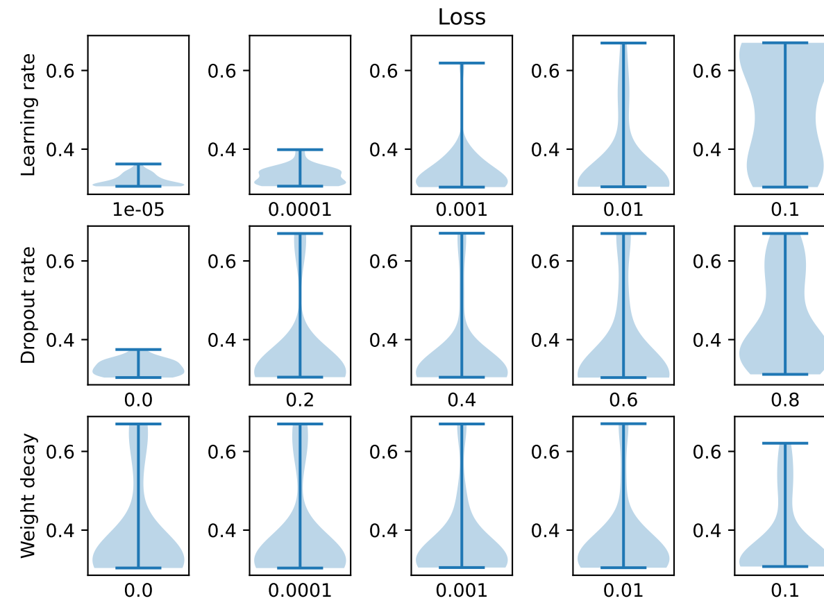
MLP (batch size 64)
