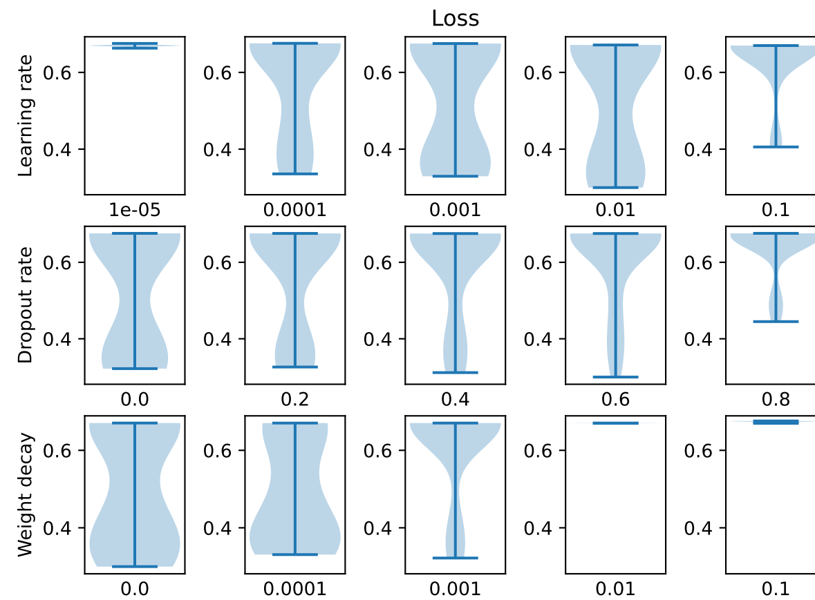
DenseGCN (full batch)
