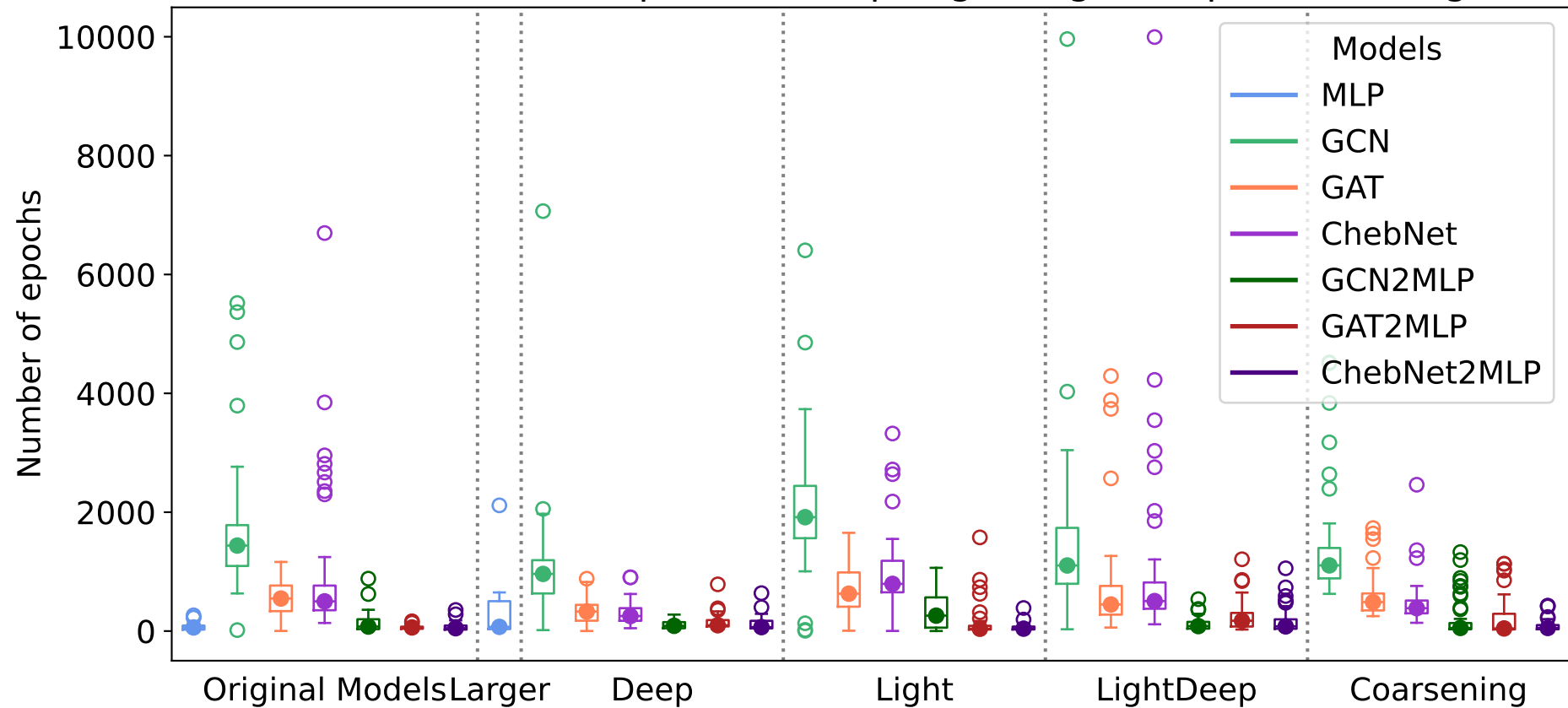
Test results over all outer splits for Deep, Light, LightDeep, Coarsening models
