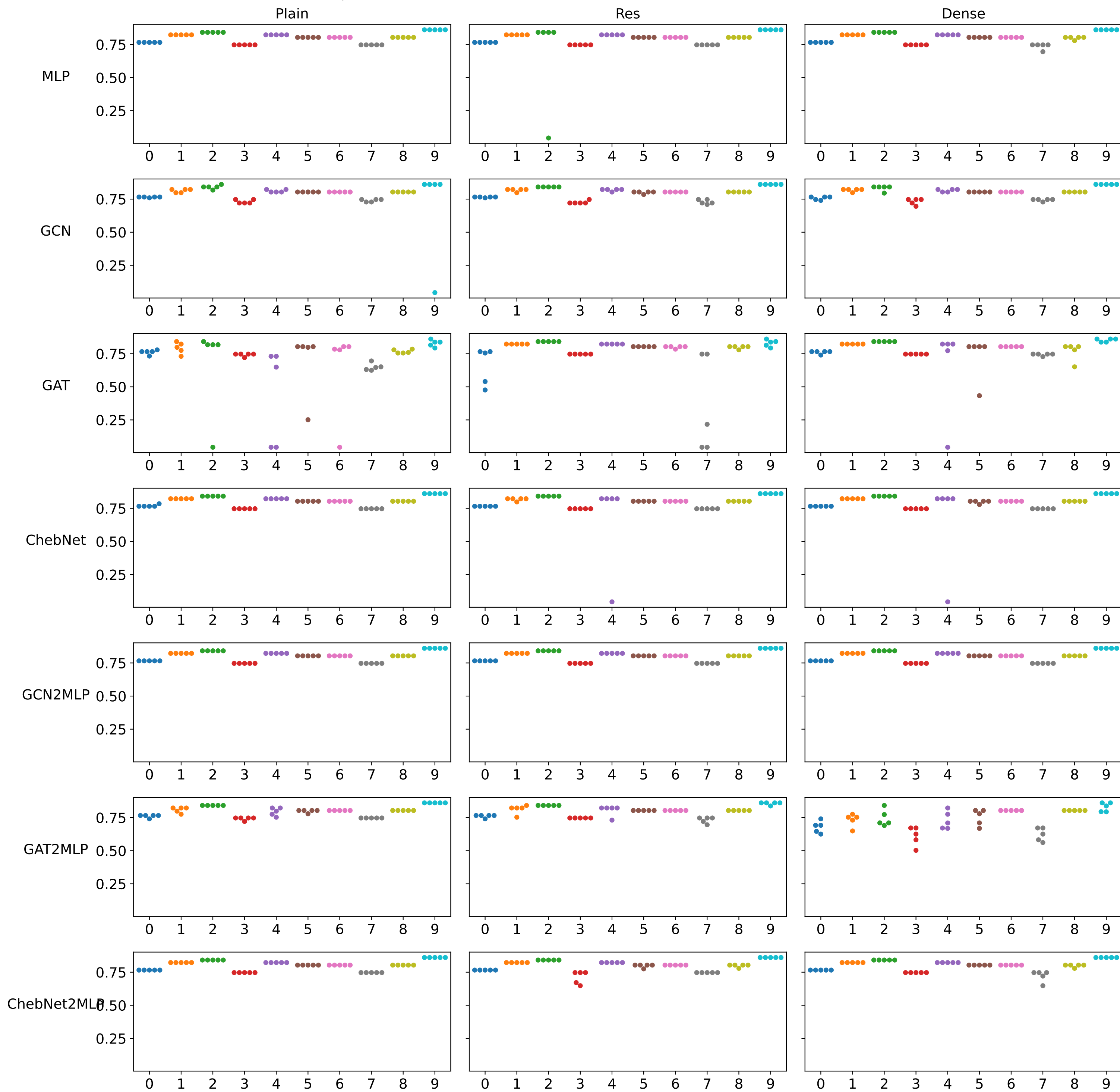
Results per outer test round in MCC for full data - INCL. NEW MODELS
