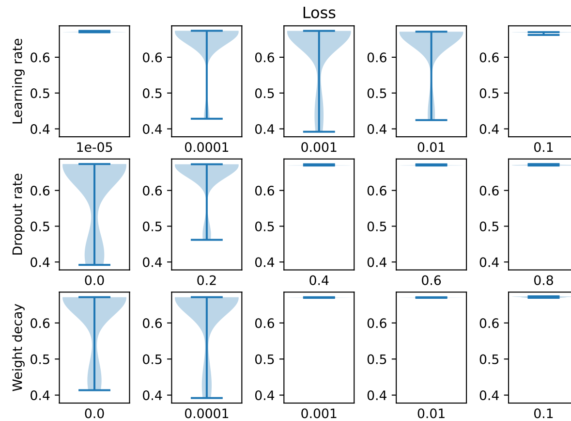
ResGCN (only expression data)
