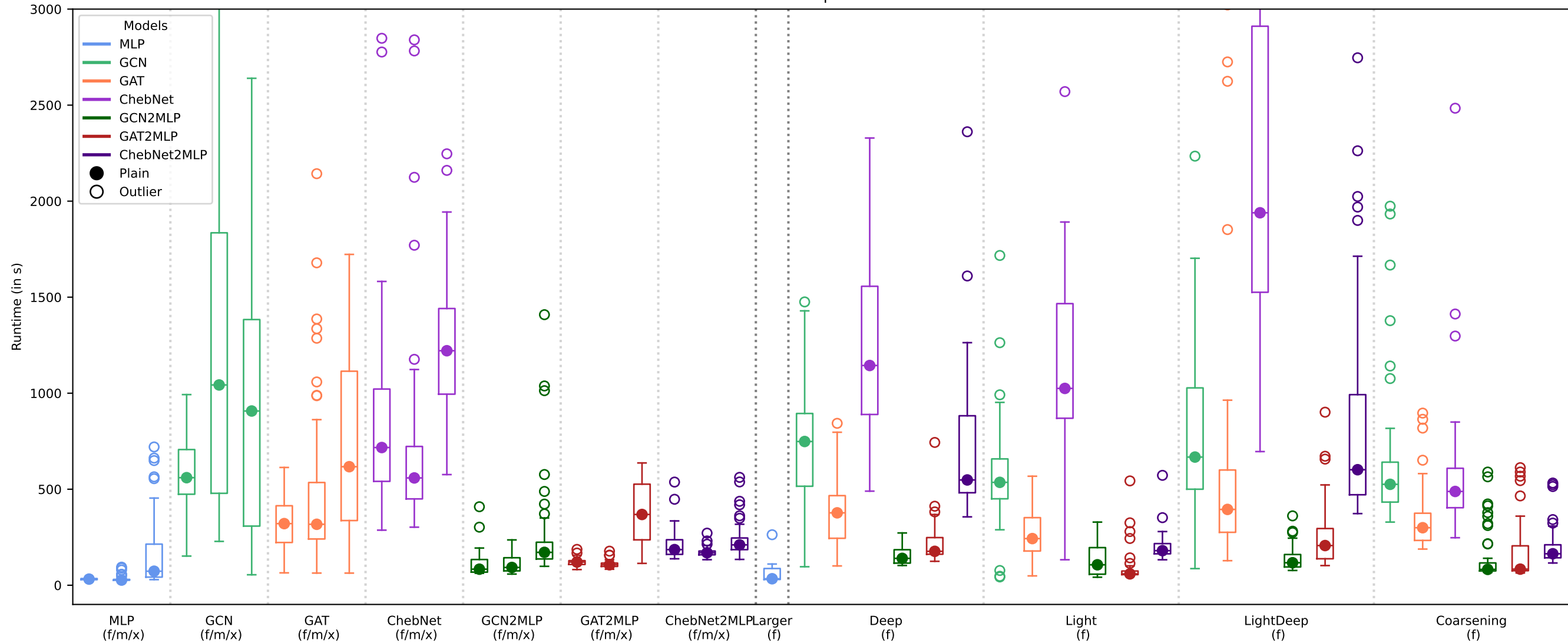
Run time over all outer splits for all Plain models
