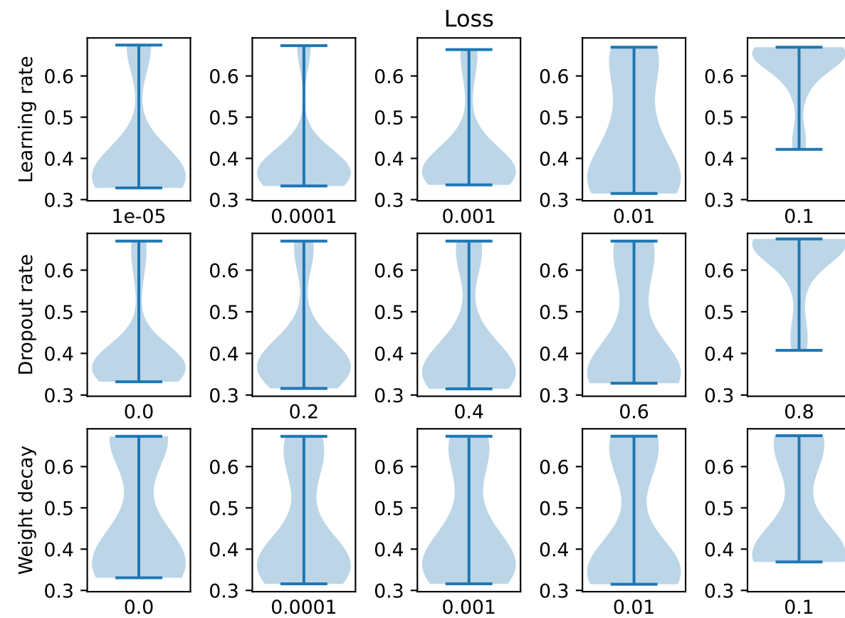
MLP (only expression data)
