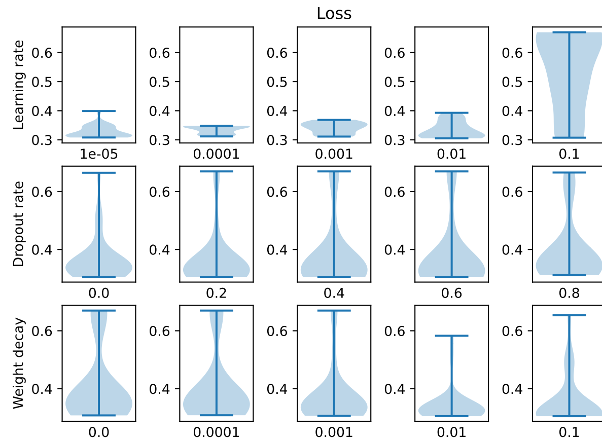
MLP (full batch)
