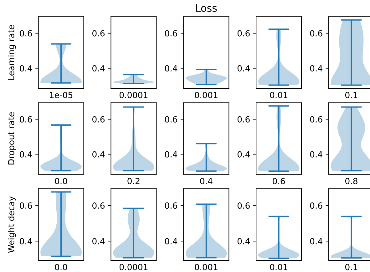
ResMLP (only methylation data)
