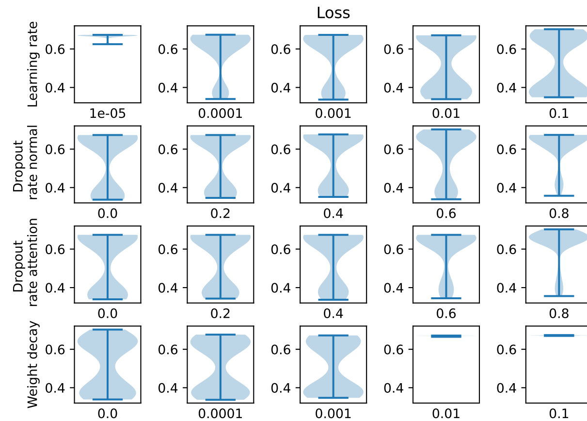
DenseGAT (only methylation data)
