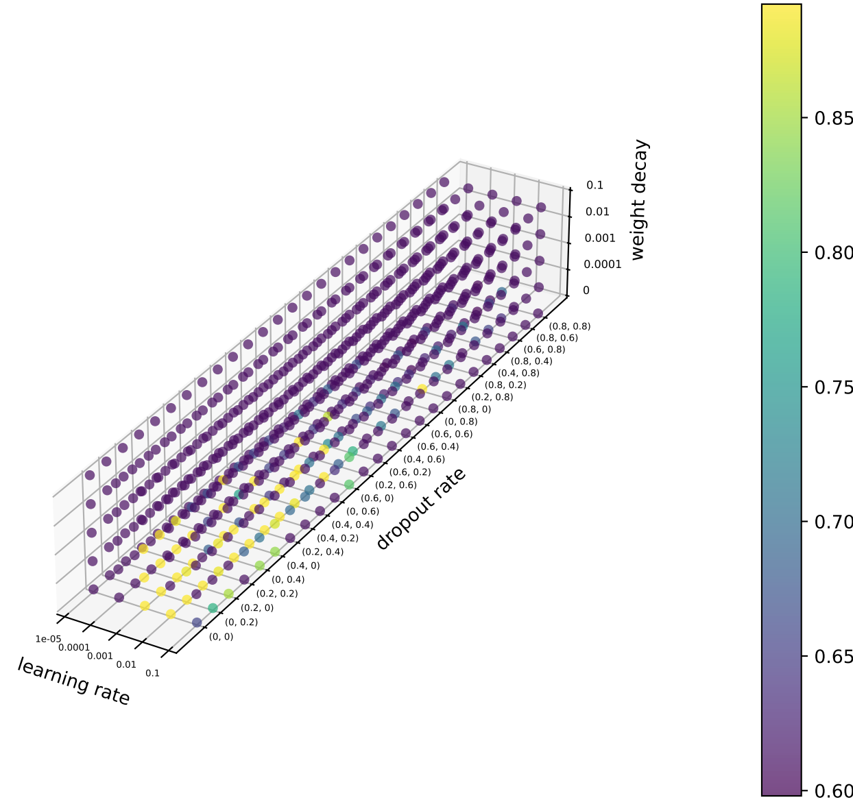
Accuracy
