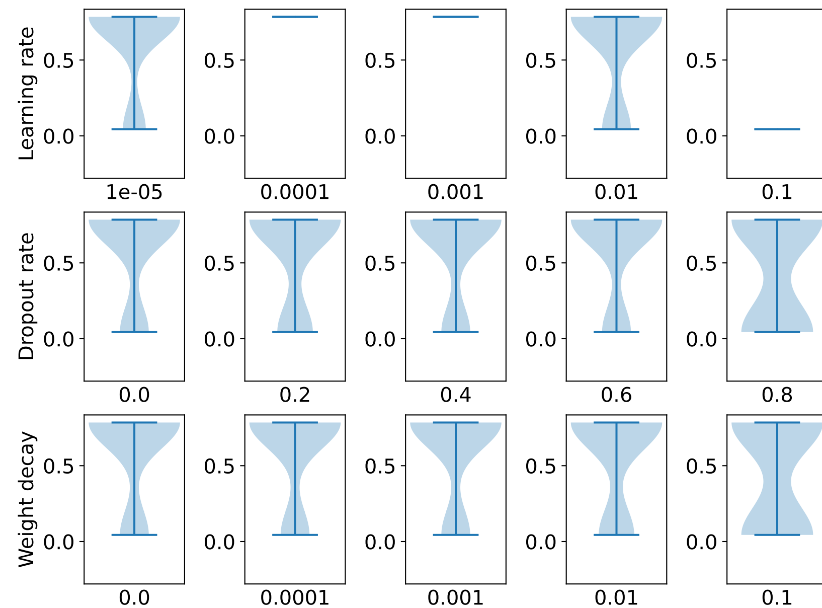
LightDeepGAT2MLP
