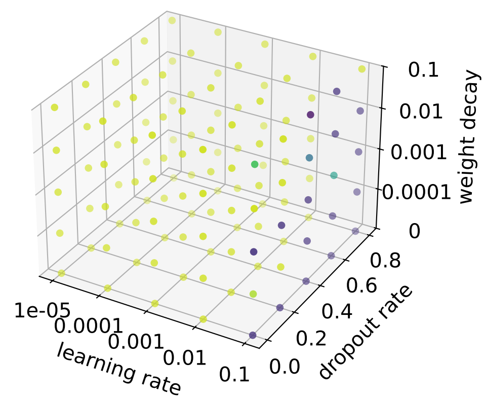
ChebNet2MLP
