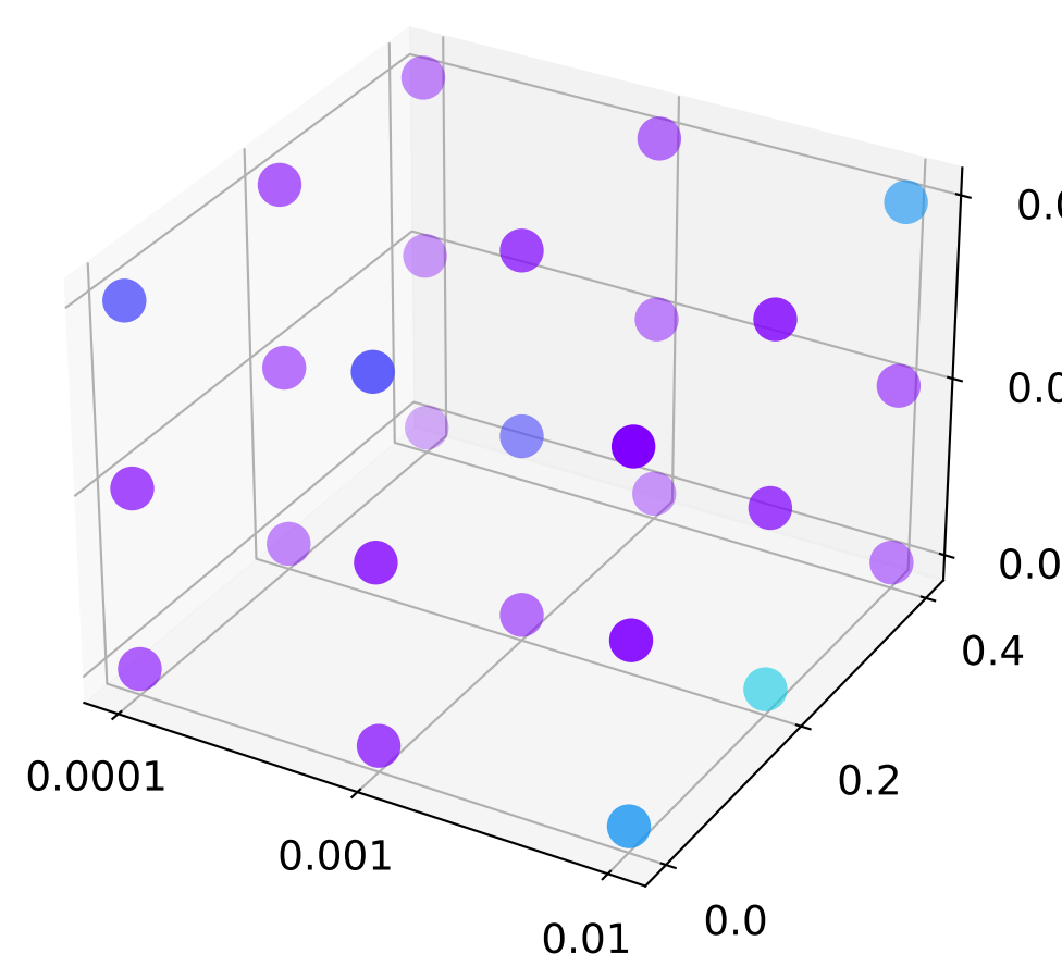
xResGAT2MLP
