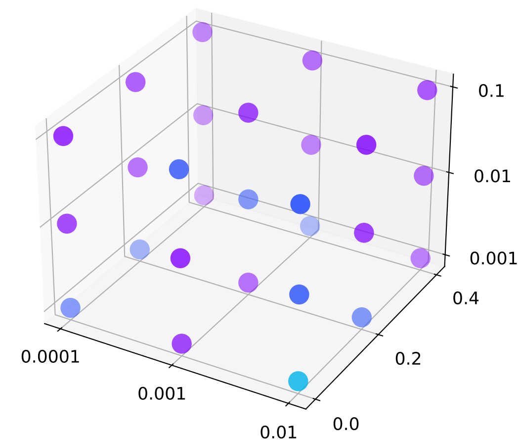
GCN2MLP
