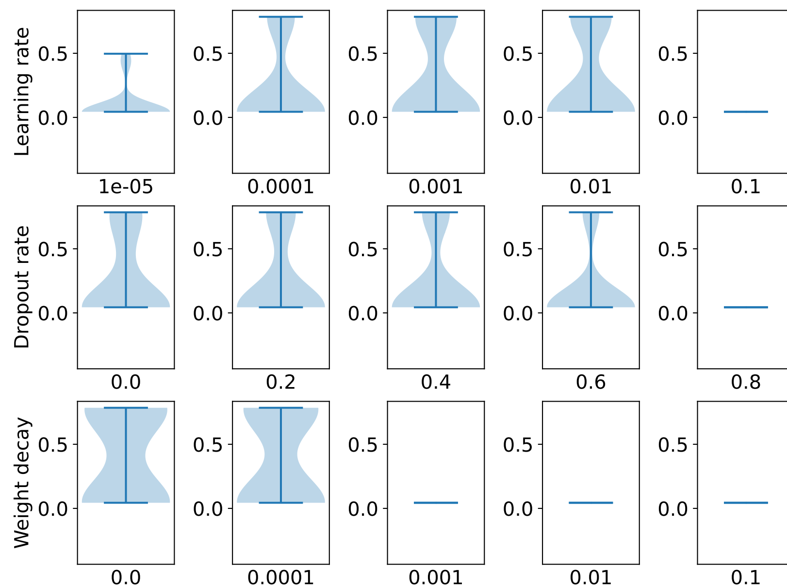
DeepGAT
