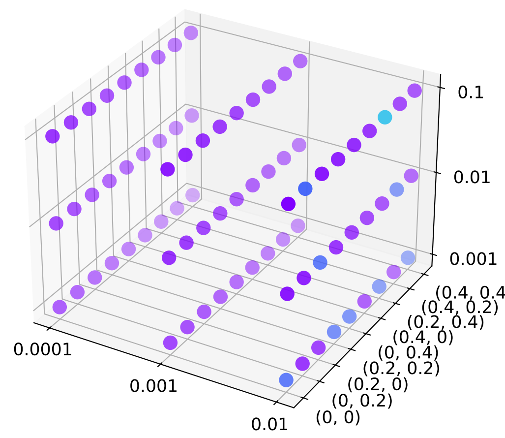
GAT2MLP
