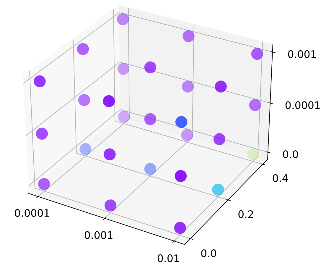
ChebNet2MLP
