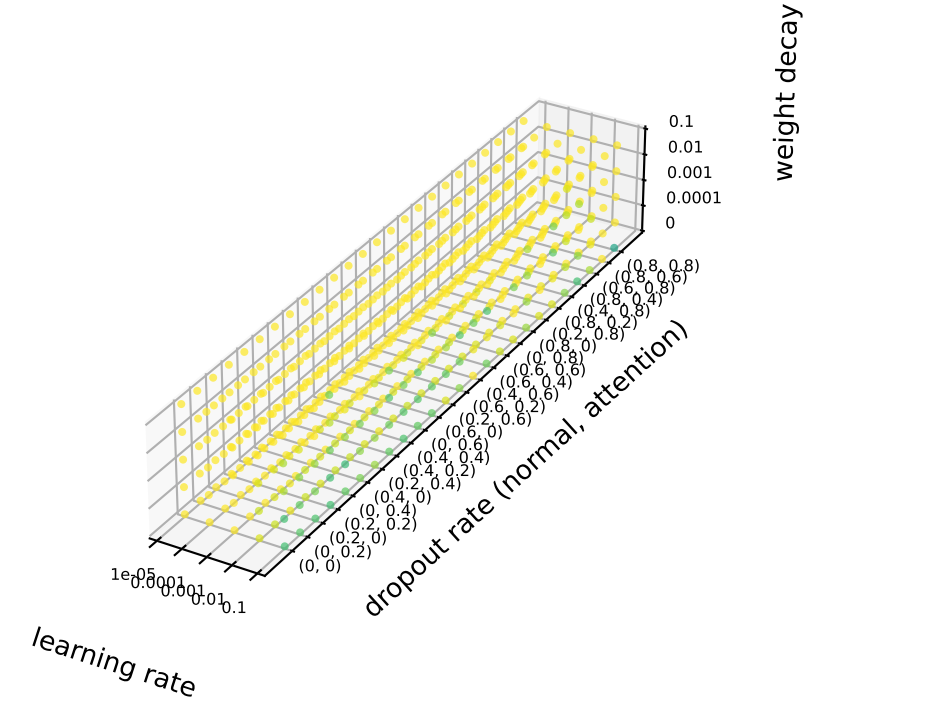
mDenseGAT2MLP
