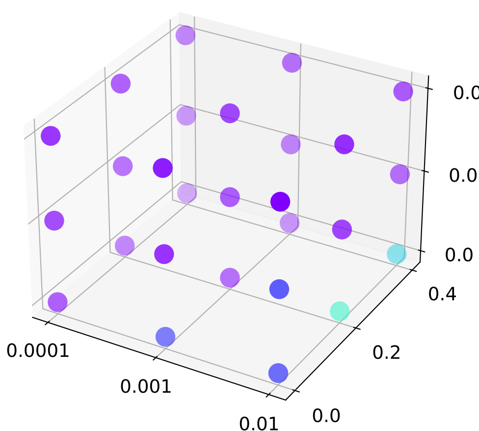
xDenseGCN2MLP
