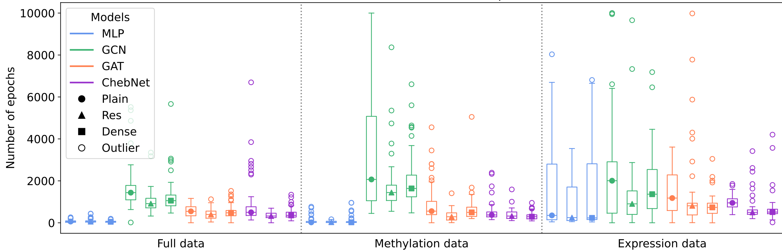
Test results over all outer splits
