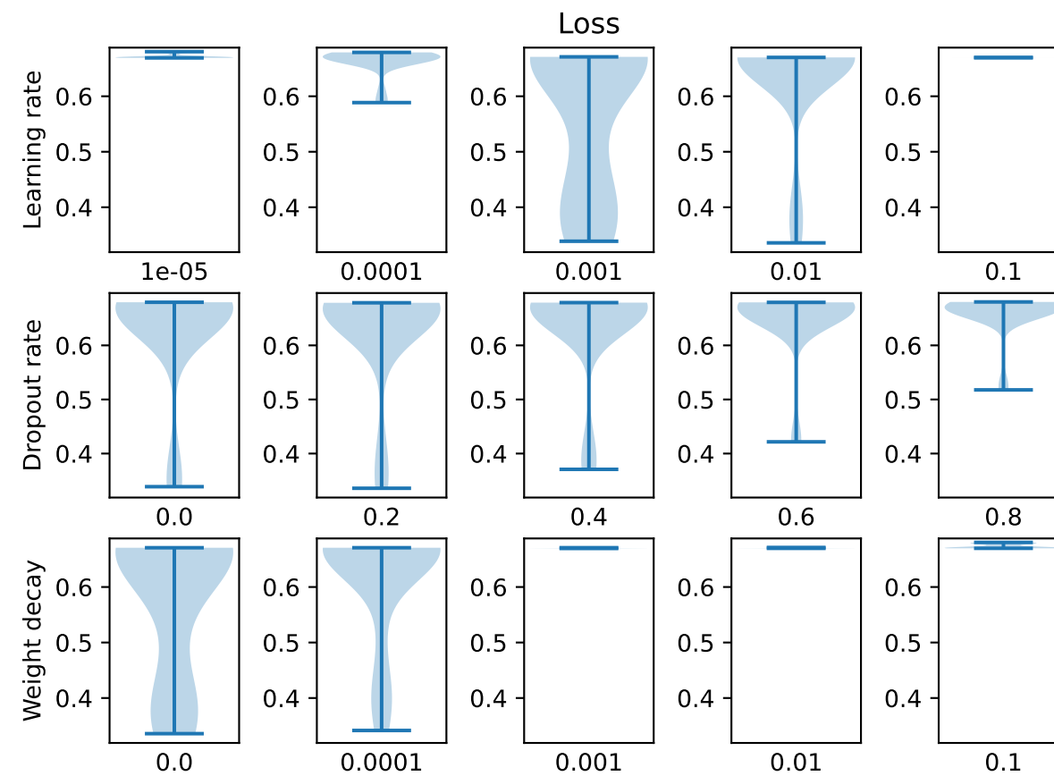
GCN (batch size 64)
