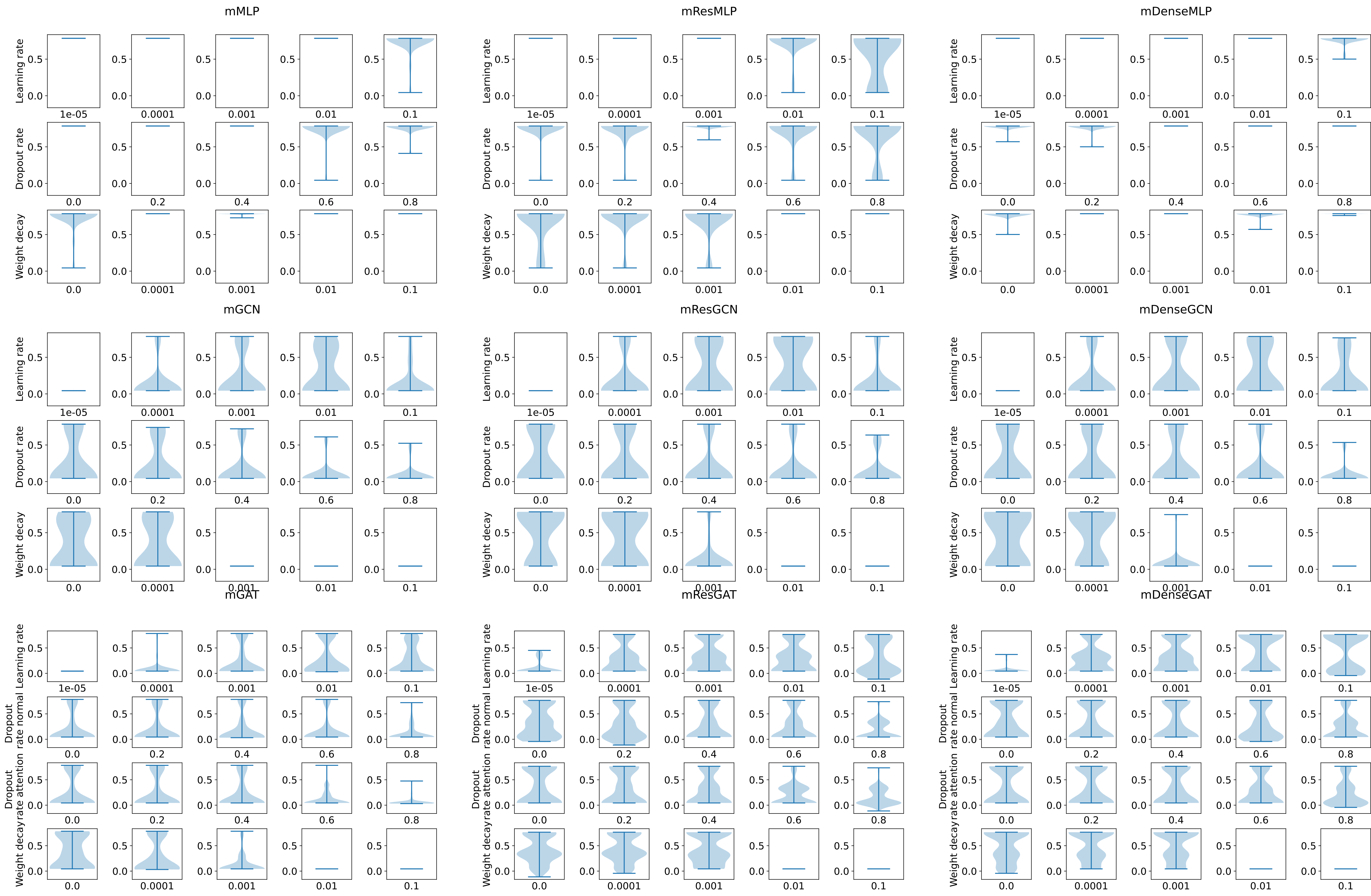
Testrun hyperparameter MCC results for methylation data
