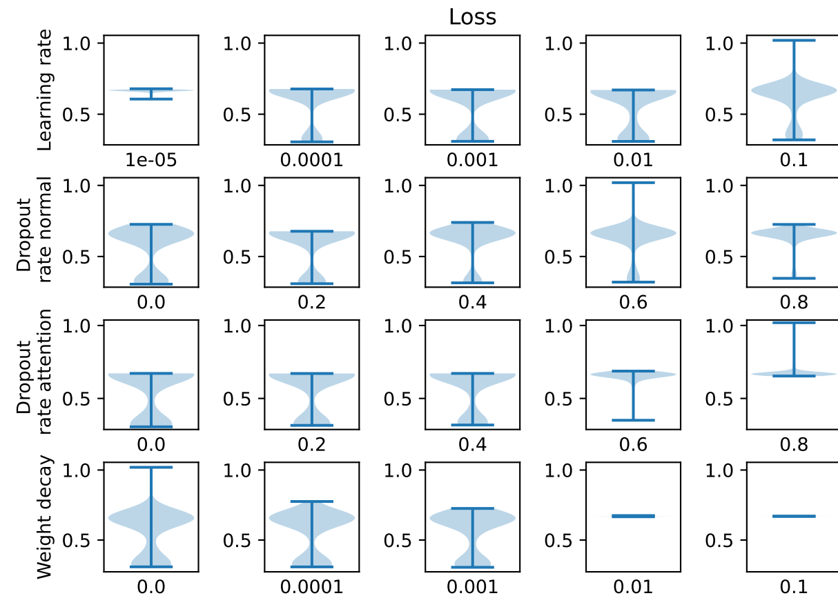
ResGAT (full batch)
