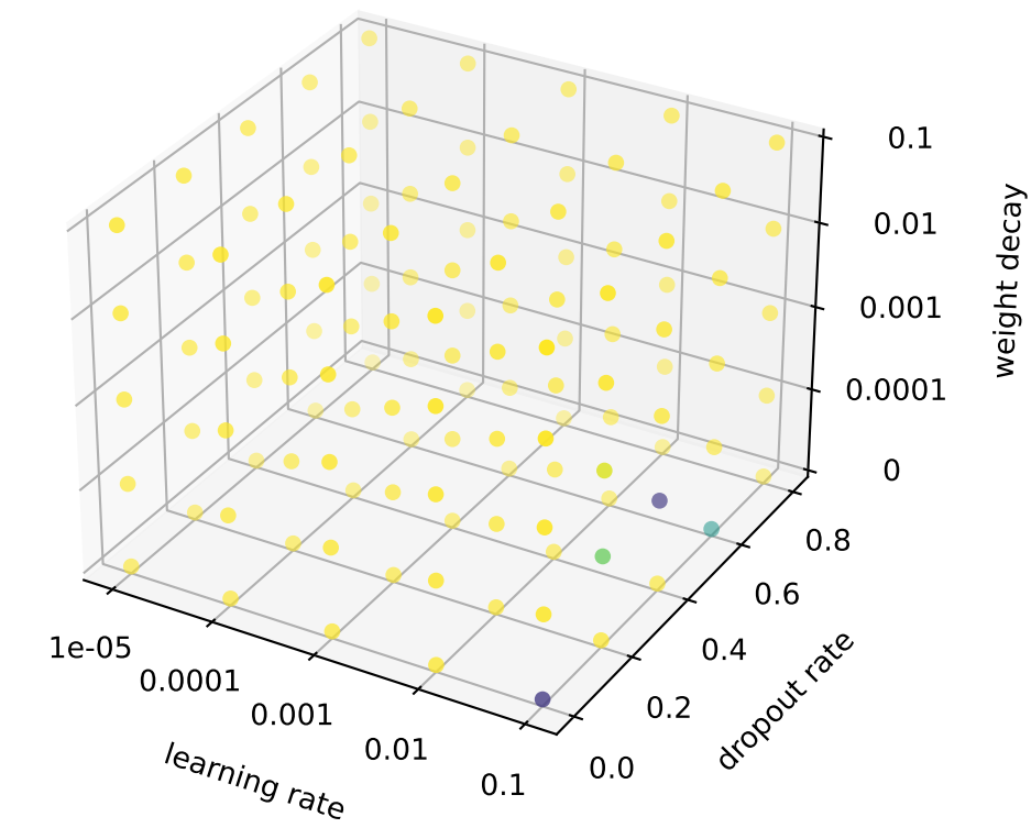
mDenseGAT2MLP
