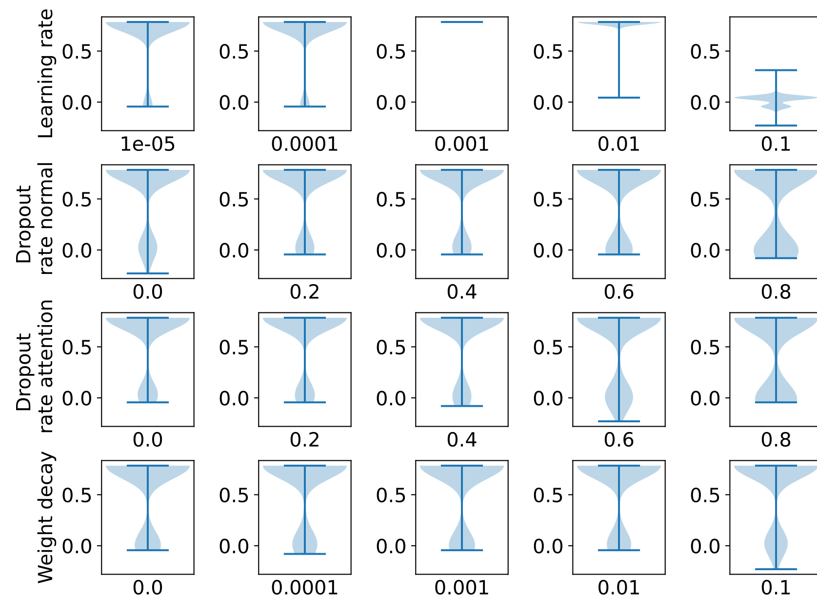
LightDeepGAT2MLP
