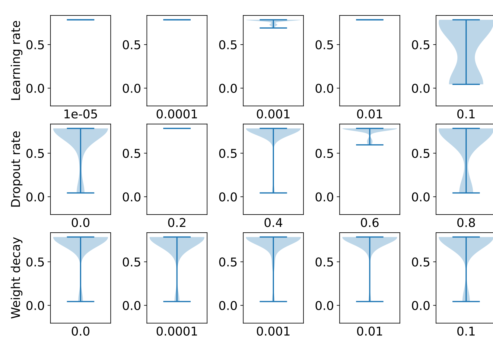
CoarseningChebNet2MLP
