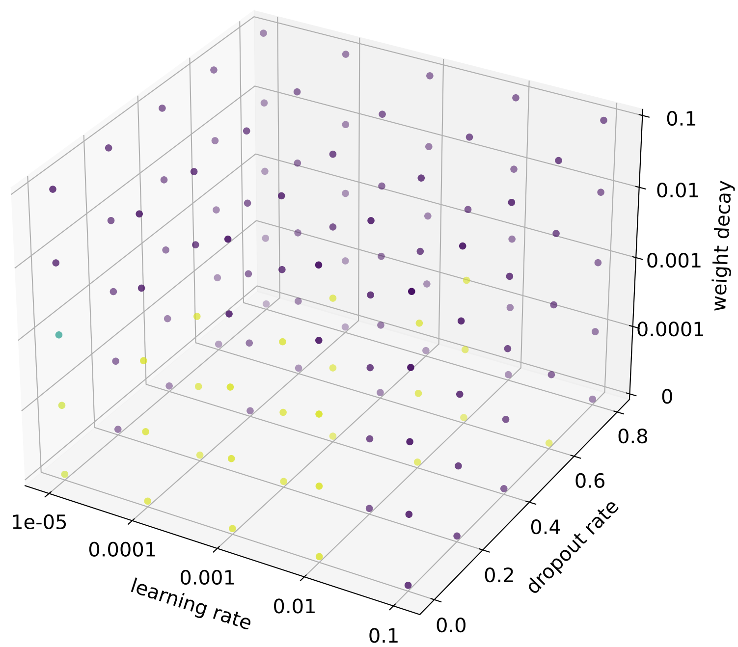
DeepChebNet
