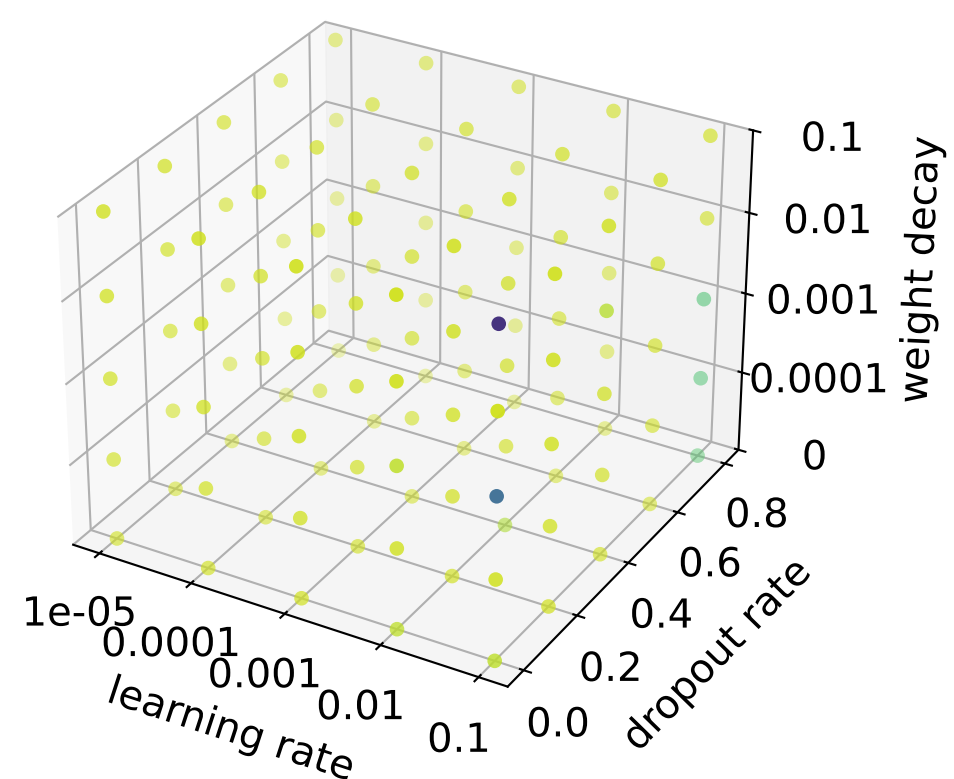
mResChebNet2MLP
