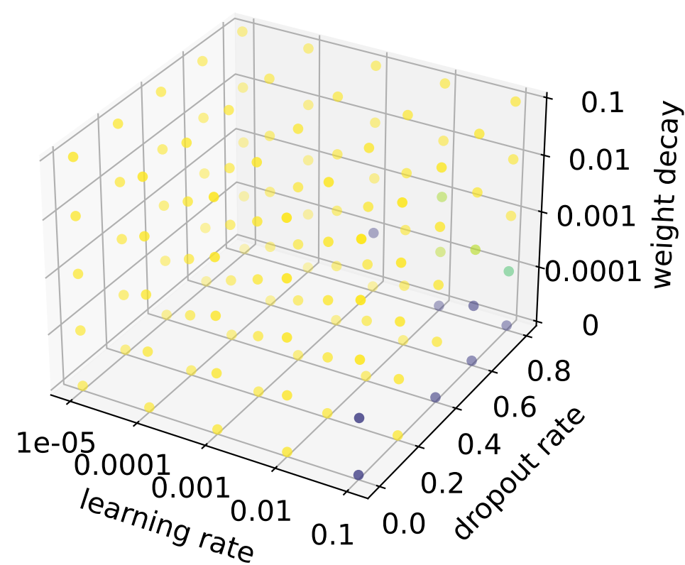
DenseMLP
