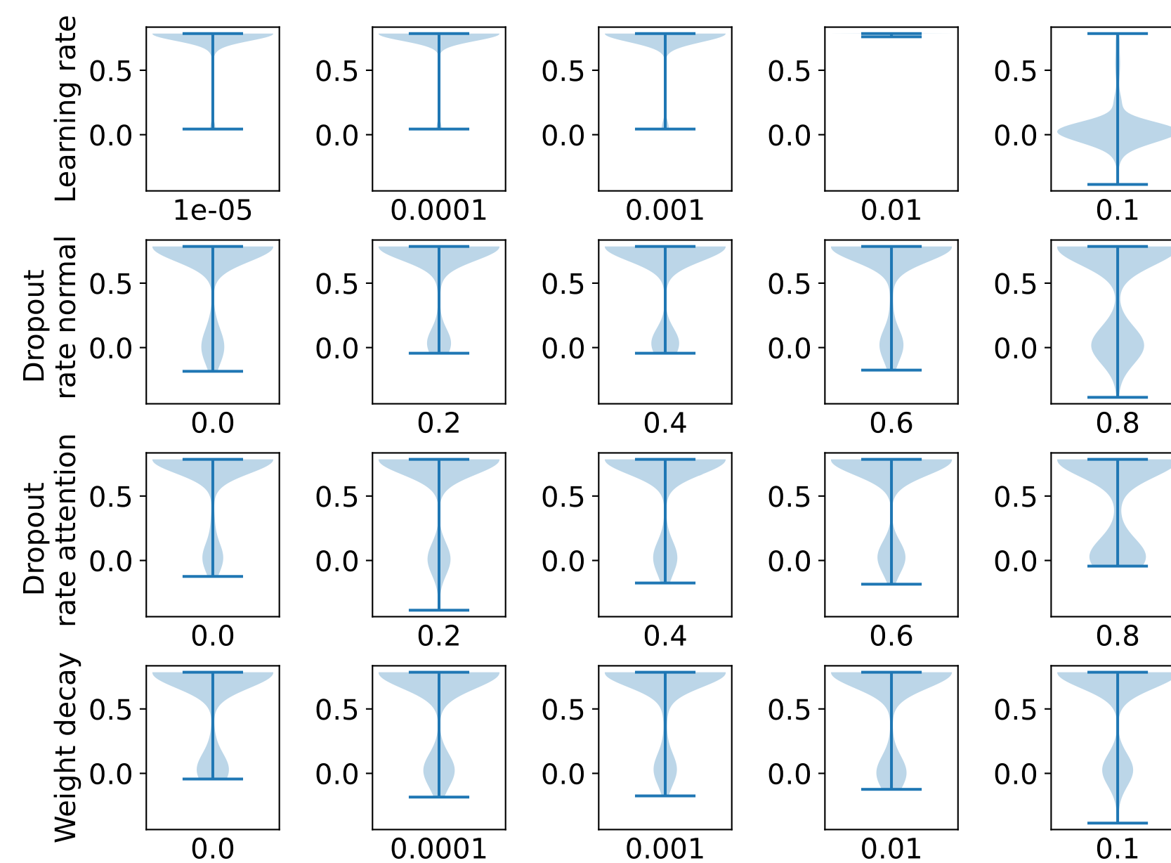
DeepGAT2MLP
