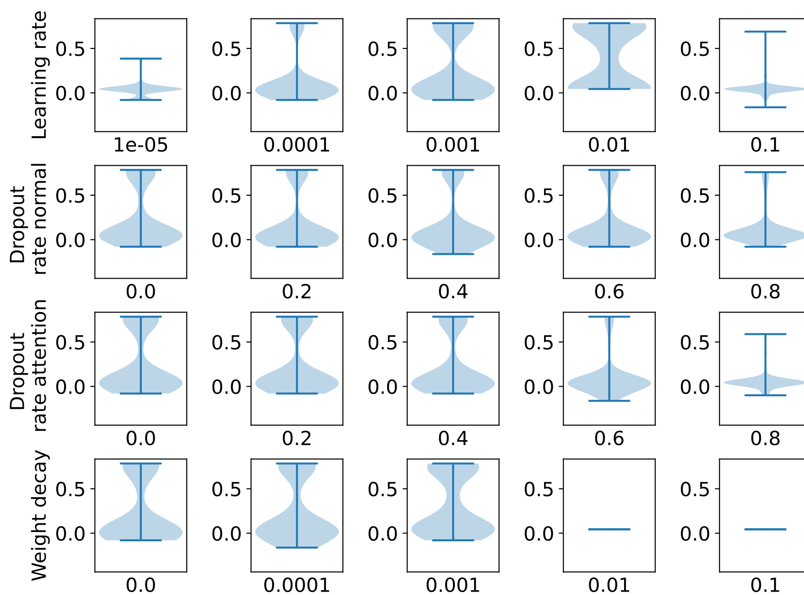
DeepGAT
