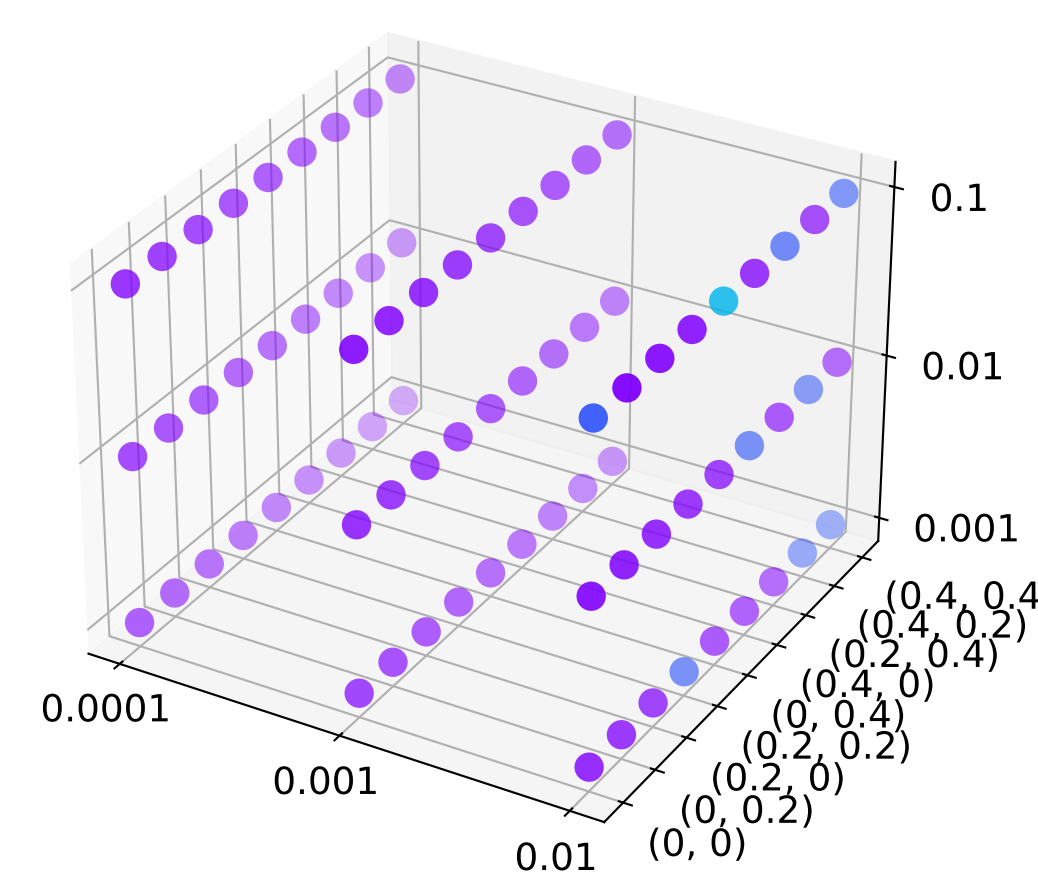
mChebNet2MLP
