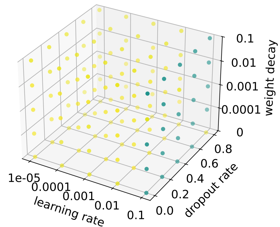
xDenseGCN2MLP
