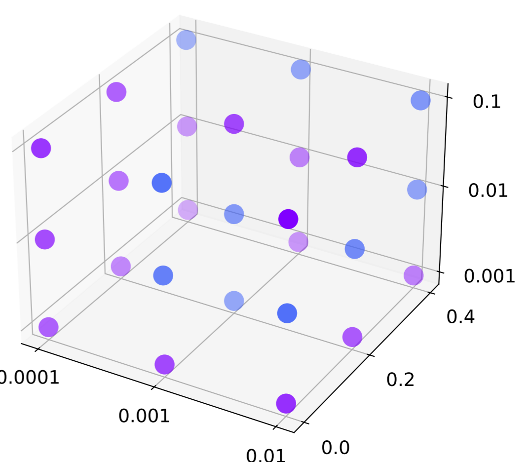
DenseChebNet2MLP
