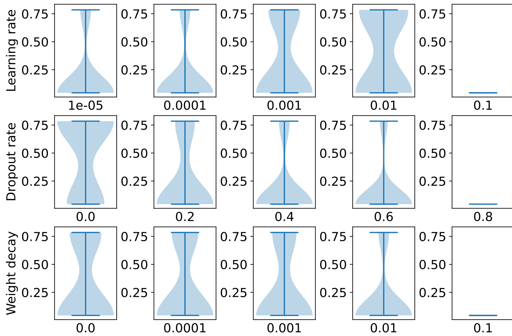
LightDeepChebNet
