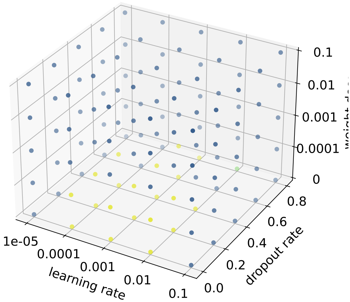
LightDeepGCN
