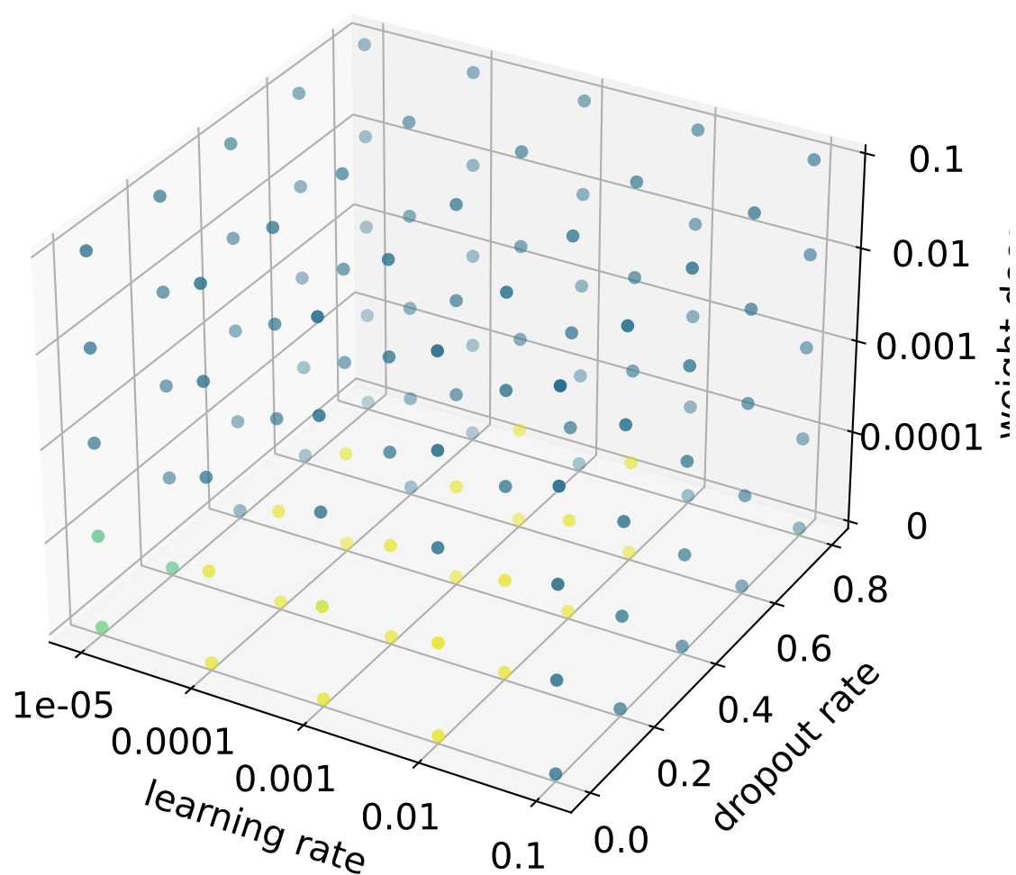
DeepGCN
