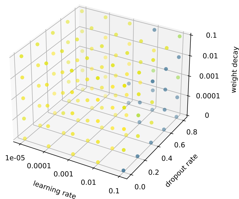
xDenseMLP
