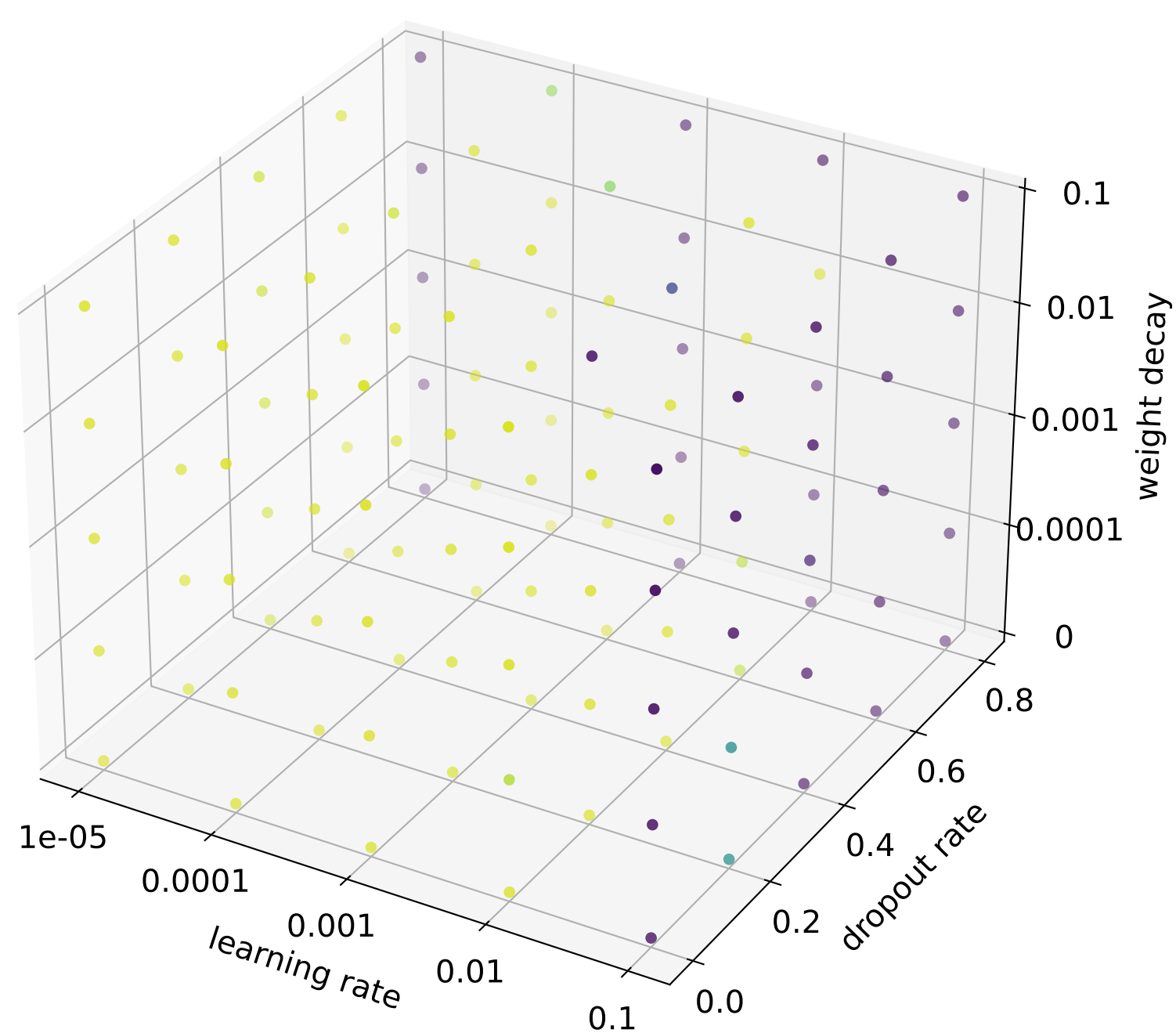
LightDeepChebNet2MLP
