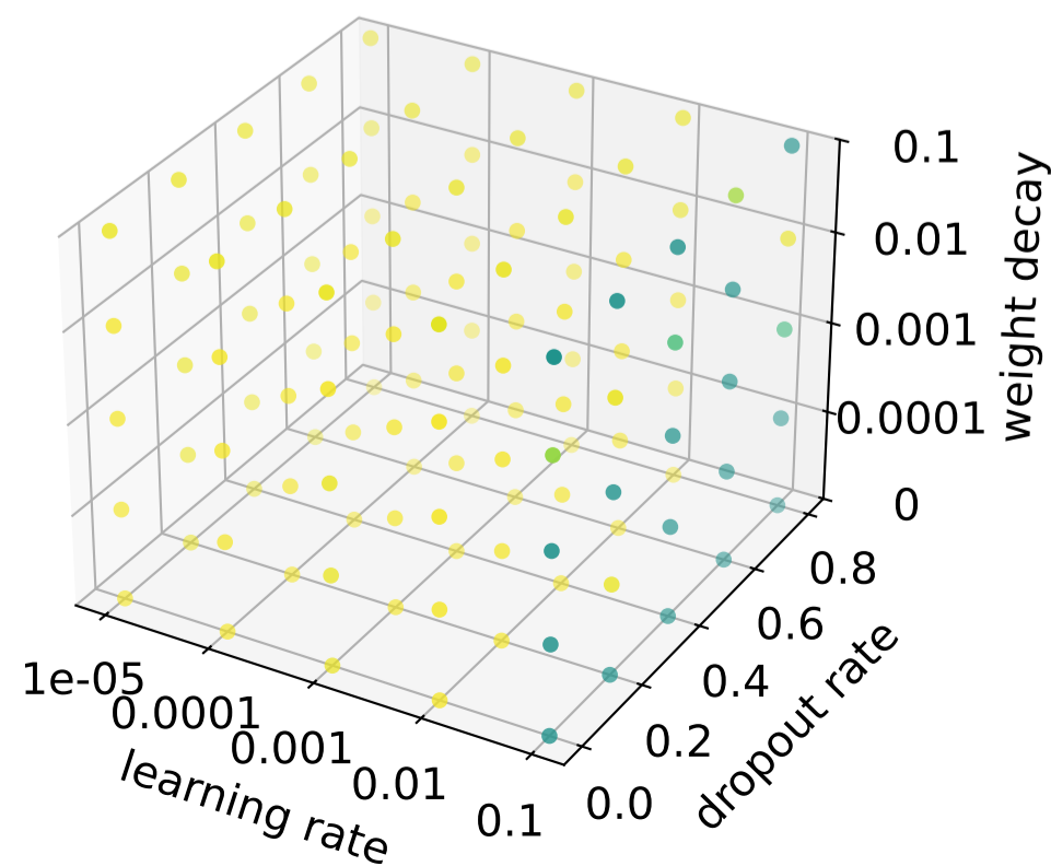
xResGCN2MLP
