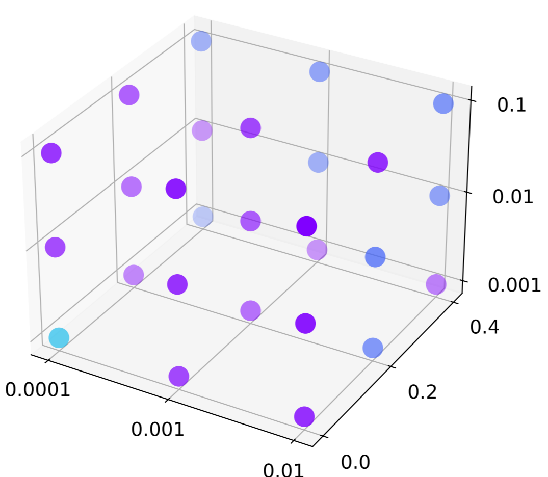
ResChebNet2MLP
