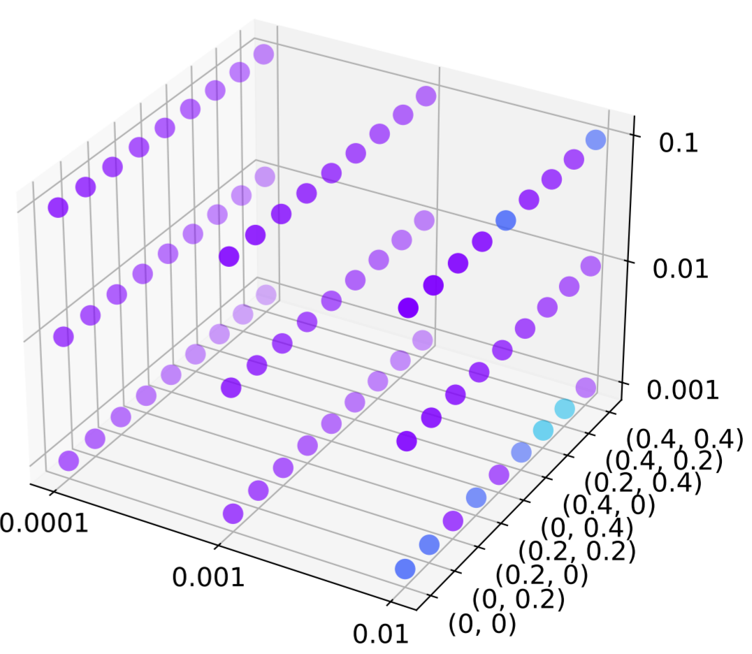
DenseGAT2MLP
