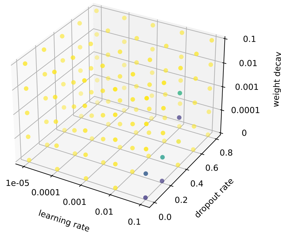
mResGAT2MLP
