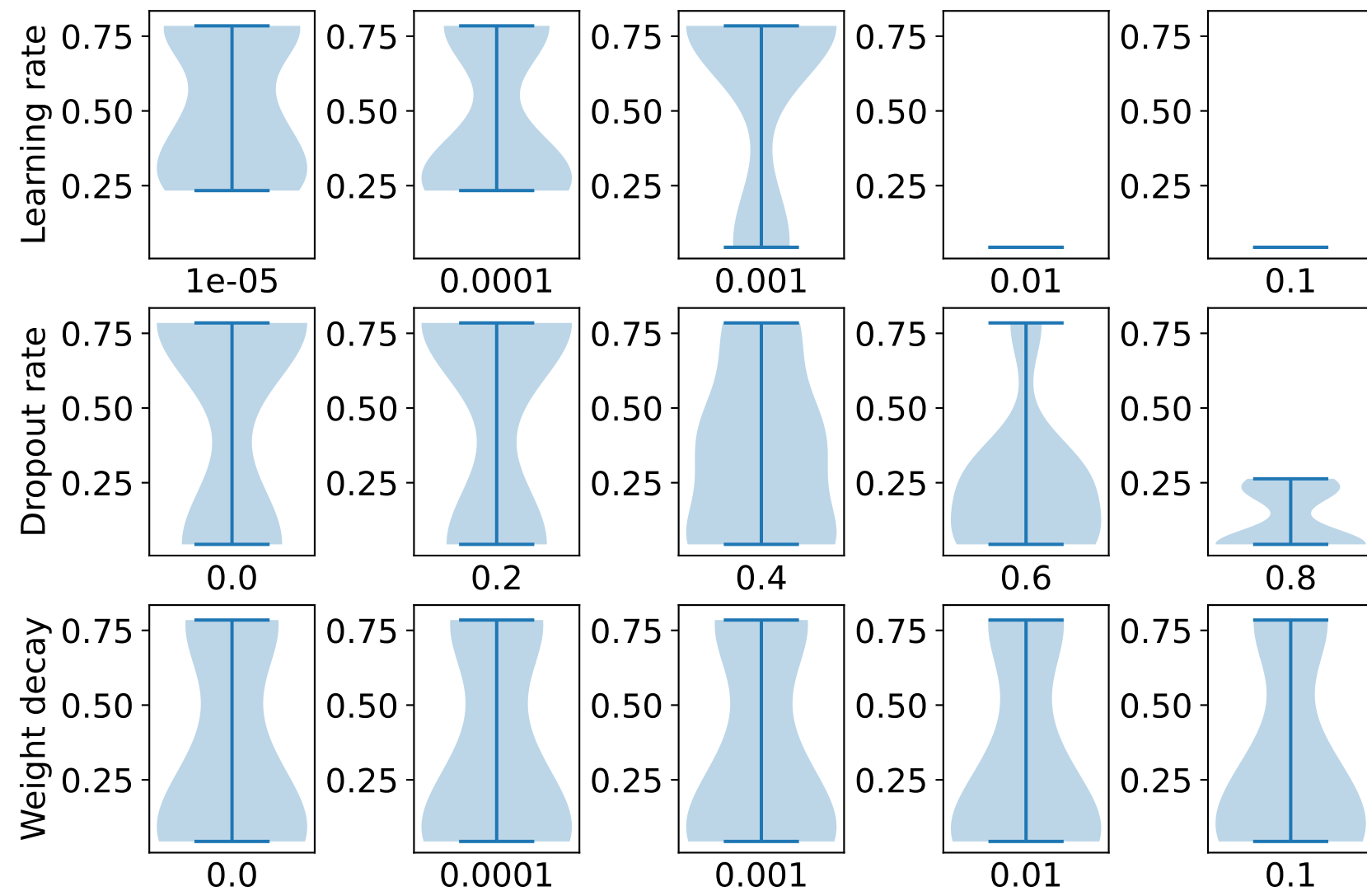
LightDeepChebNet2MLP
