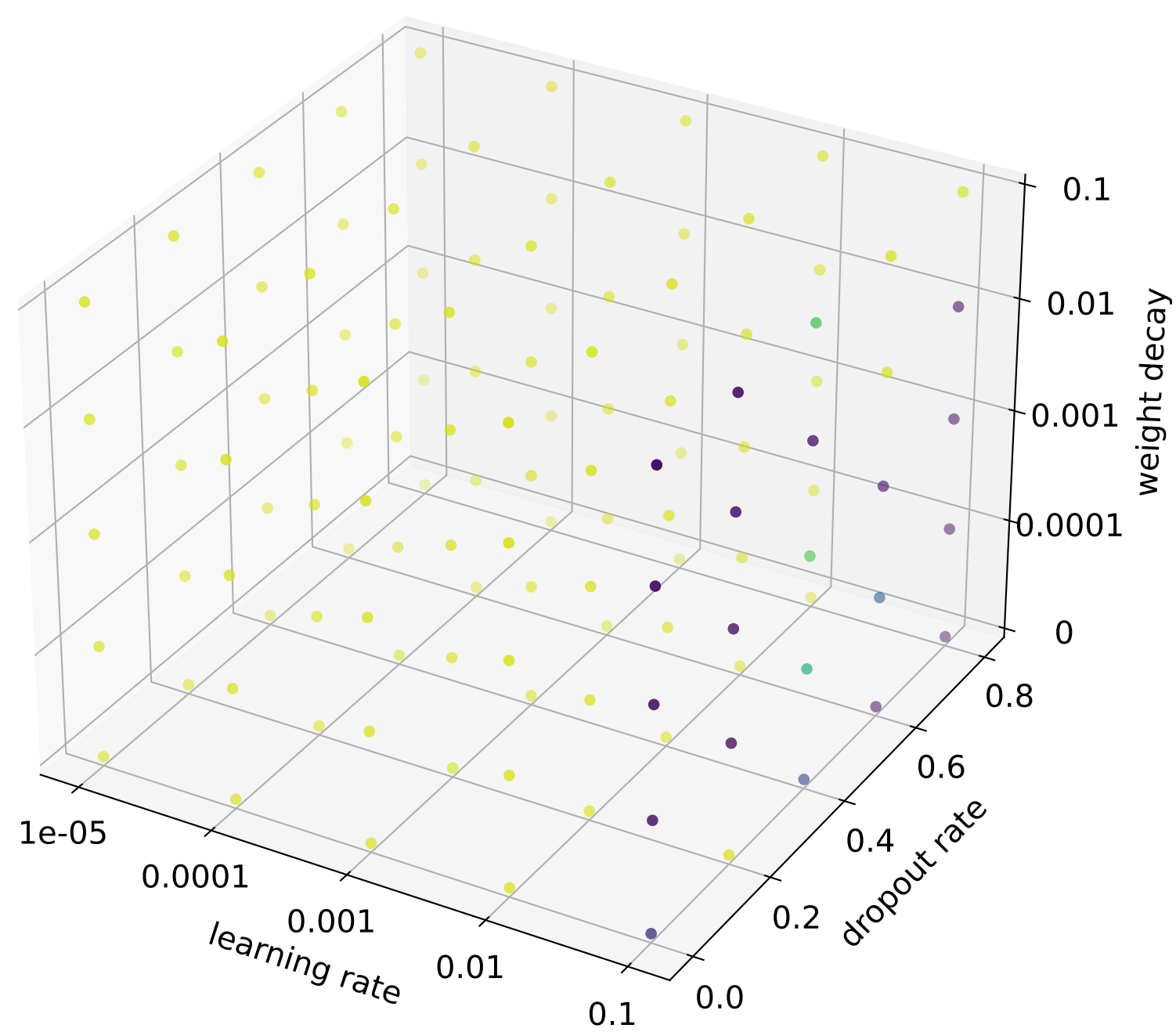
DeepChebNet2MLP
