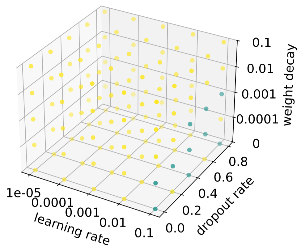
ResGCN2MLP
