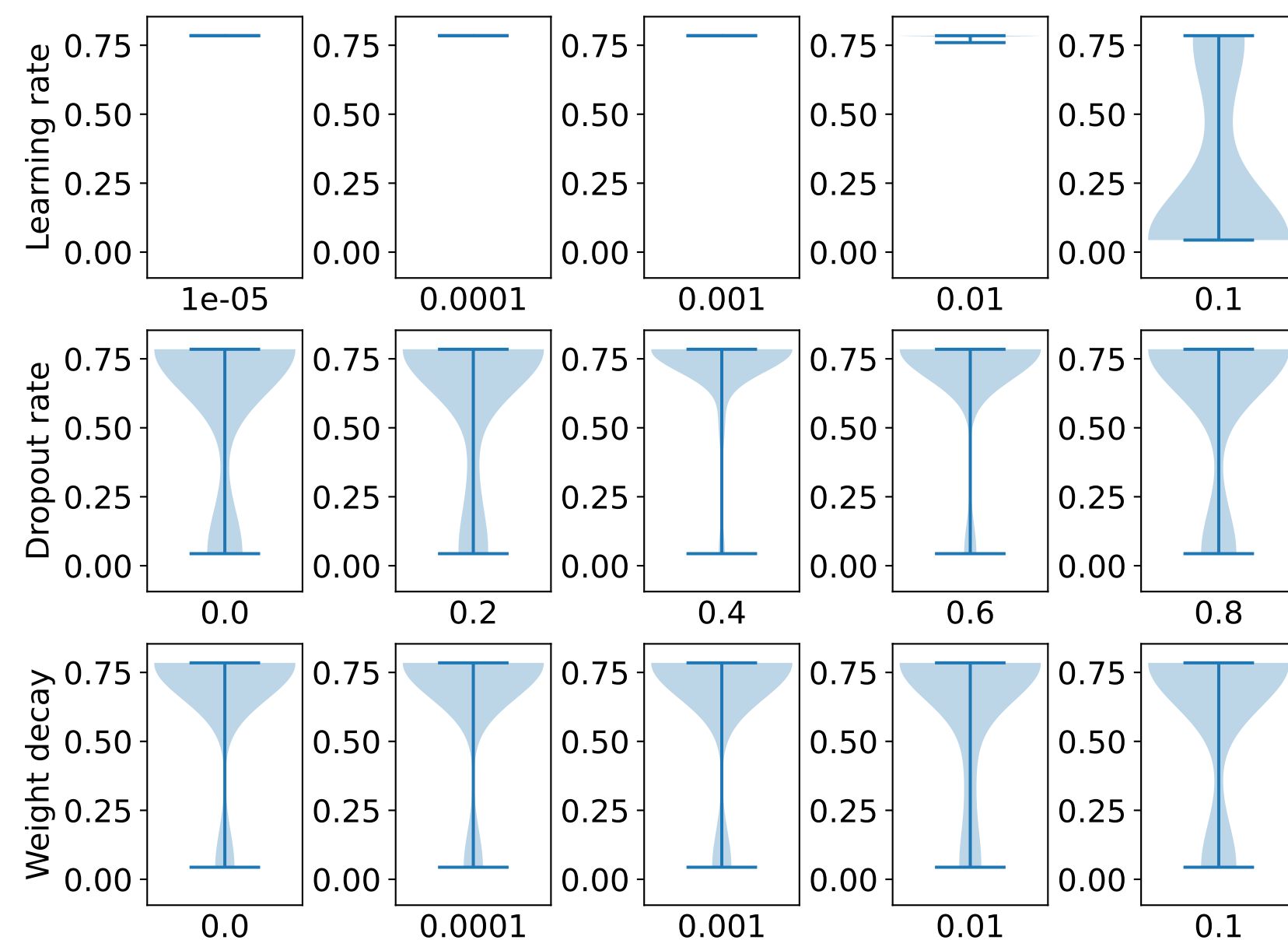
LightGAT2MLP
