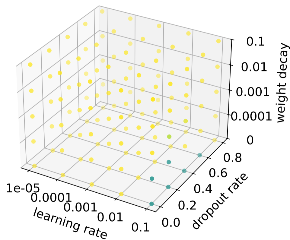
mResGCN2MLP
