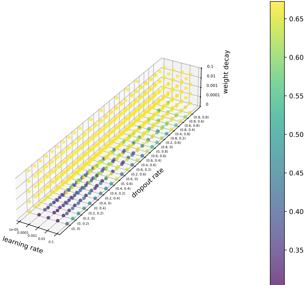
Loss
