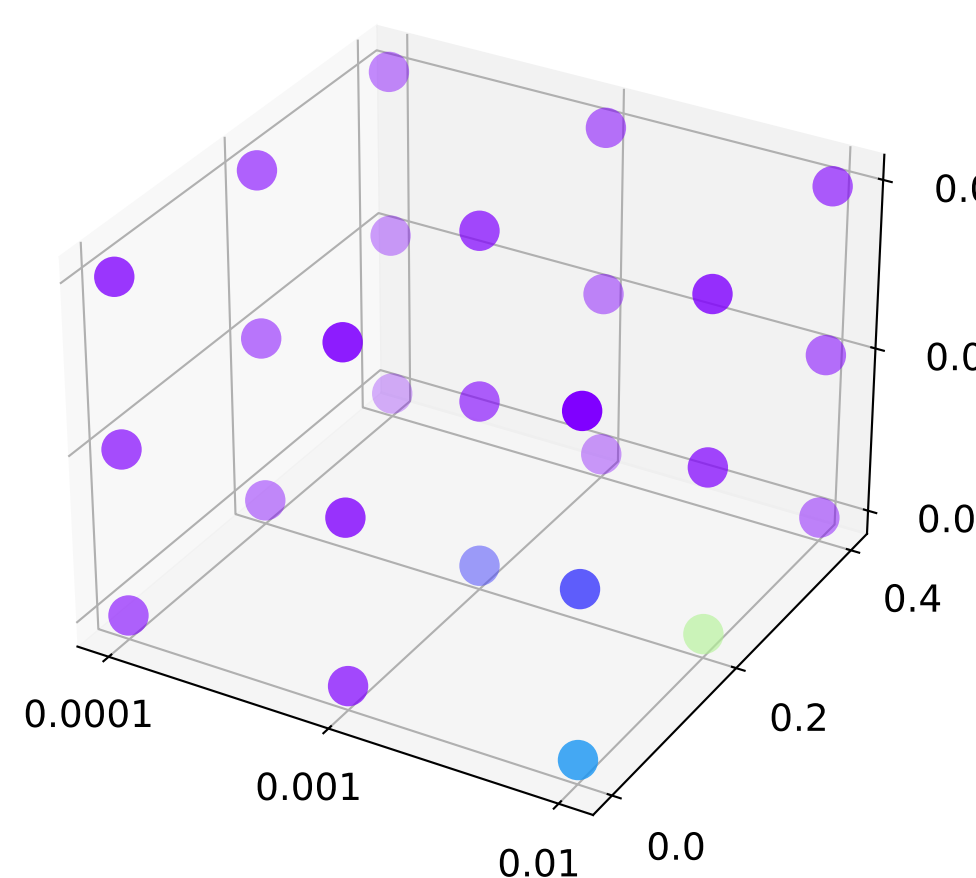
xResGCN2MLP
