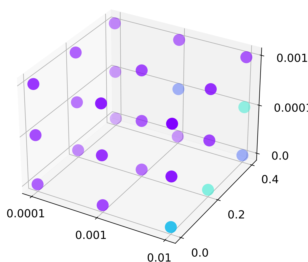
mResGCN2MLP
