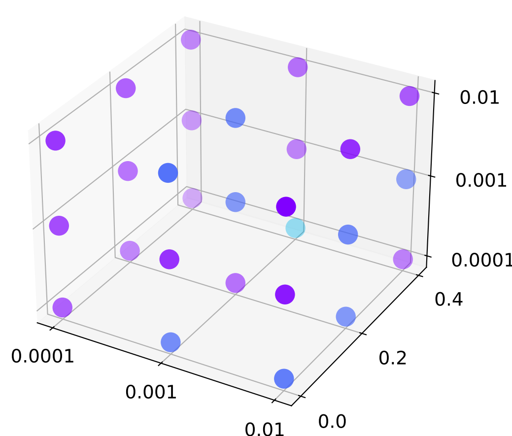
mResChebNet2MLP
