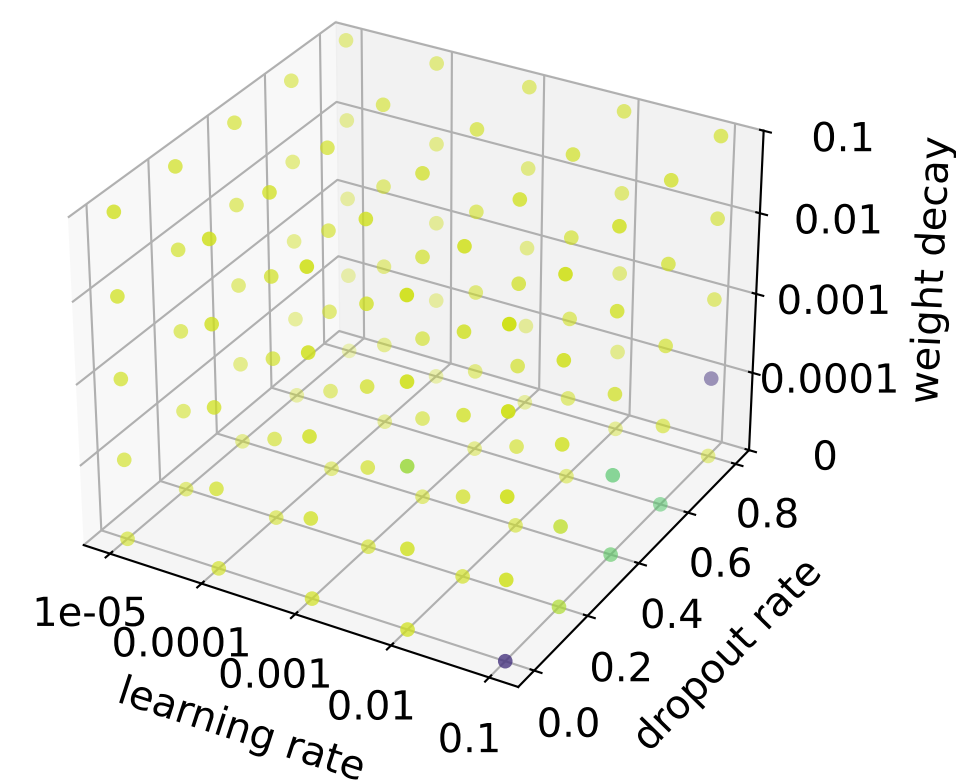
DenseChebNet2MLP
