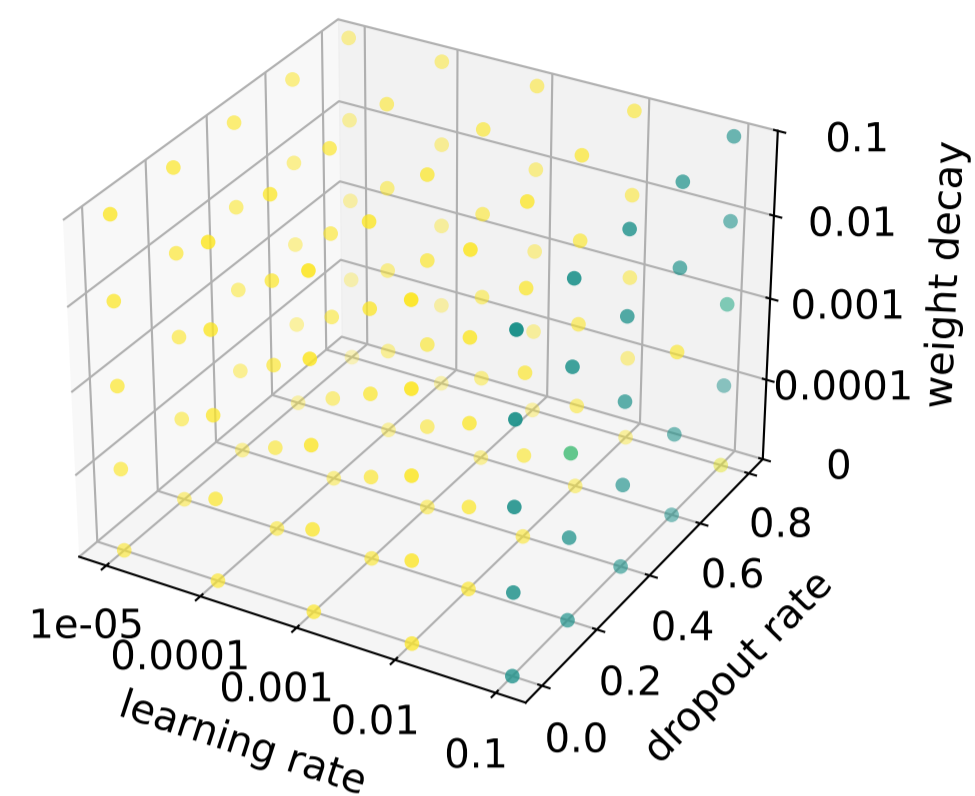
GCN2MLP
