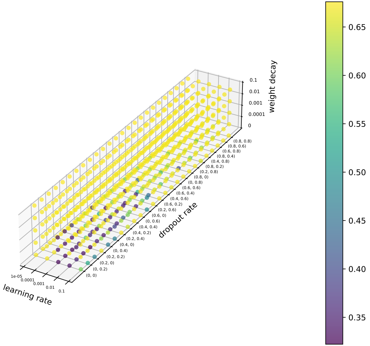
Loss
