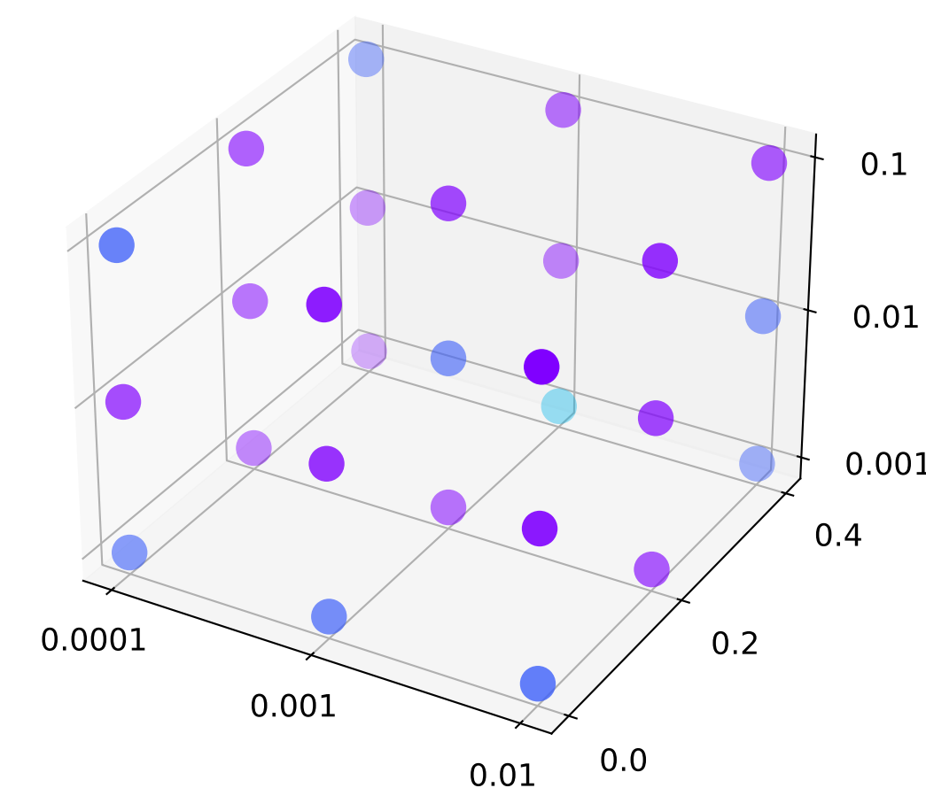
ChebNet2MLP
