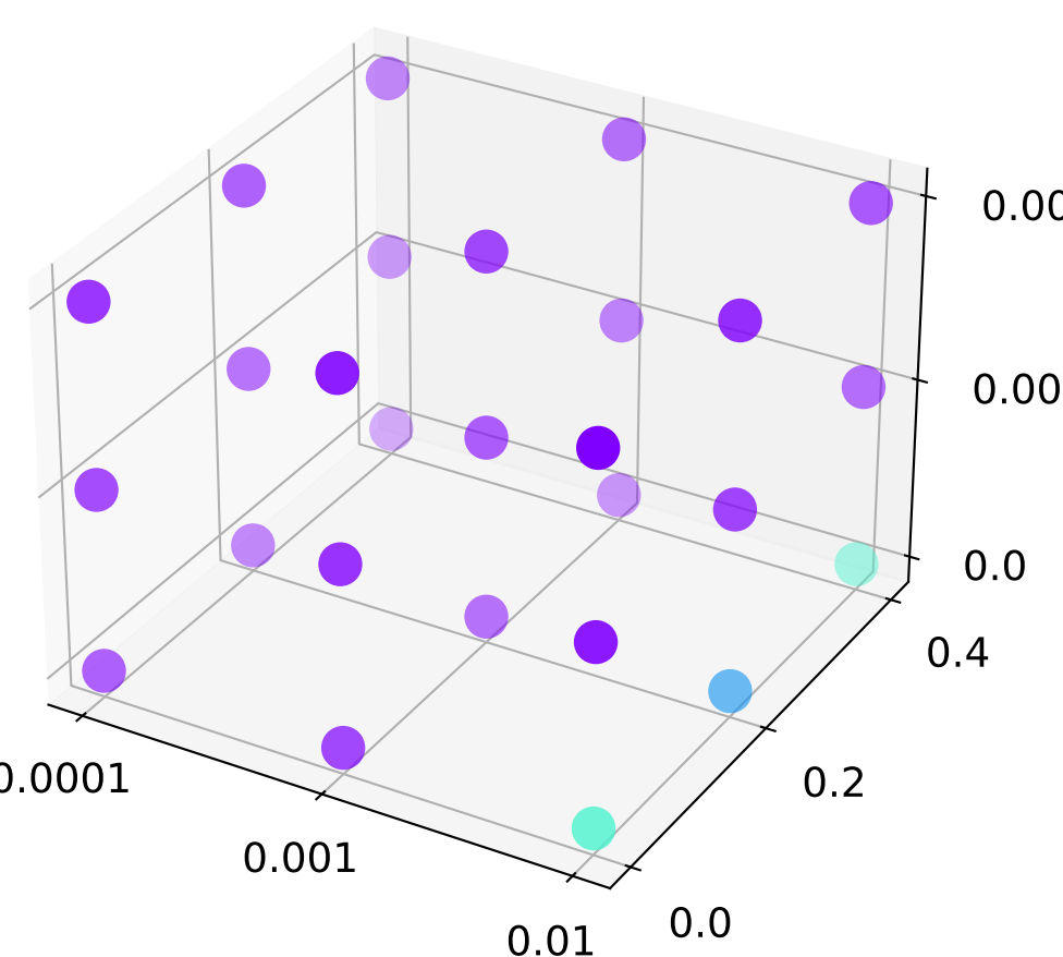
xGCN2MLP
