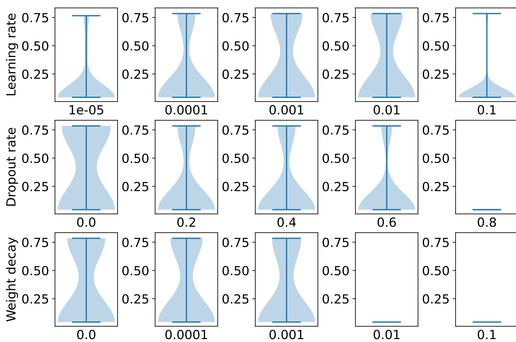
DeepChebNet
