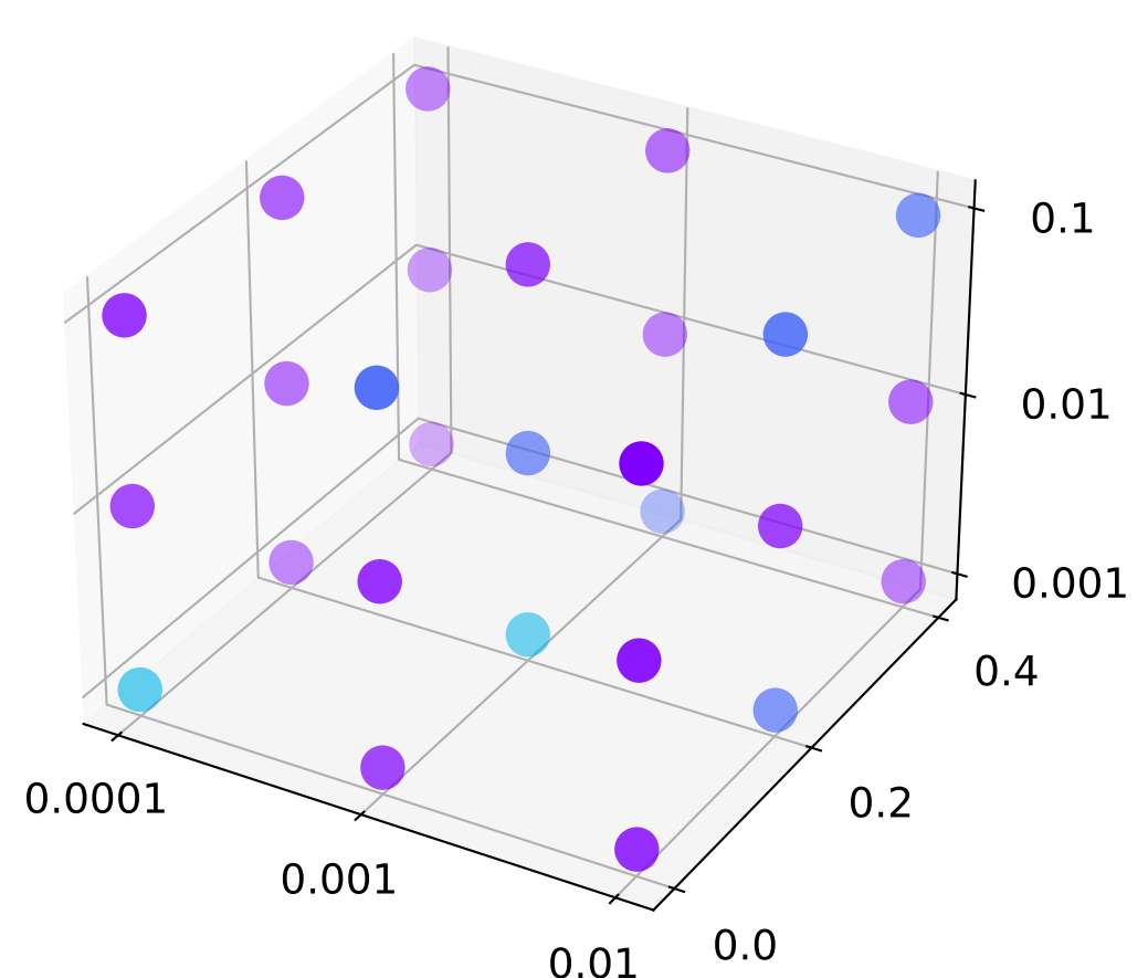
mResGAT2MLP
