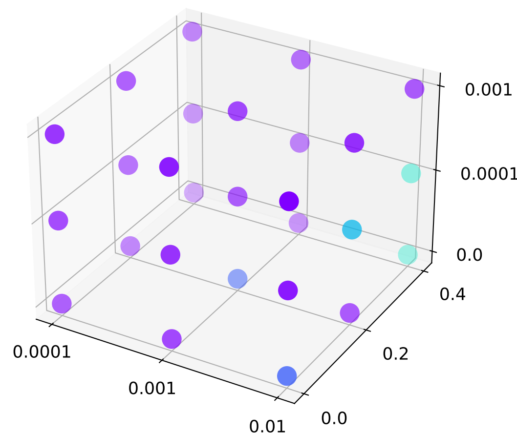
GAT2MLP
