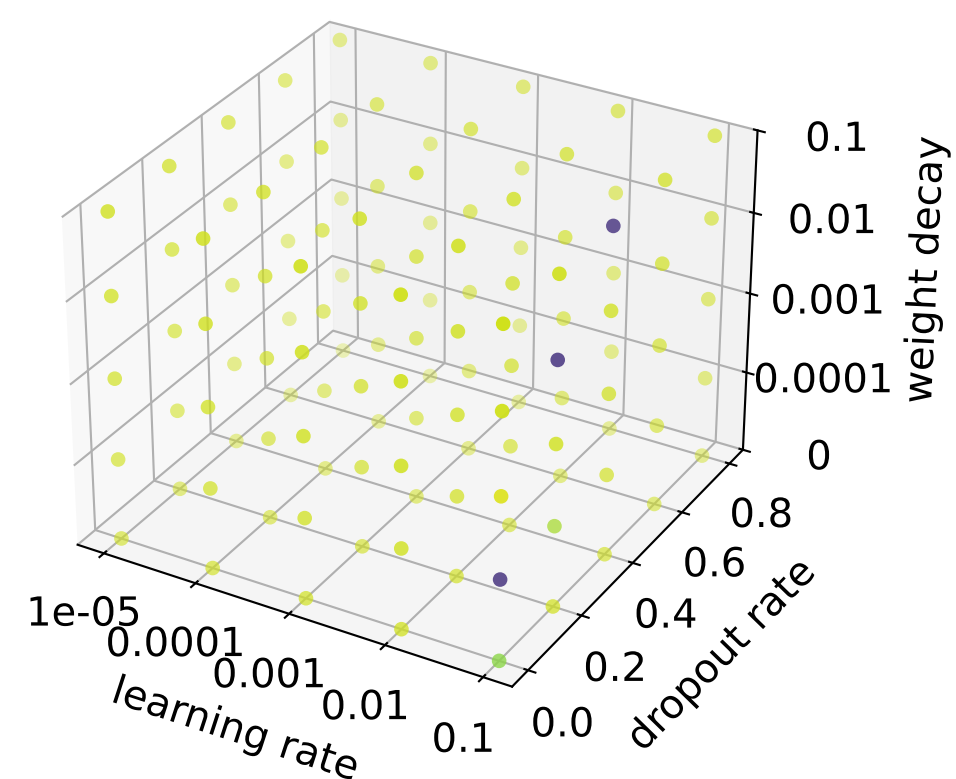
mChebNet2MLP
