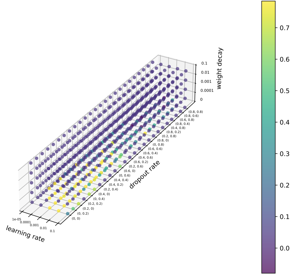
MCC
