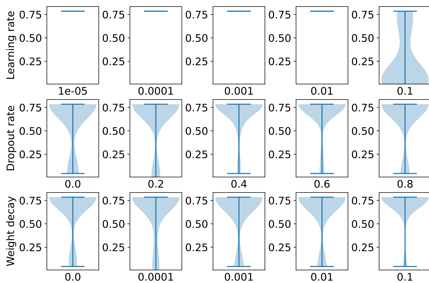
DeepChebNet2MLP
