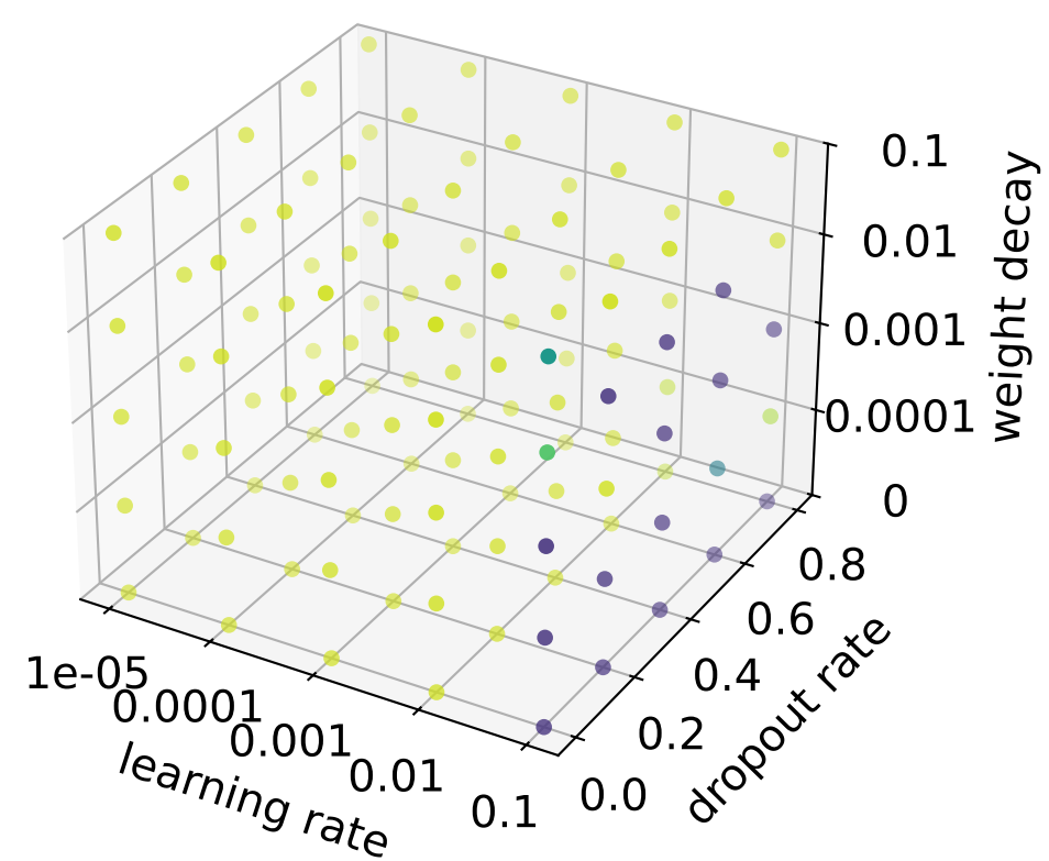
ResChebNet2MLP
