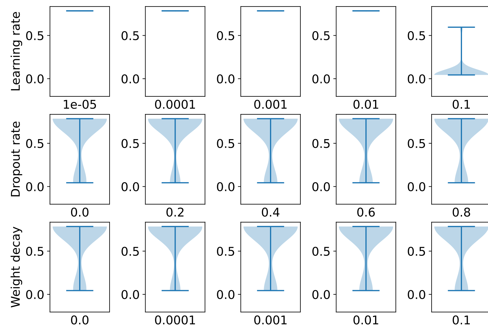
CoarseningChebNet2MLP
