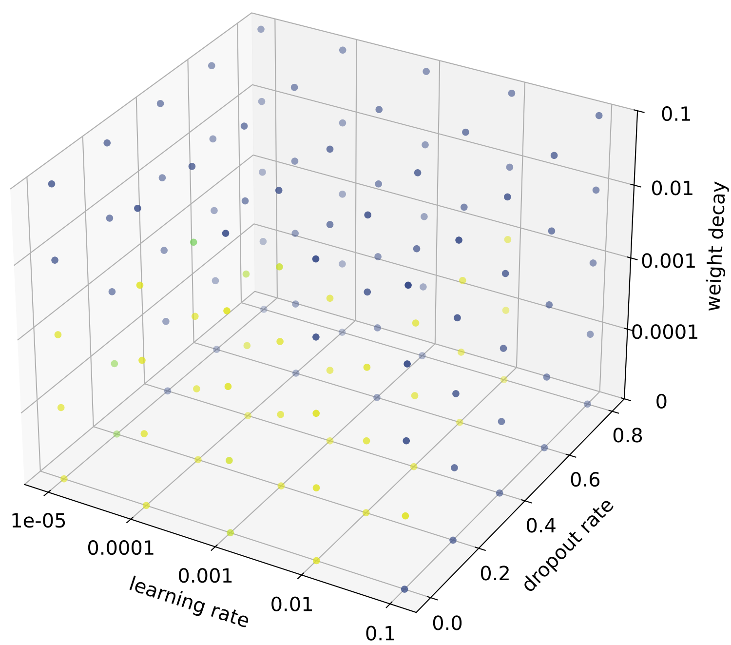
CoarseningGAT2MLP
