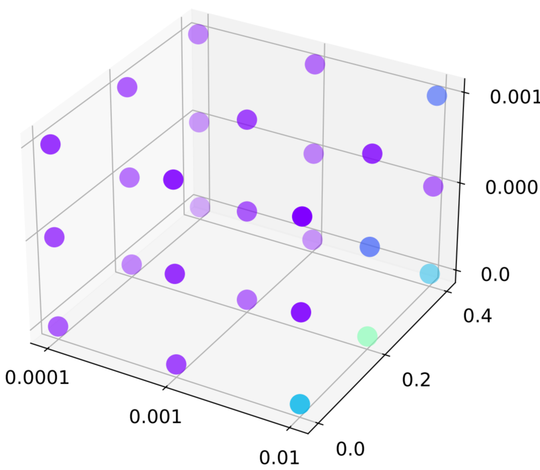
ResChebNet
