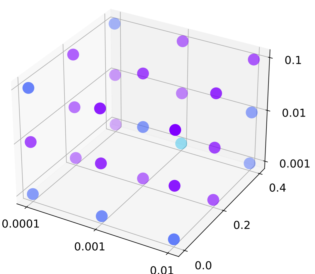
ChebNet2MLP
