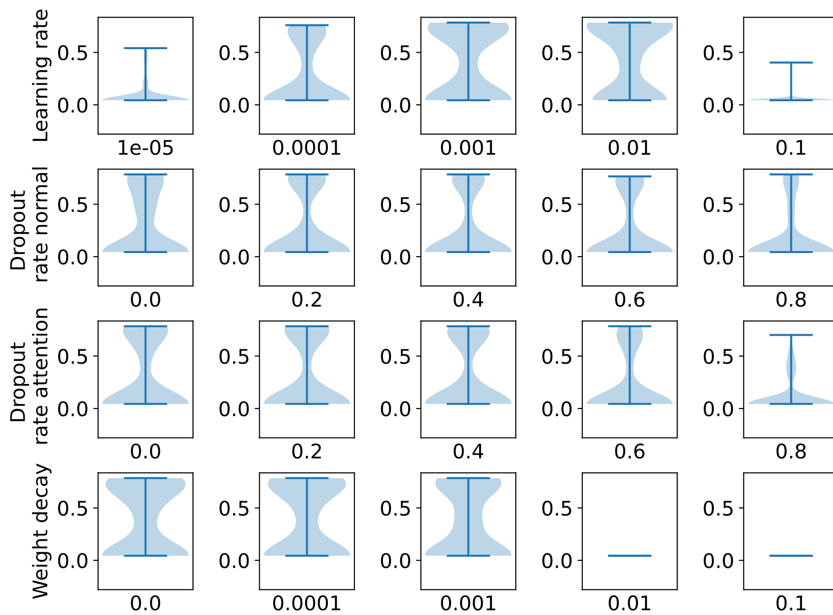
LightDeepGAT
