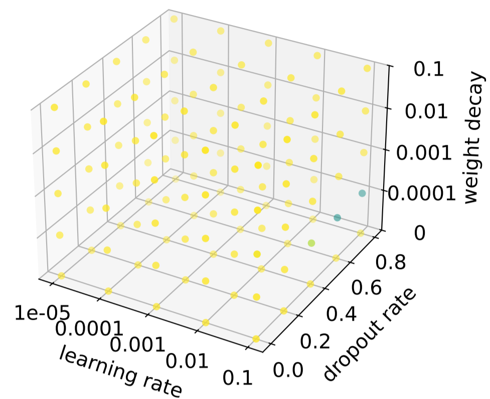
DenseGCN2MLP
