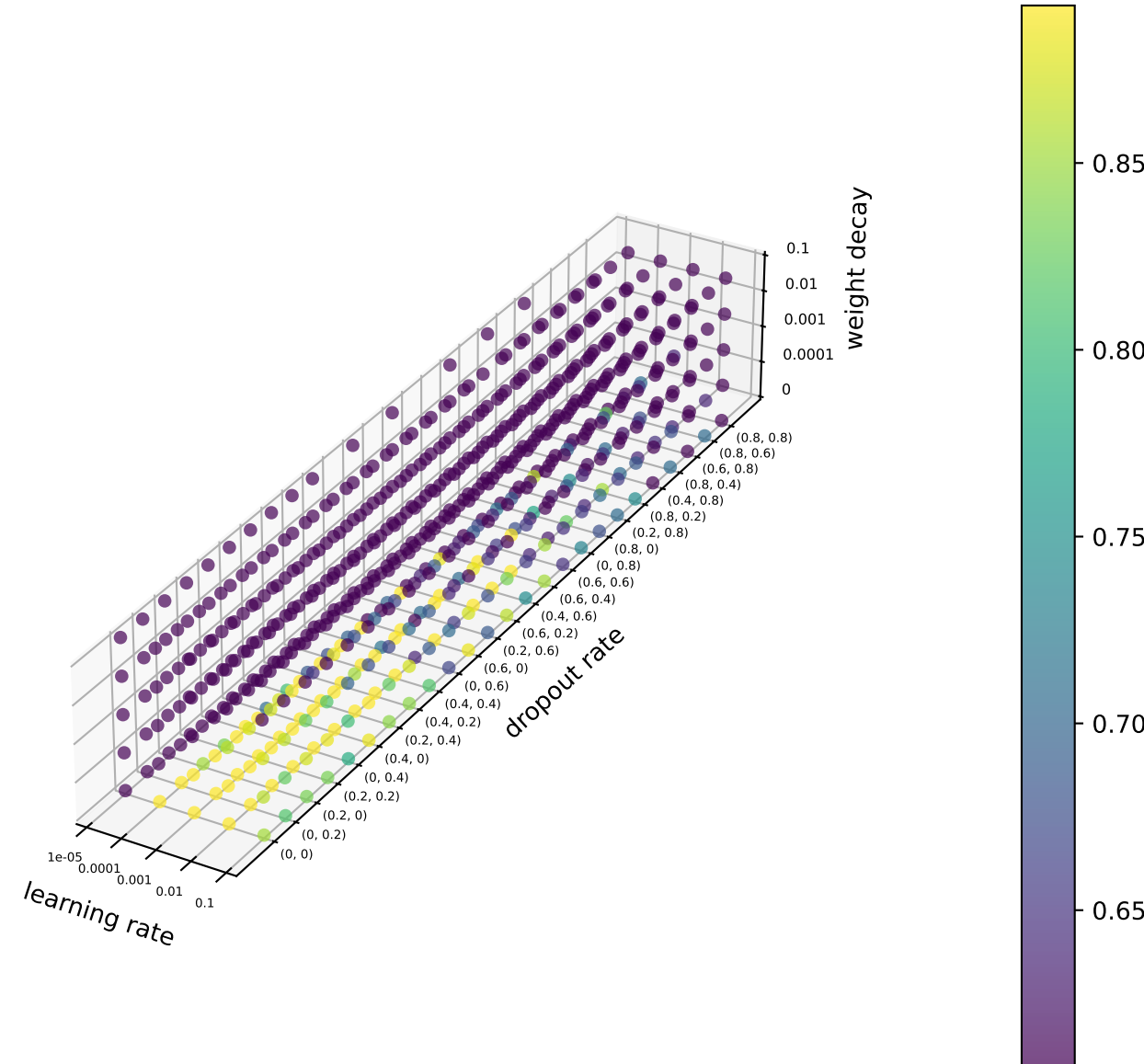
Accuracy
