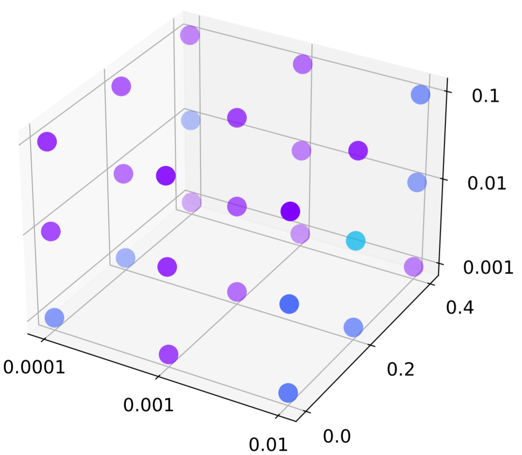
GCN2MLP
