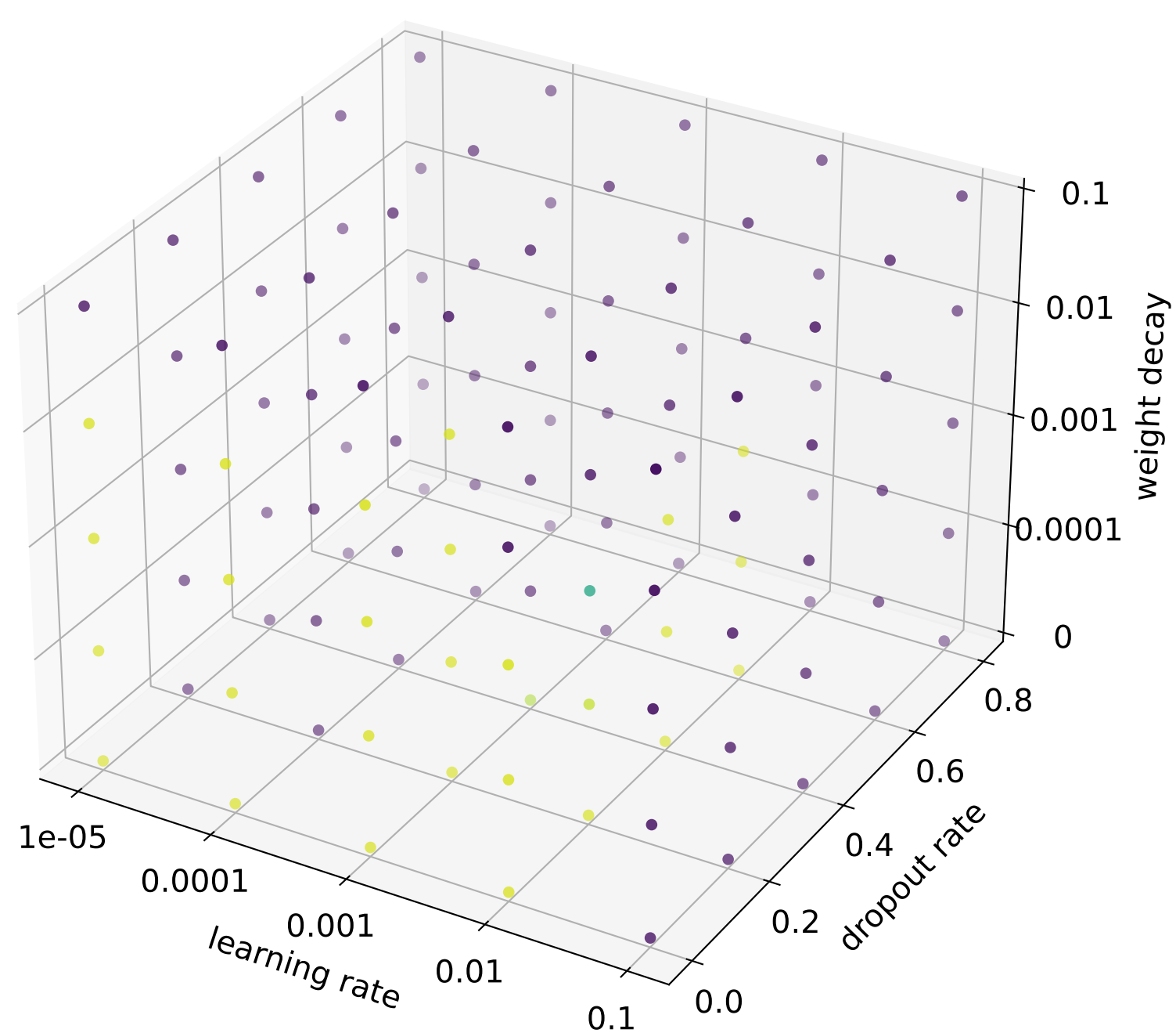
LightDeepChebNet
