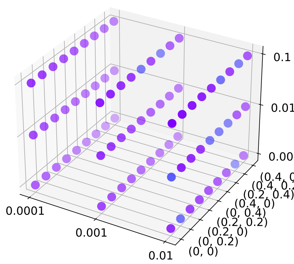
xDenseChebNet2MLP
