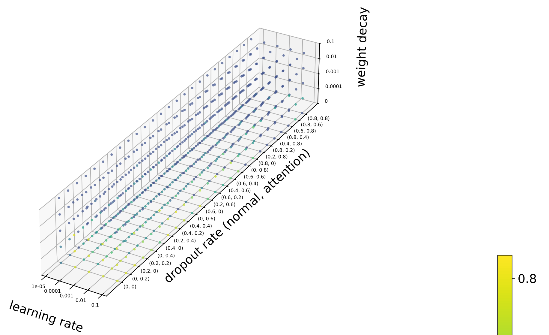
CoarseningGCN2MLP
