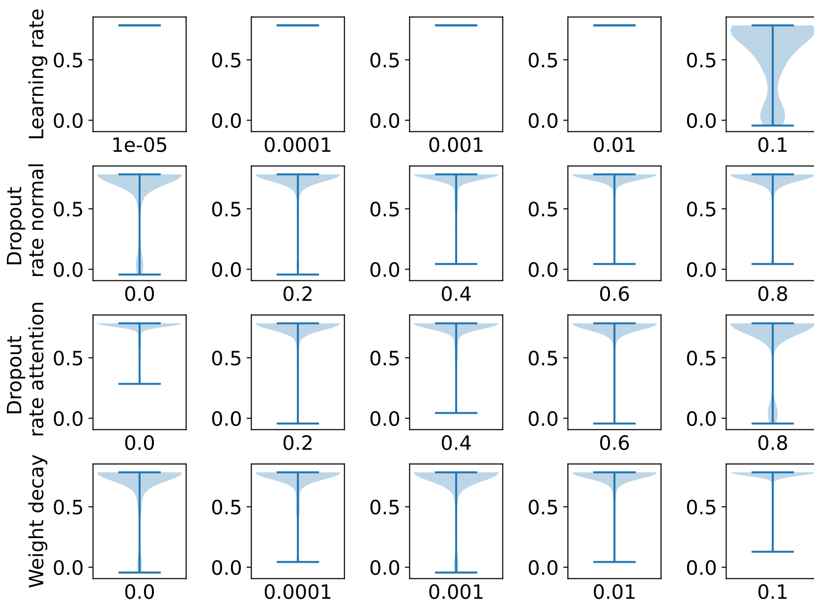
LightGAT2MLP
