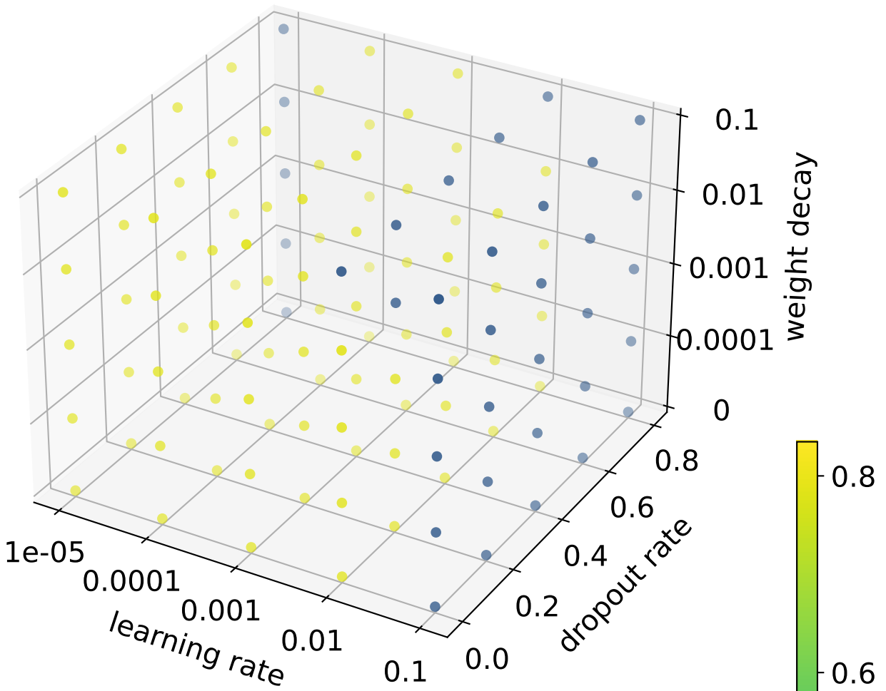
LightDeepGCN2MLP
