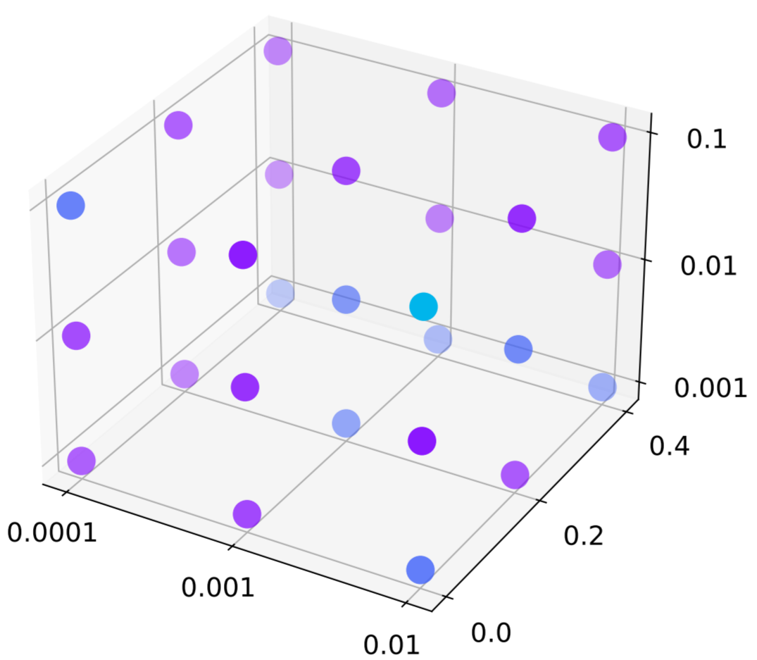
ResGCN2MLP
