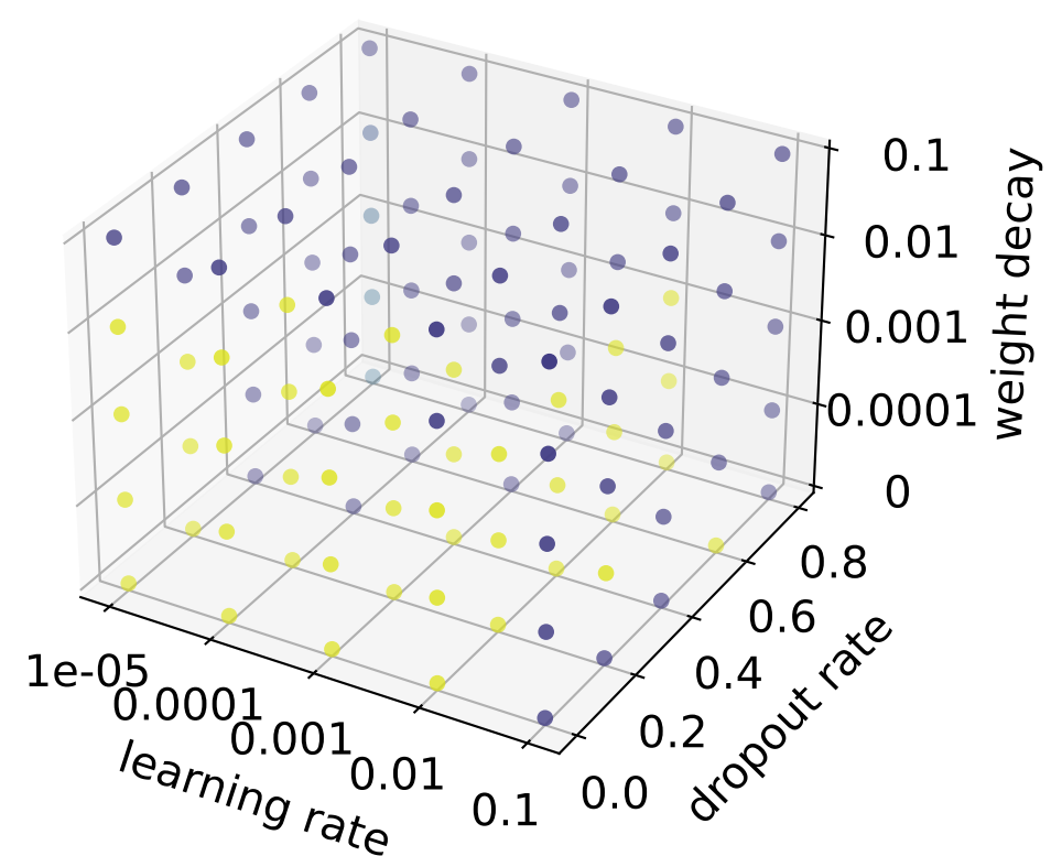
ResChebNet
