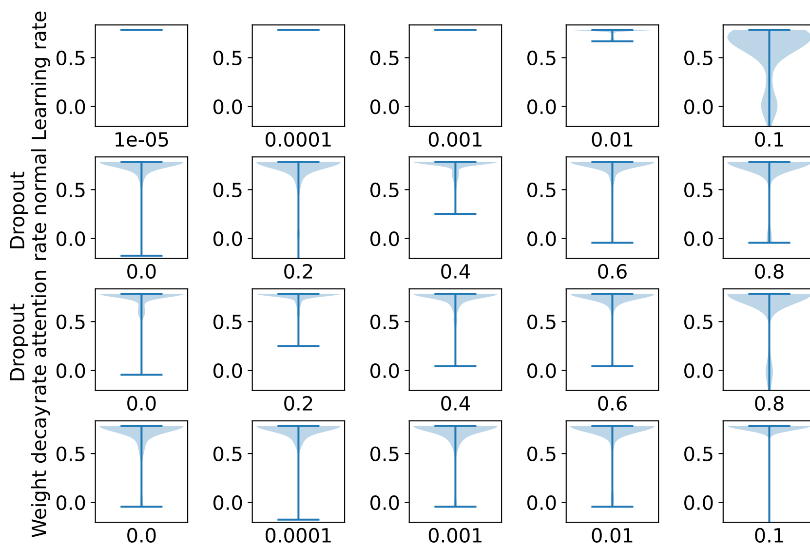
CoarseningGAT2MLP
