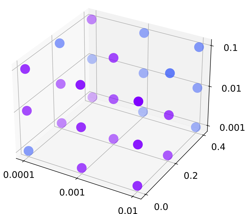
mDenseGAT2MLP
