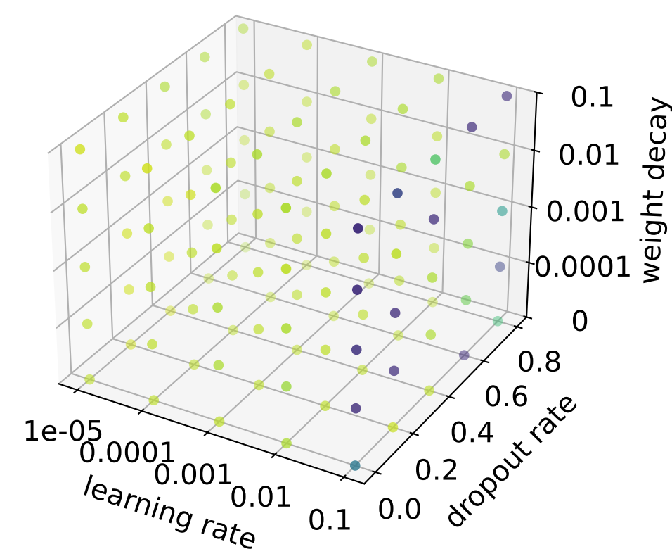
xDenseChebNet2MLP
