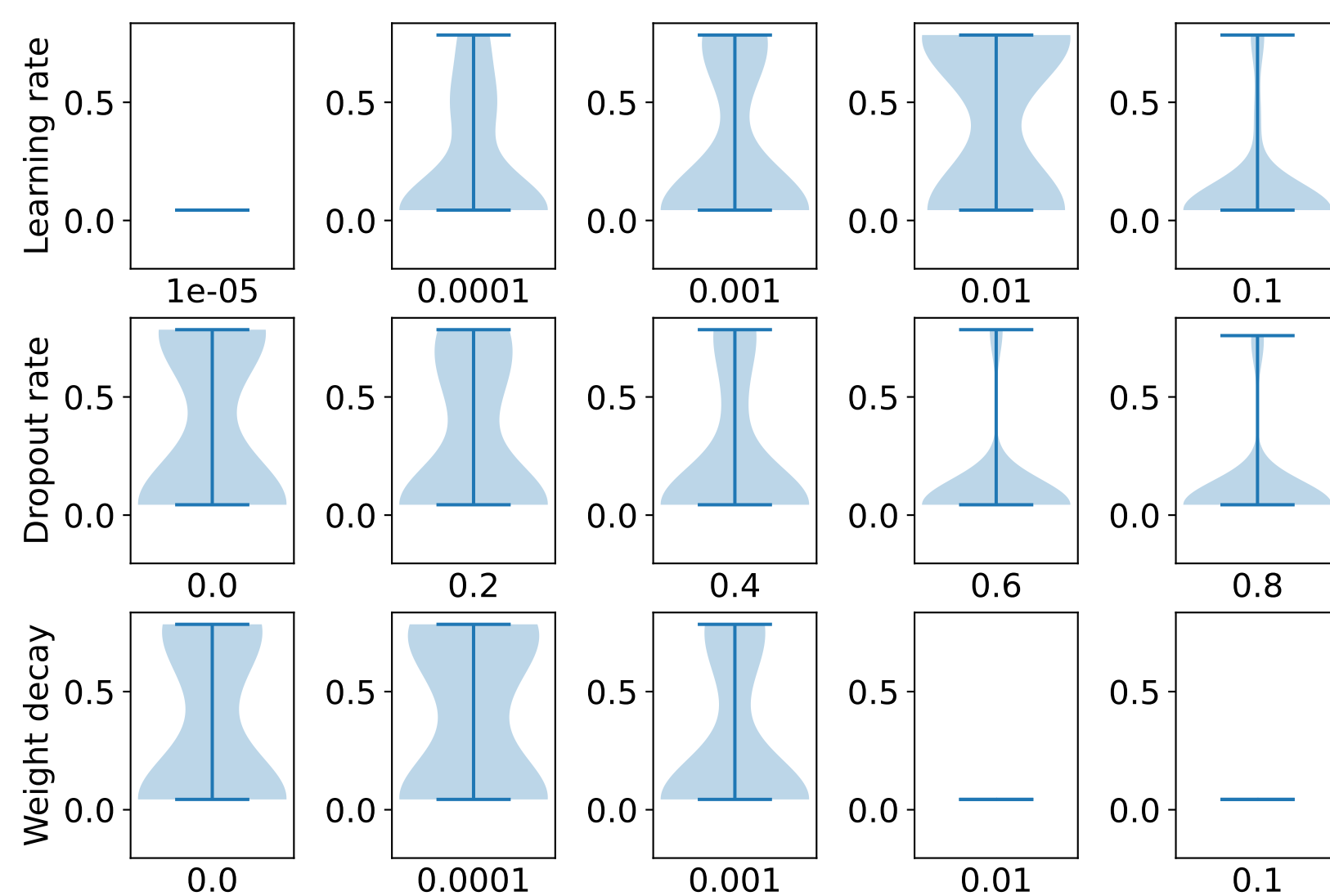
CoarseningChebNet
