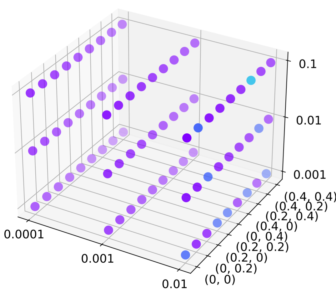
GAT2MLP
