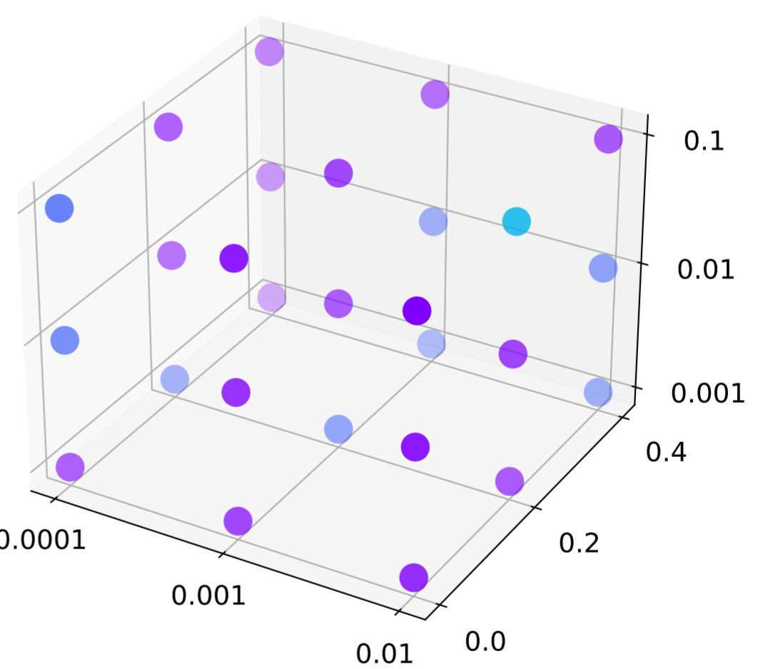
DenseGCN2MLP
