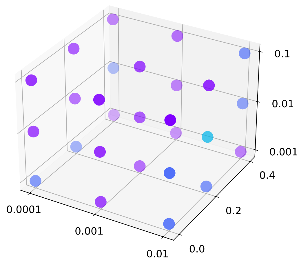
GCN2MLP
