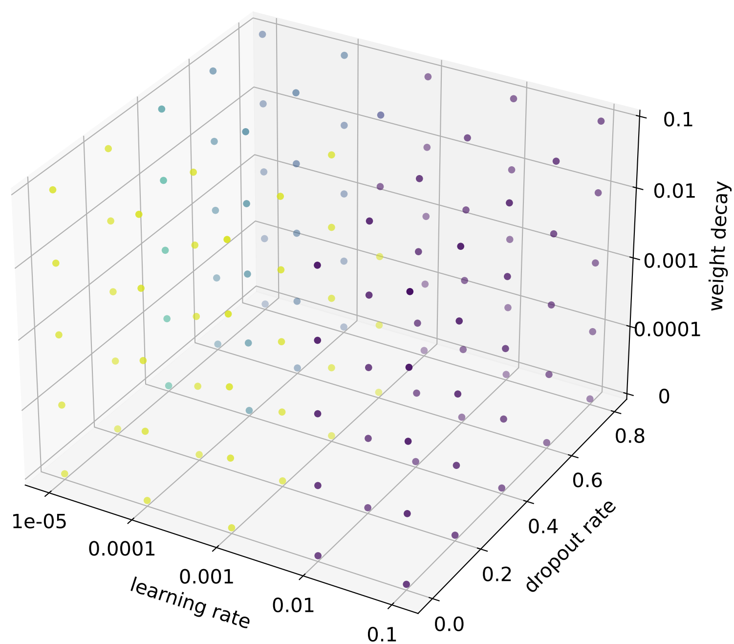
LightDeepChebNet2MLP
