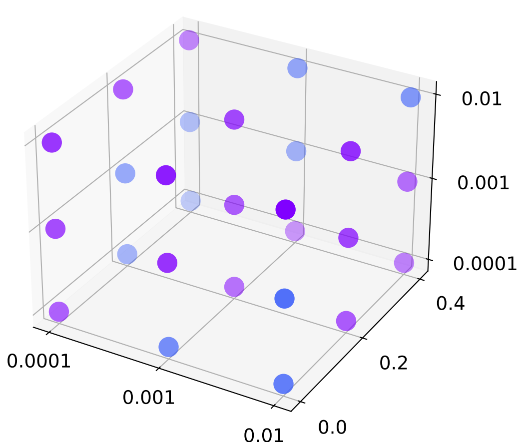
mDenseChebNet2MLP
