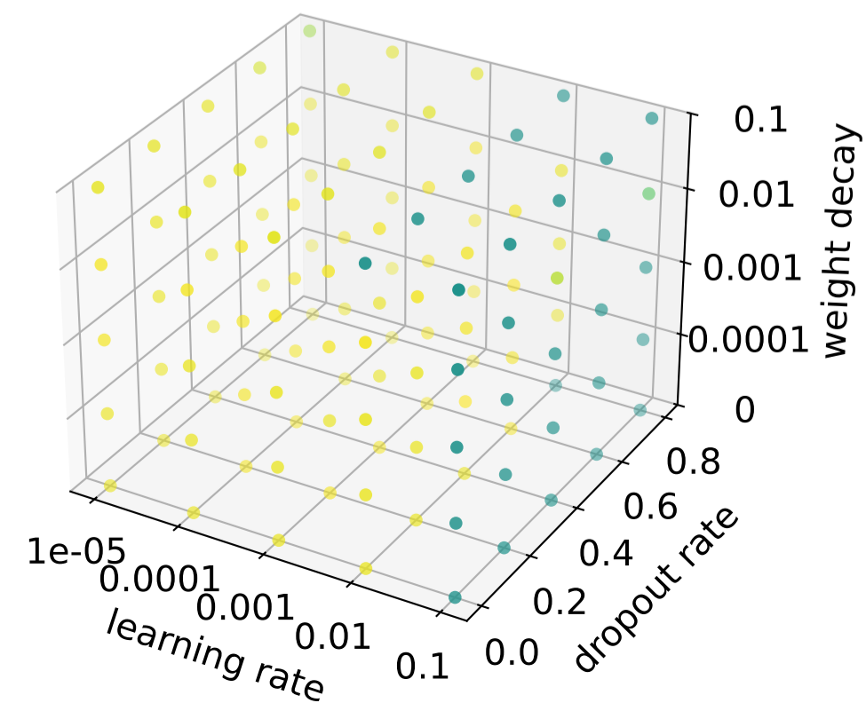
xGCN2MLP
