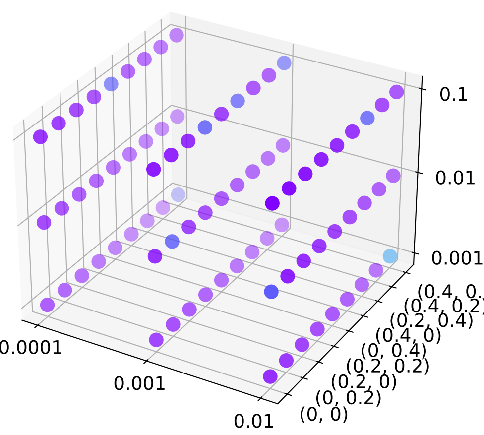
xChebNet2MLP
