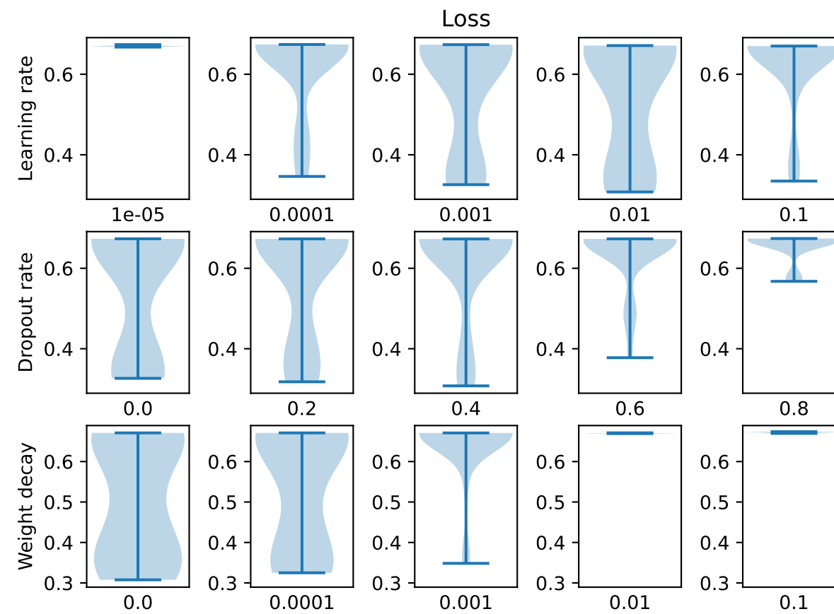
ResGCN (only methylation data)
