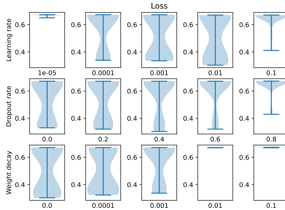
ResGCN (full batch)
