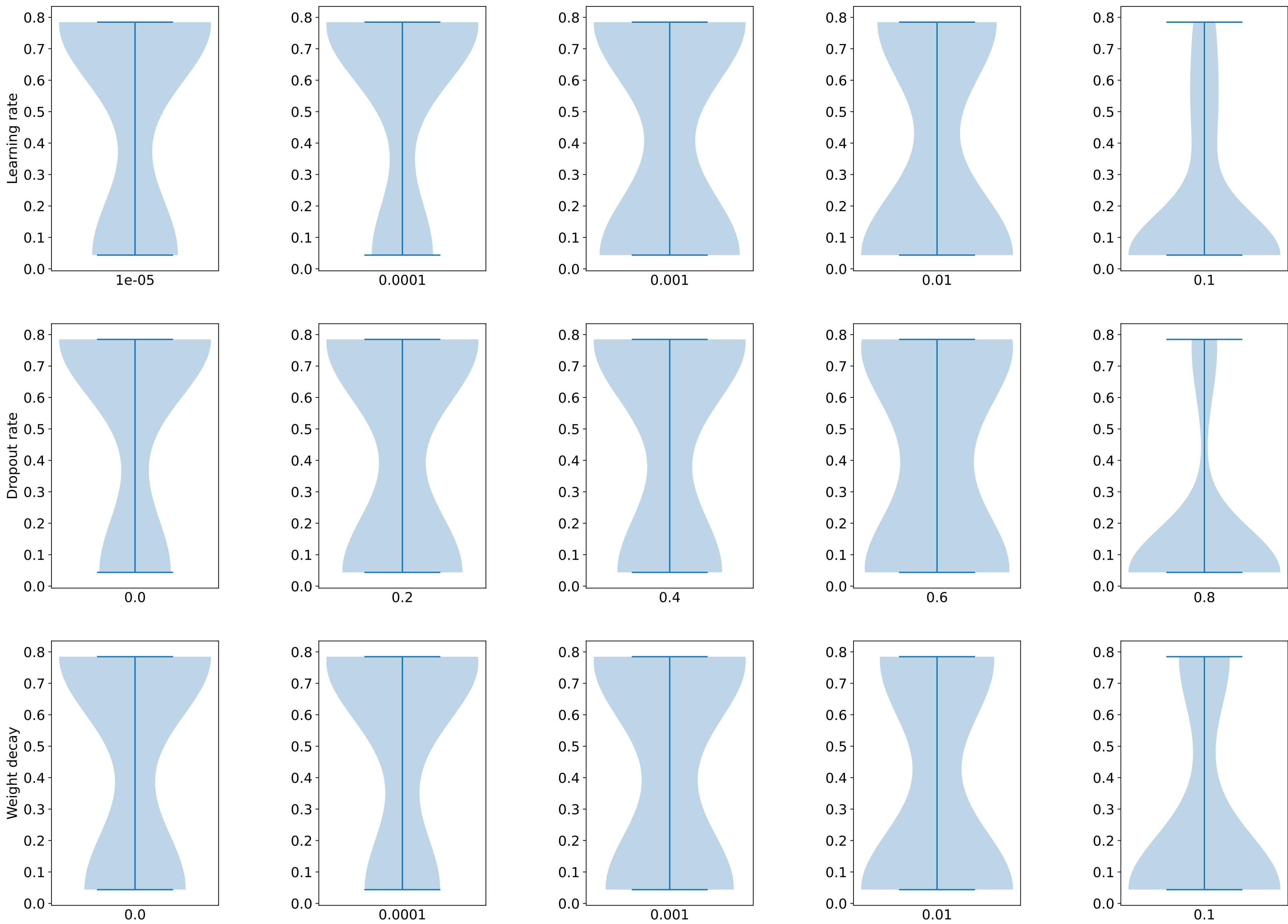
Testrun hyperparameter MCC results, full data, MLP_Larger
