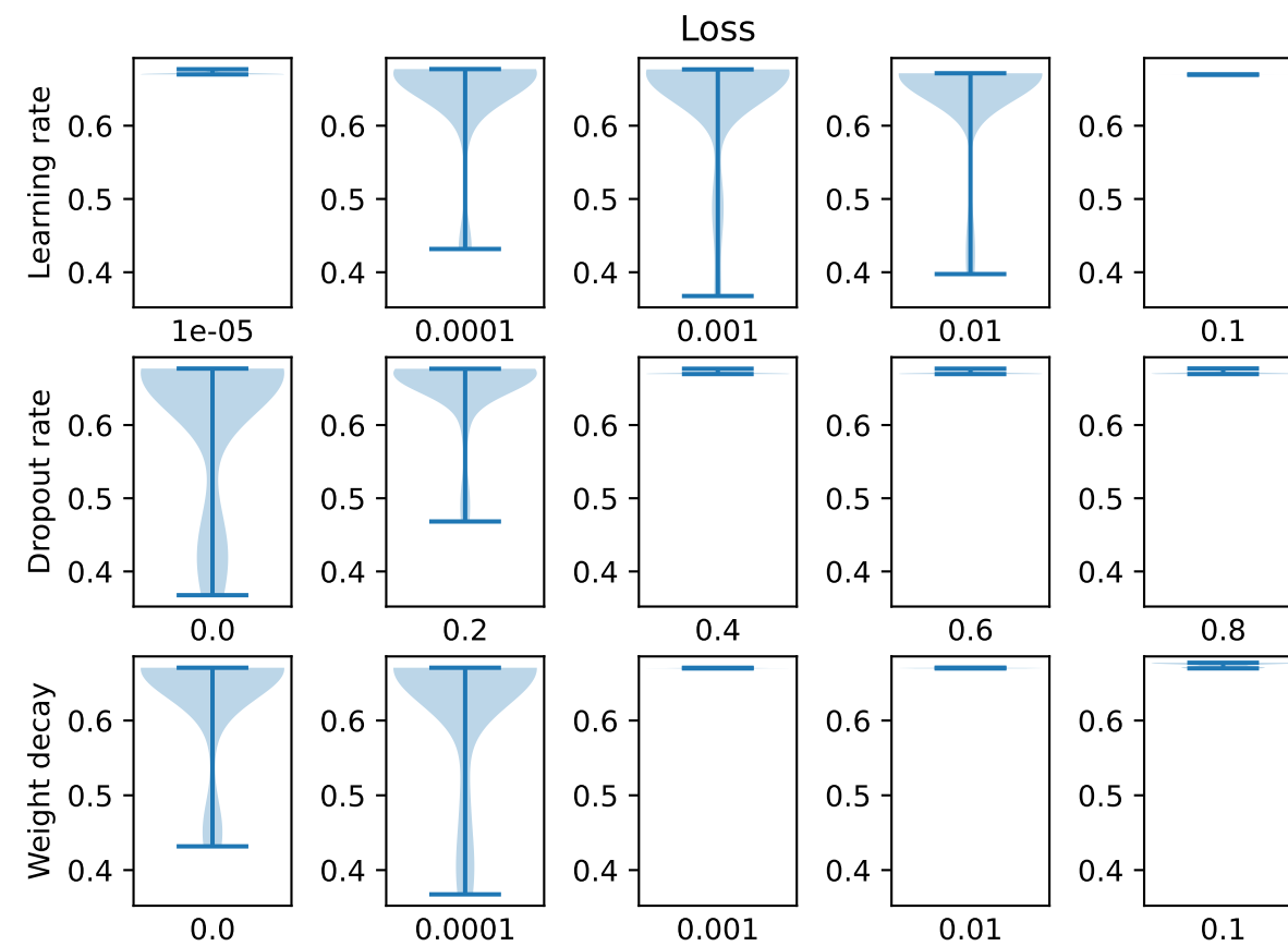
DenseGCN (only expression data)
