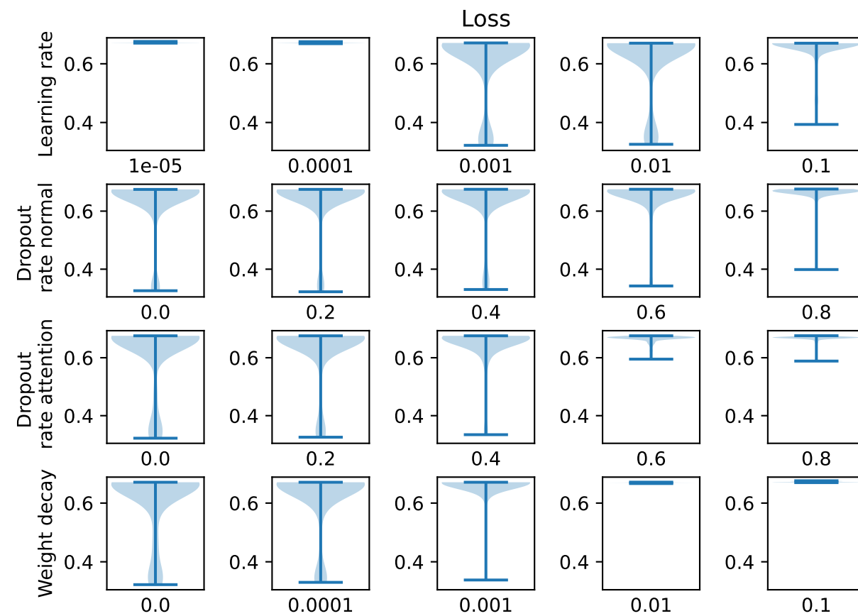
GAT (batch size 64)
