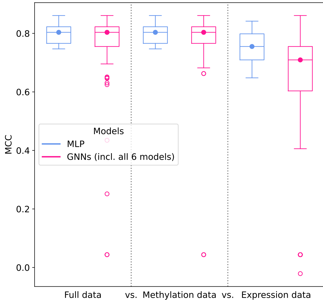
Test results plain MLP vs. GNNs for different data modalities
