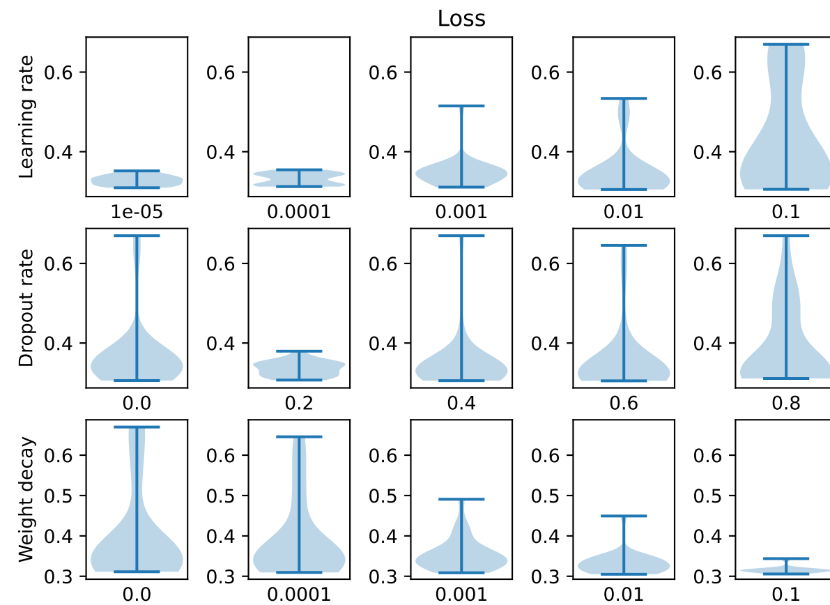
DenseMLP (full batch)
