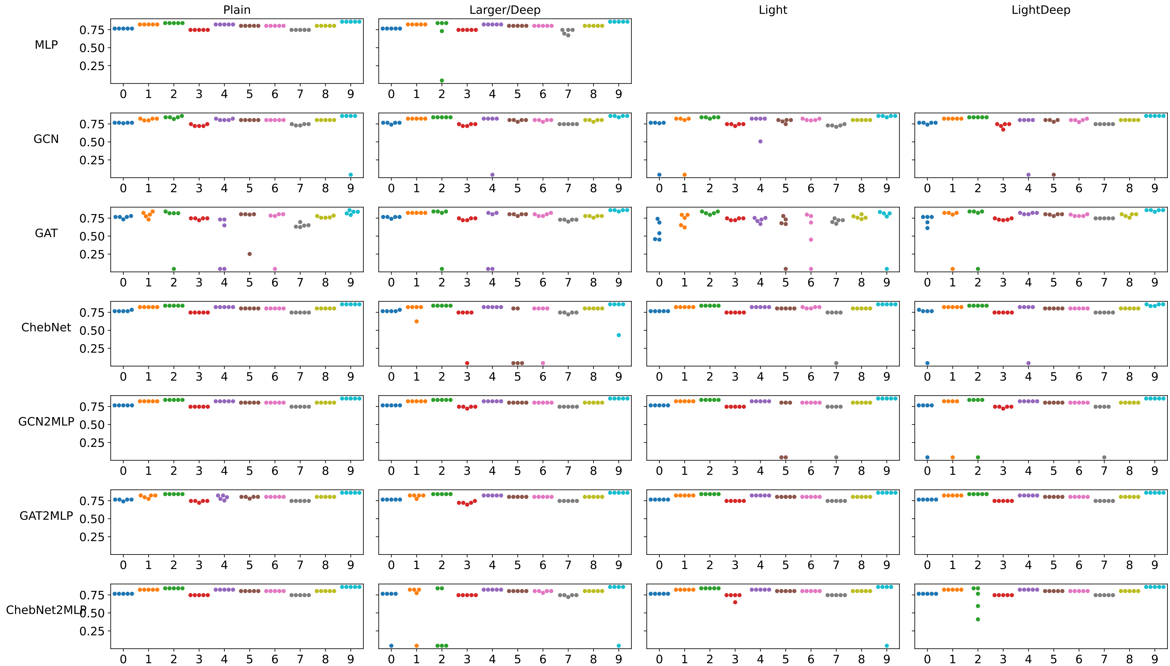
Results per outer test round in MCC for Deep, Light and LightDeep models
