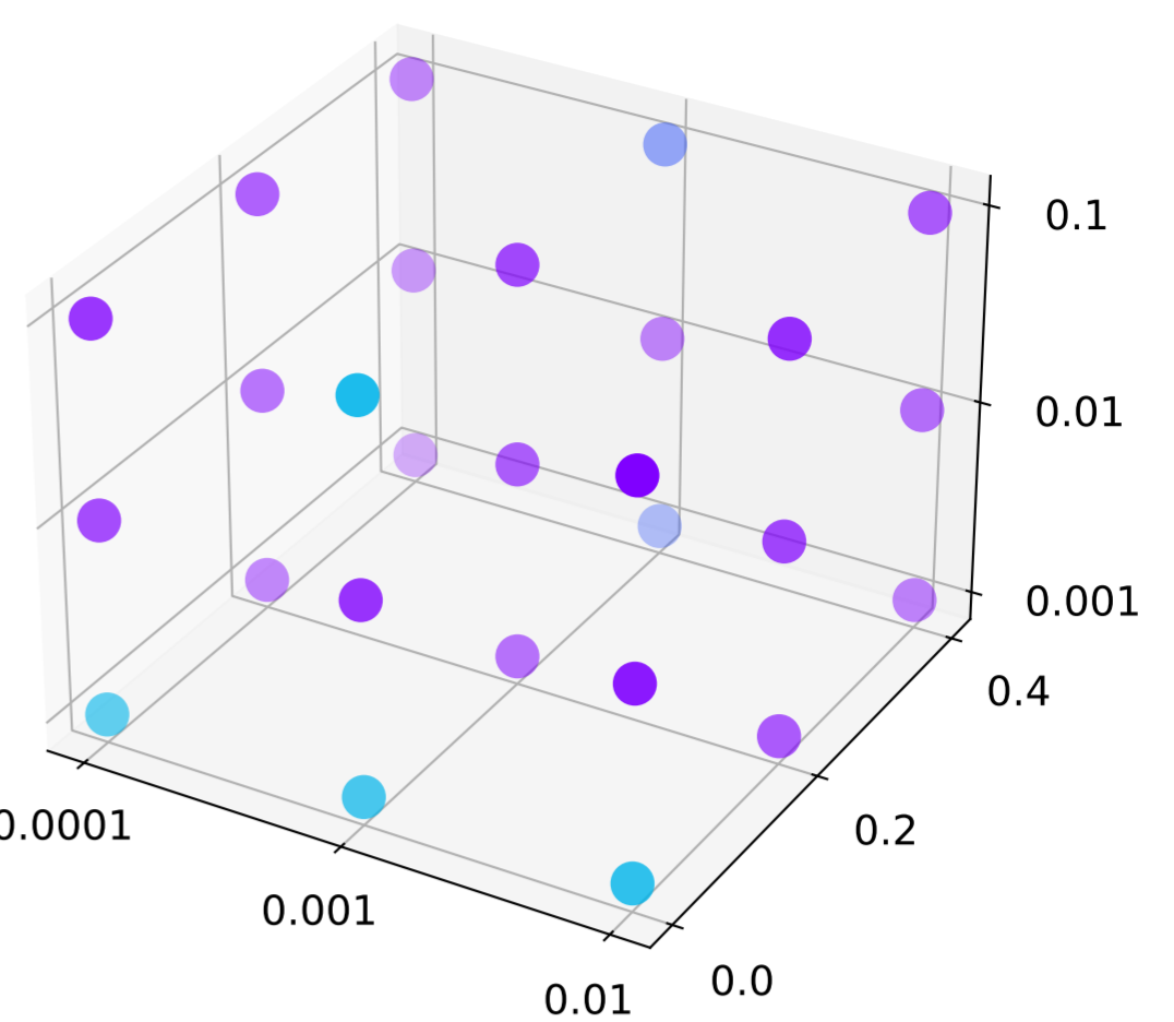
DenseMLP
