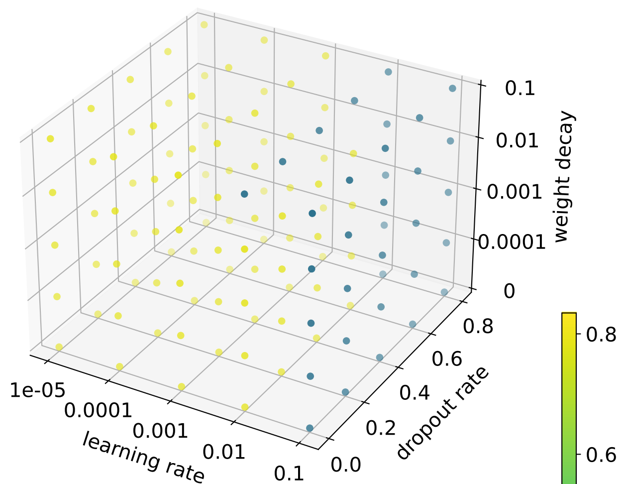
DeepGCN2MLP
