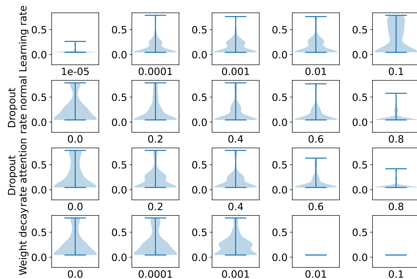
CoarseningGCN2MLP
