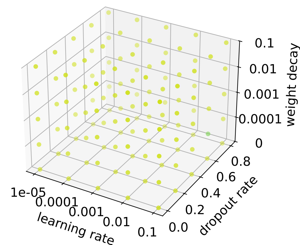
mDenseChebNet2MLP
