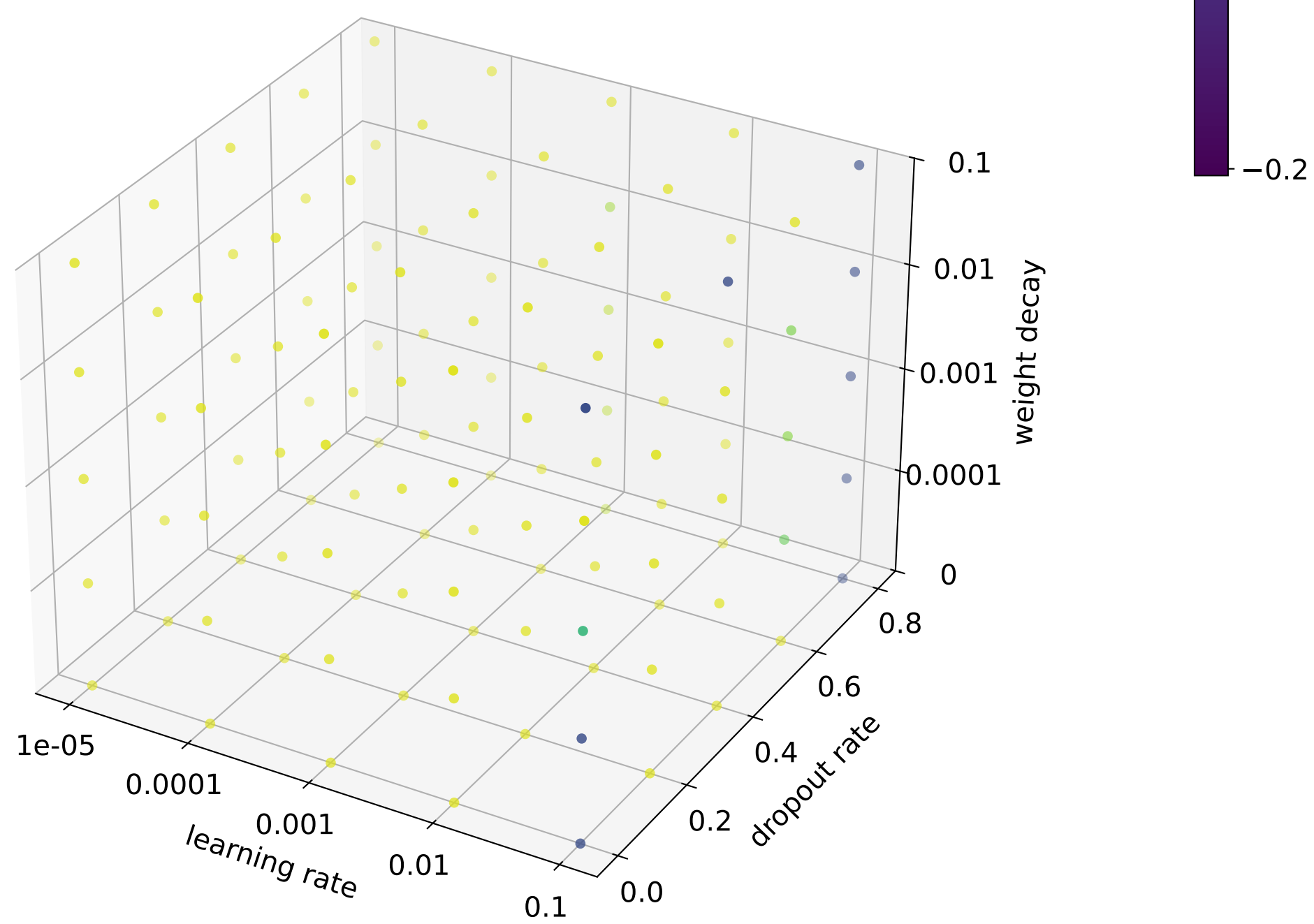
CoarseningChebNet2MLP
