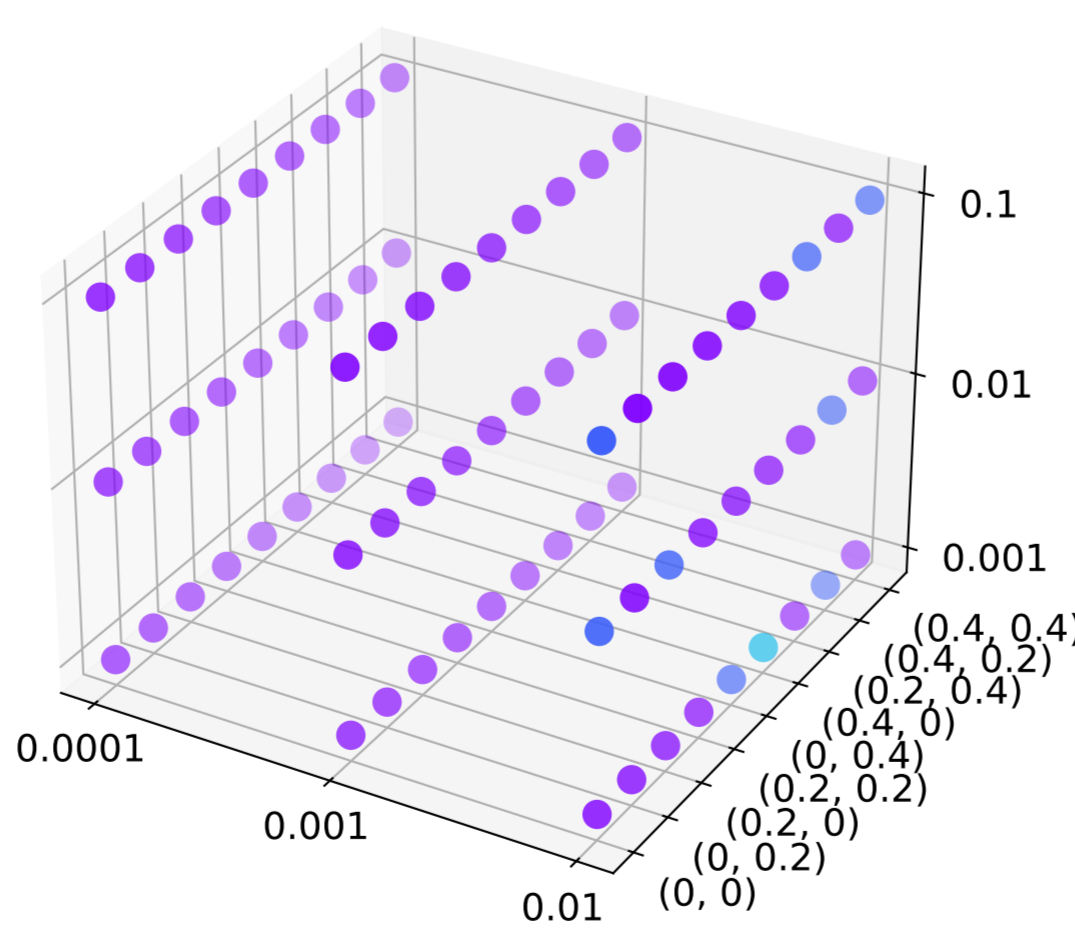
ResGAT2MLP
