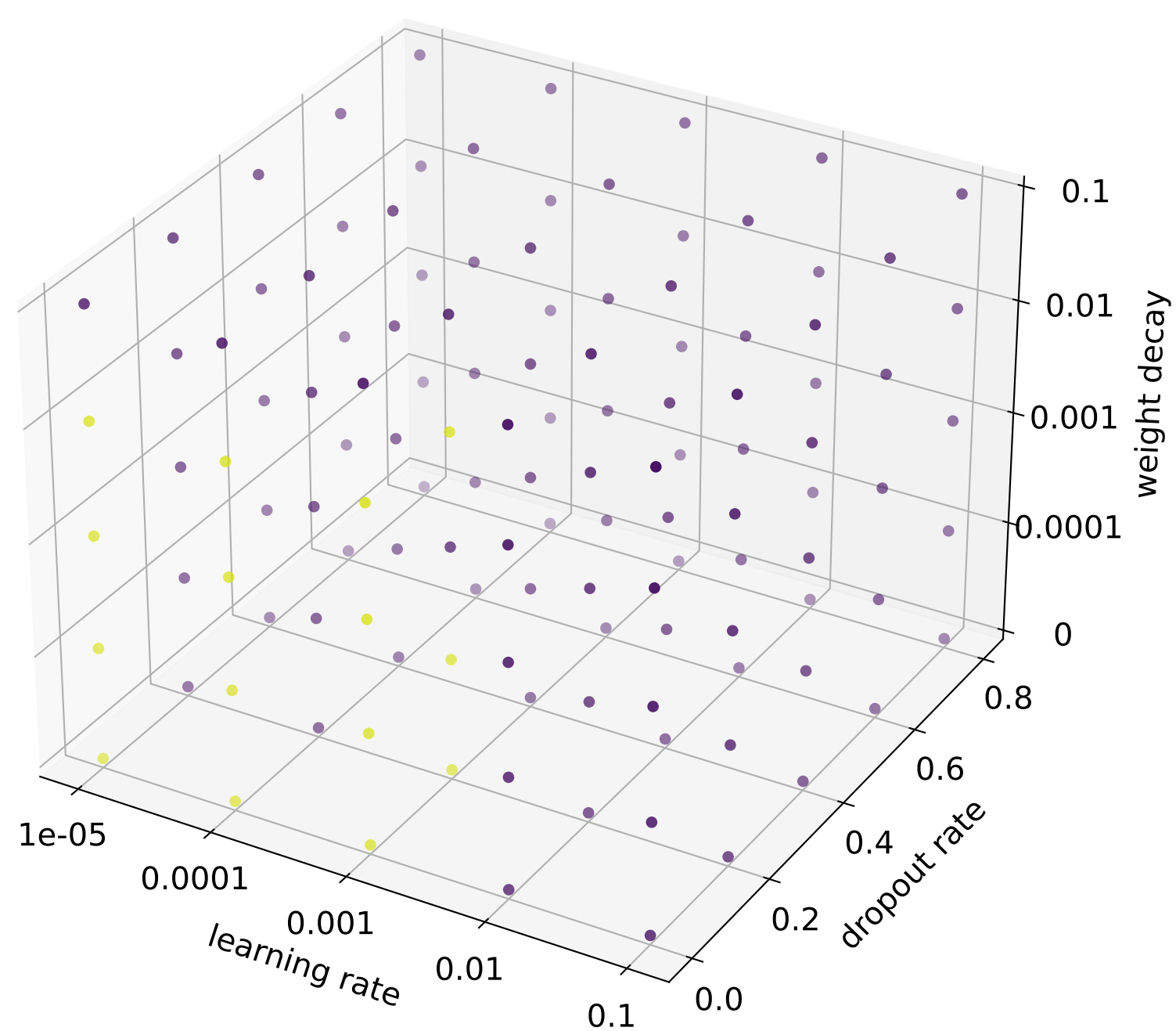
LightDeepChebNet
