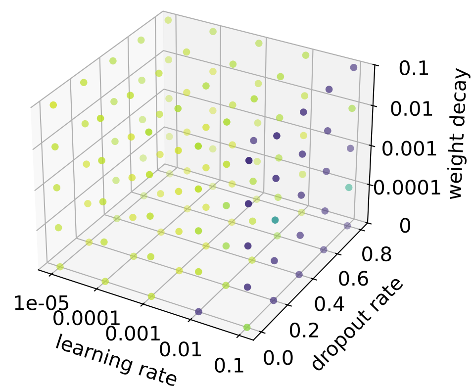
xChebNet2MLP
