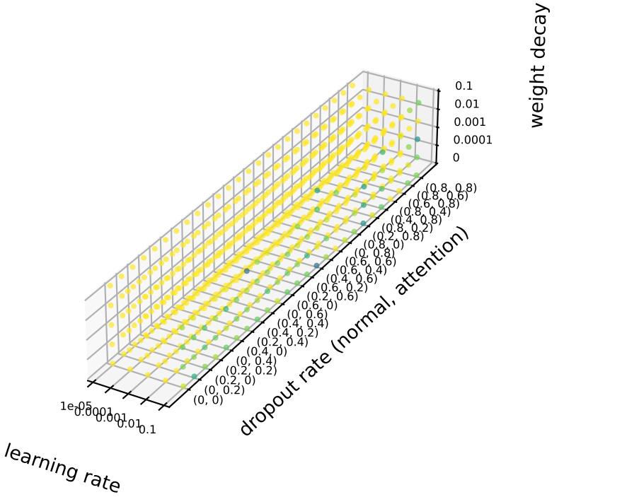
mResGAT2MLP
