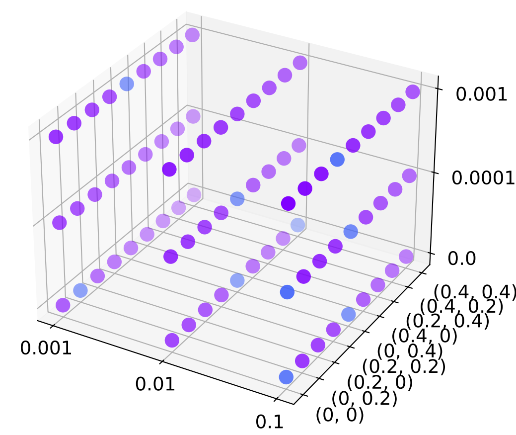
mResChebNet
