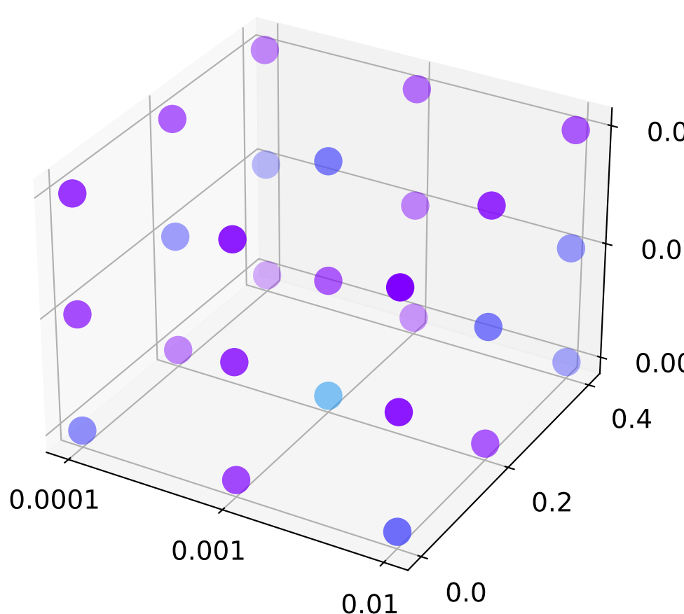
xDenseGAT2MLP
