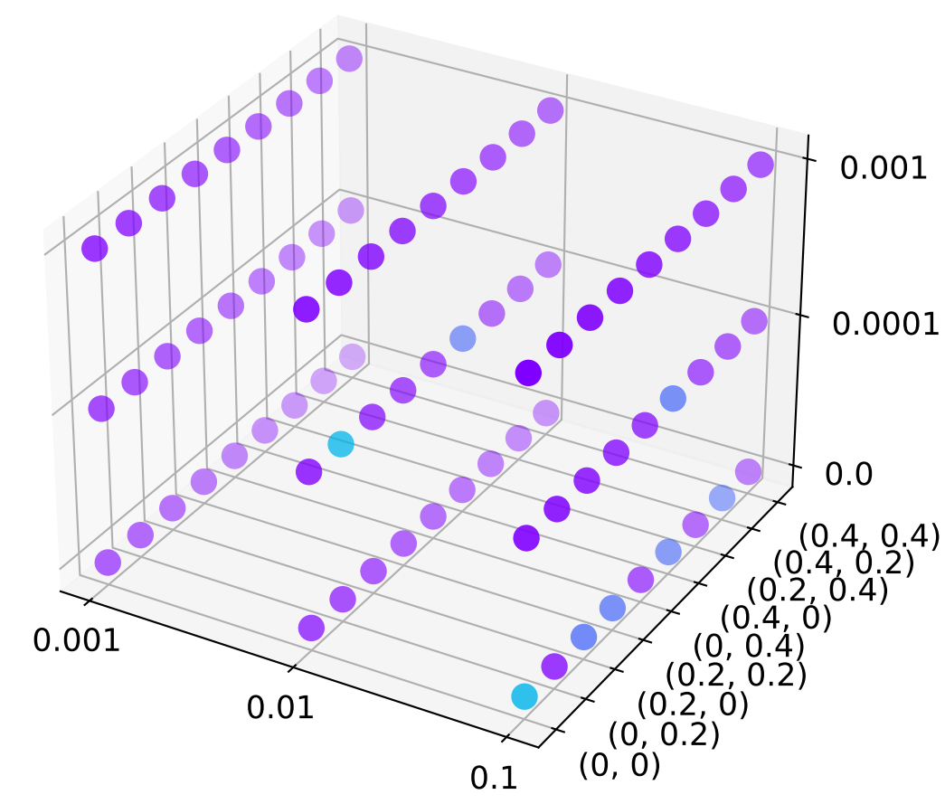
ChebNet2MLP
