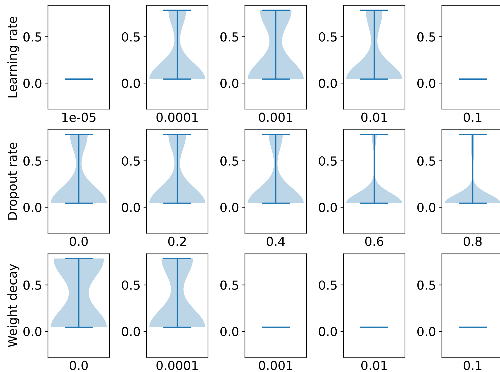
LightDeepGAT
