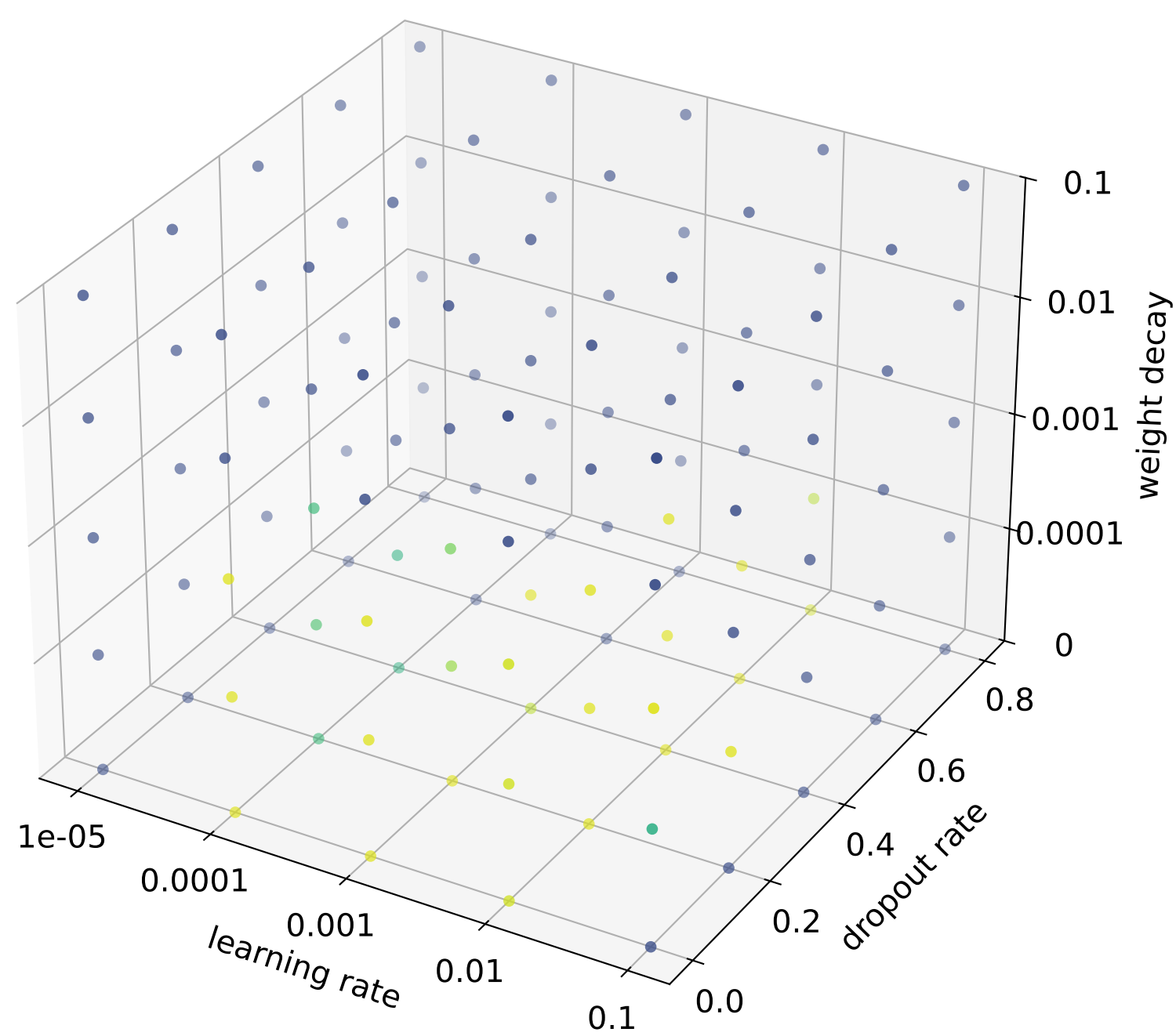
CoarseningChebNet
