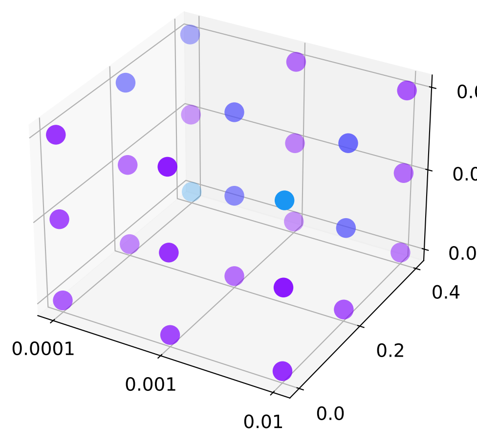
xResChebNet2MLP
