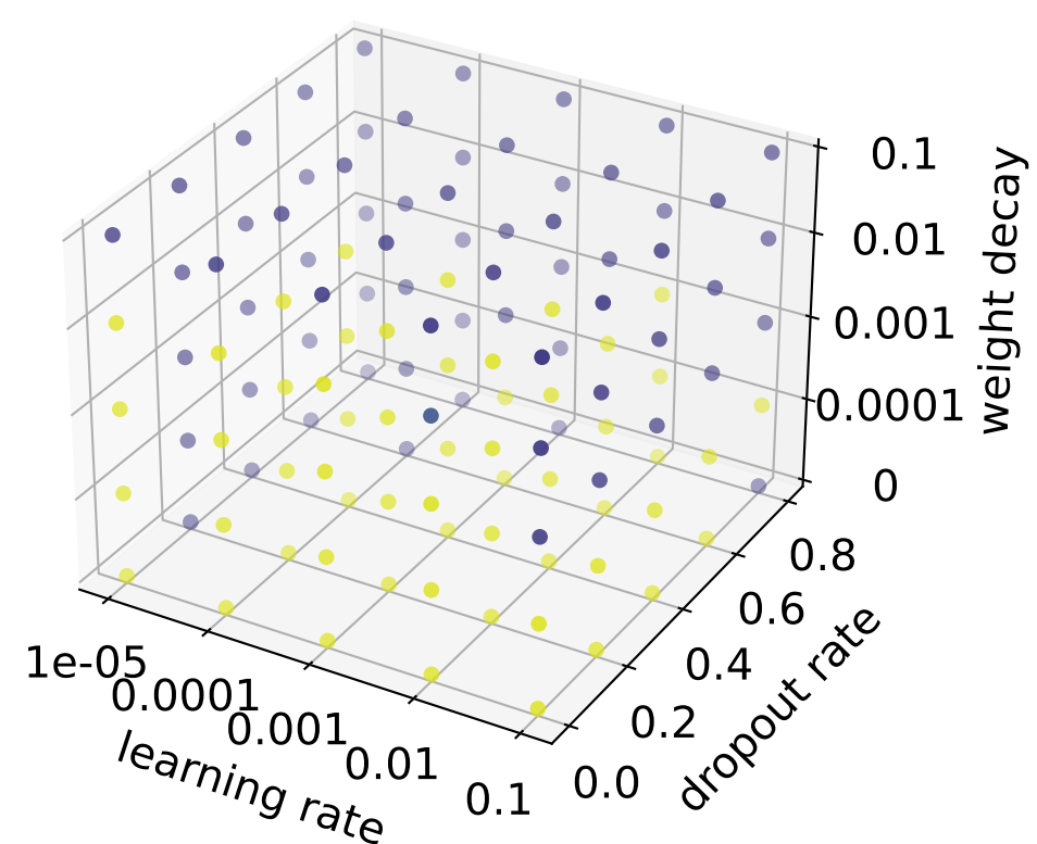
mResChebNet
