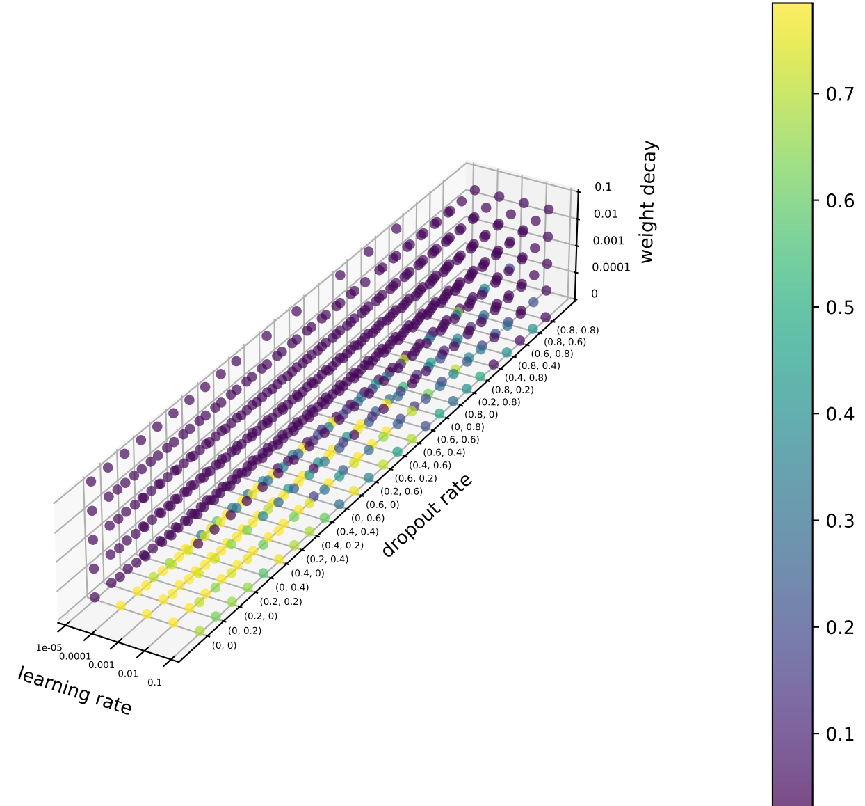
MCC
