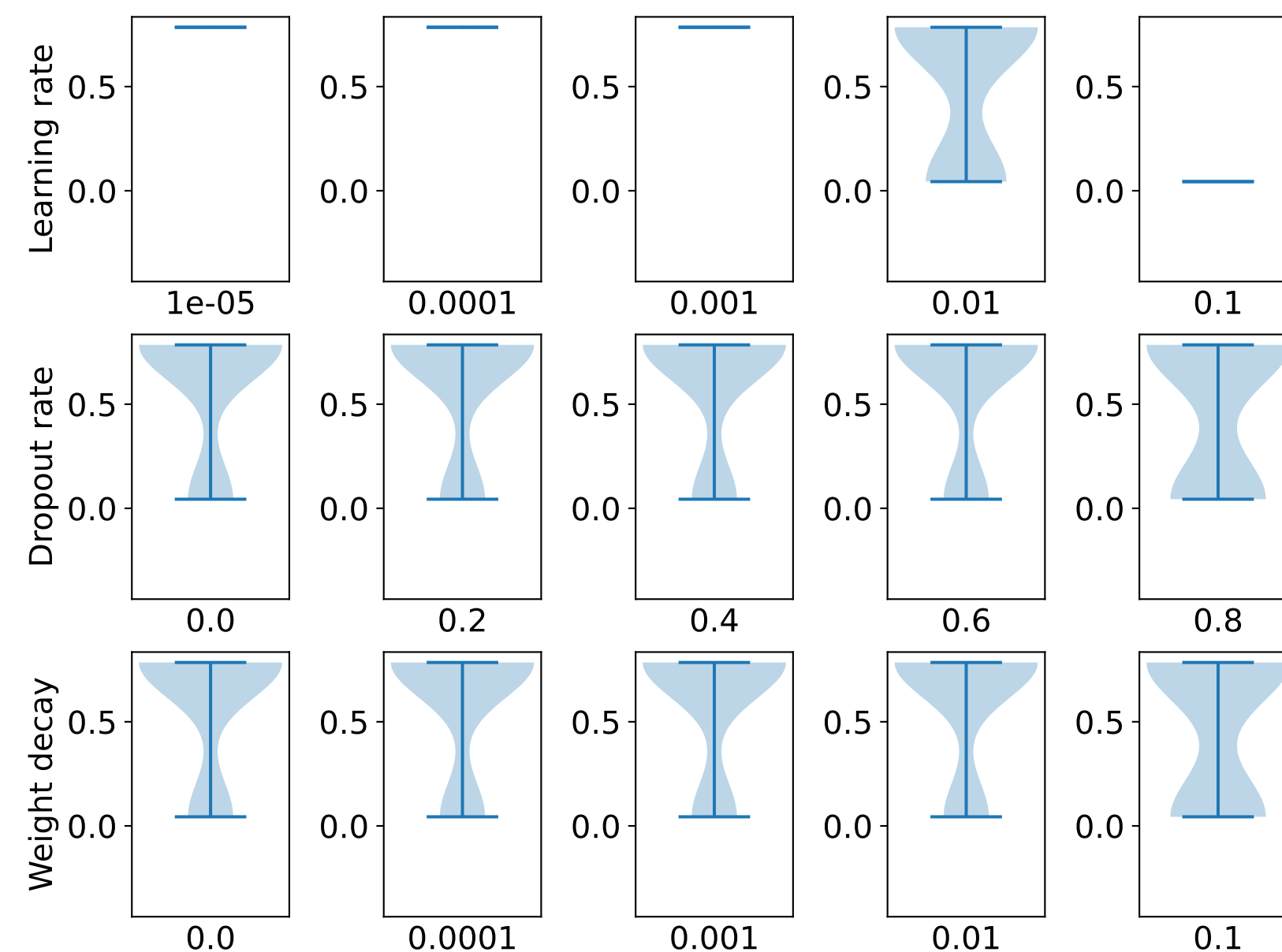
DeepGAT2MLP
