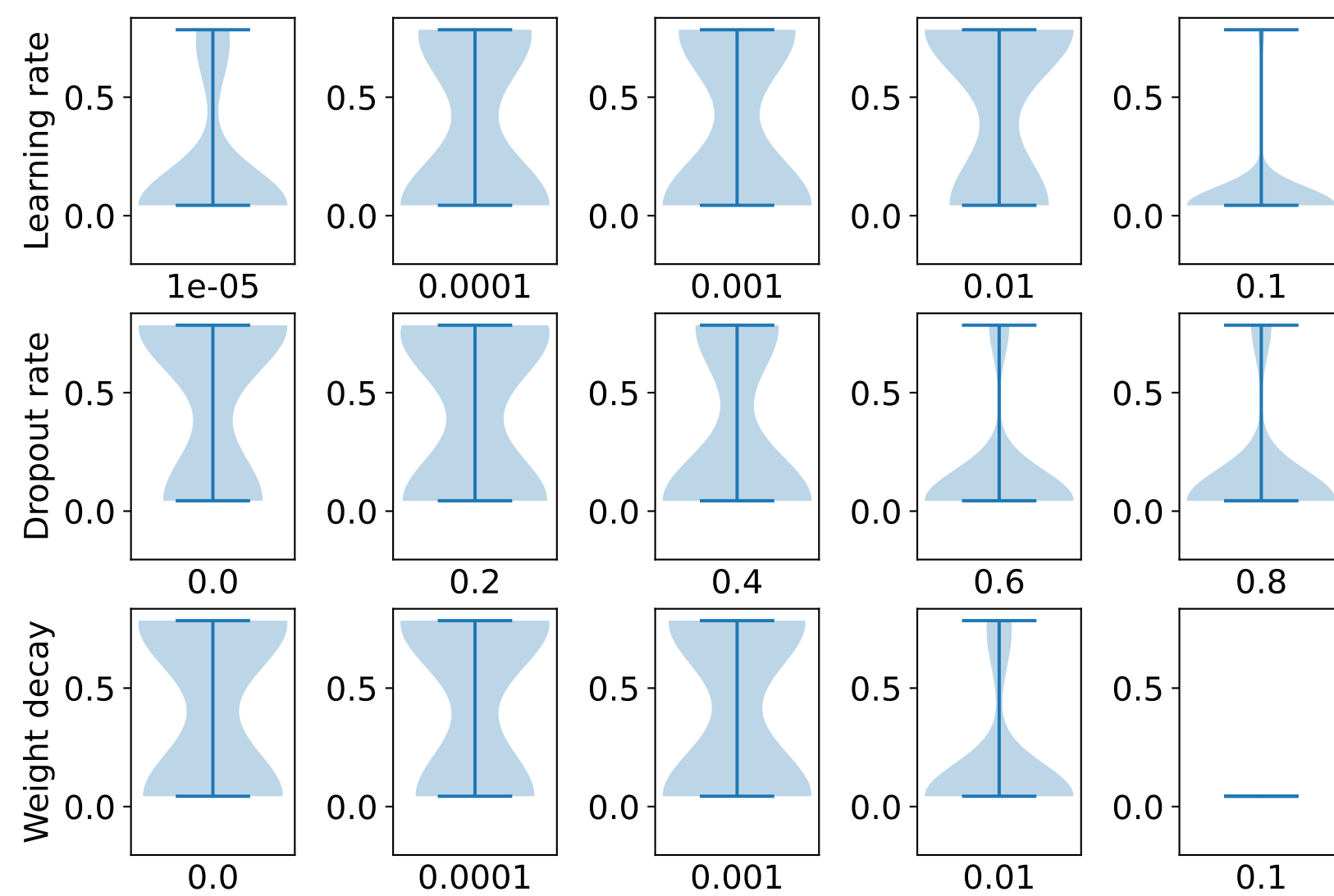
CoarseningGAT2MLP
