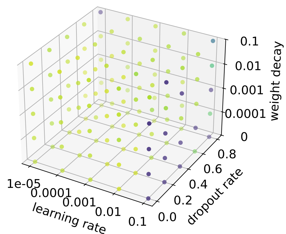
xResChebNet2MLP
