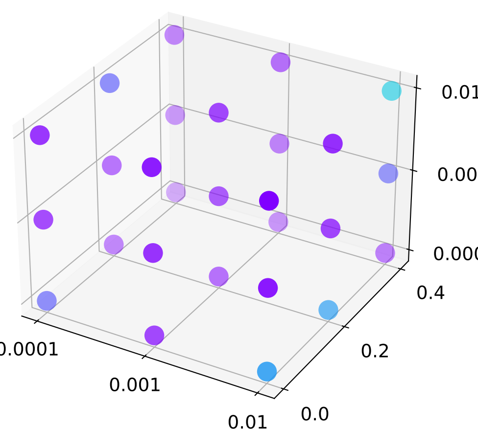
xGAT2MLP
