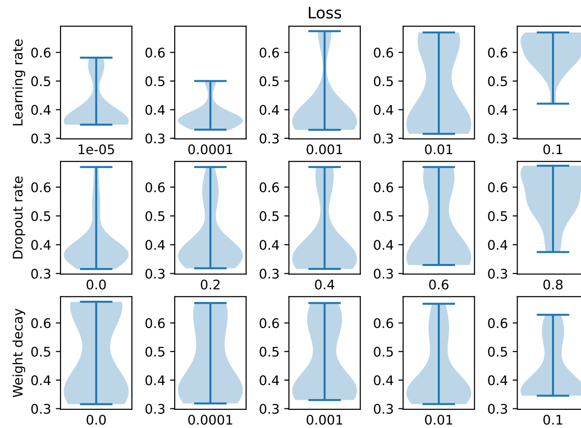
ResMLP (only expression data)
