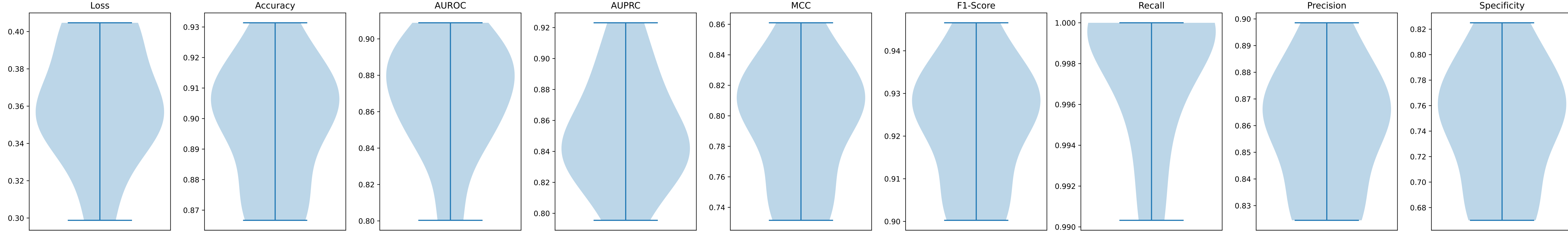
DenseGCN - Average metric test results (av. over outer folds)
