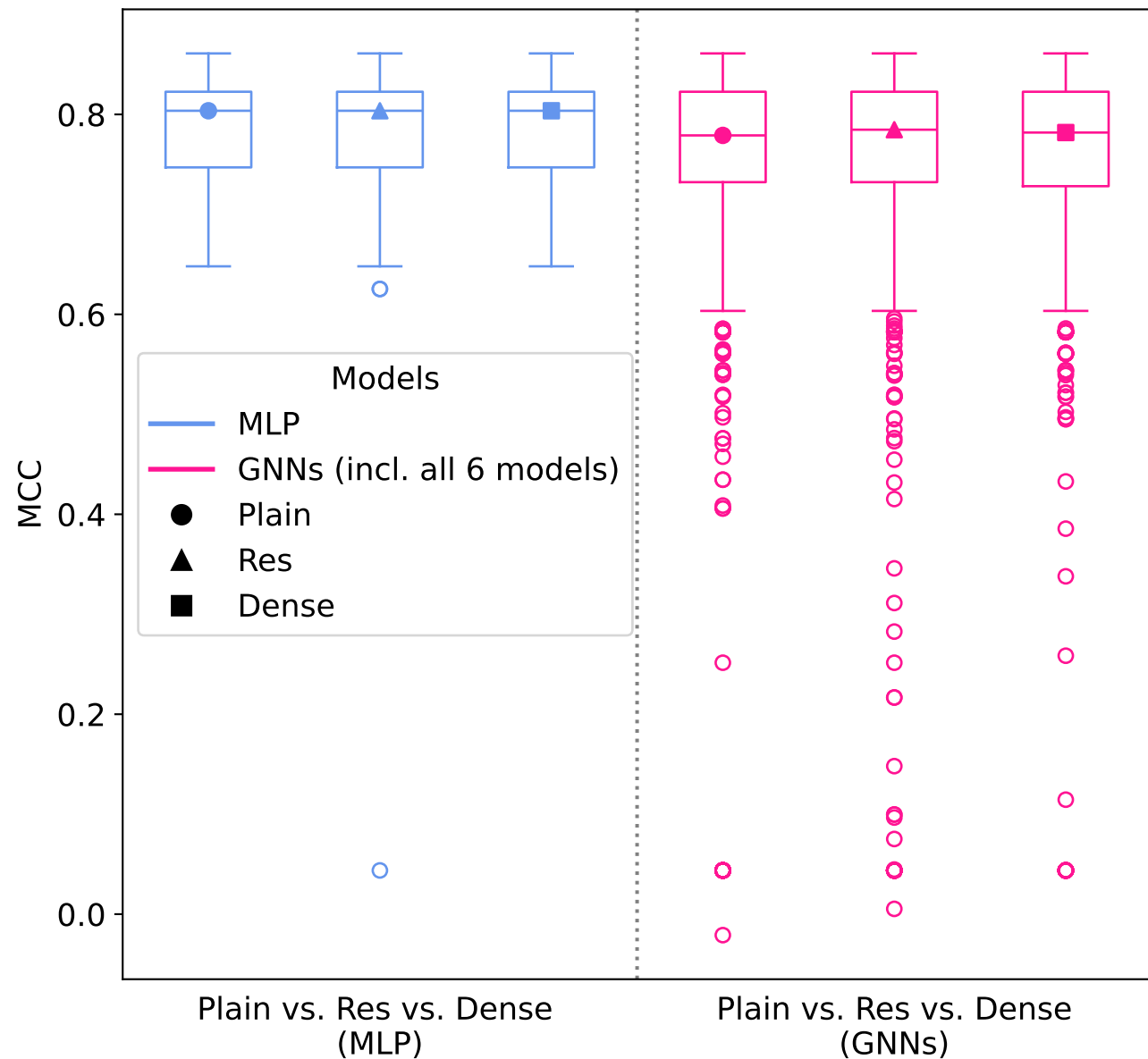
Test results for Plain vs. Res vs. Dense for MLP and GNNs over all data modalities
