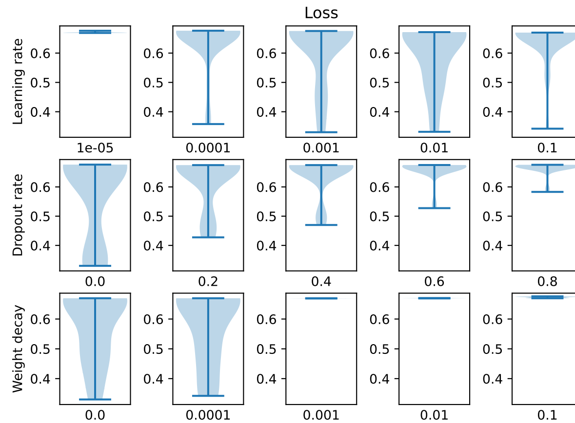
GCN (only methylation data)
