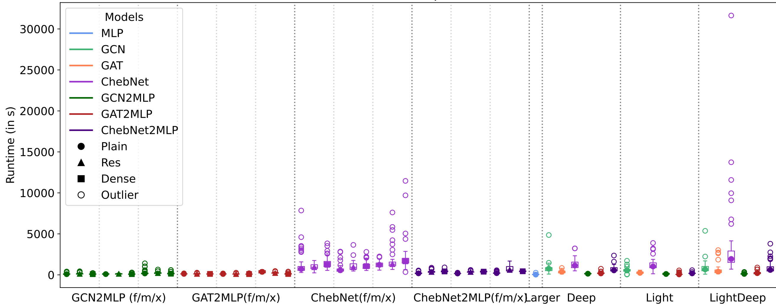
Run time over all outer splits for new models
