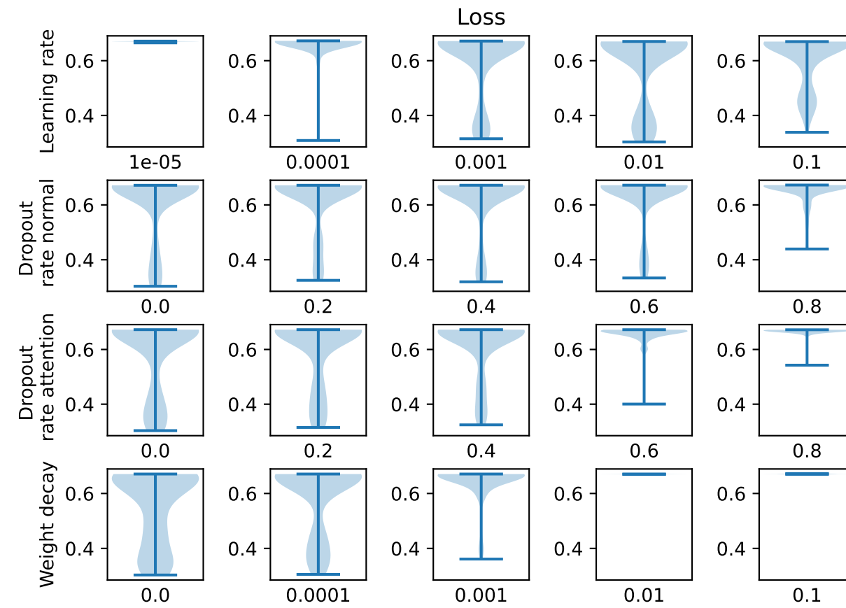
GAT (only methylation data)
