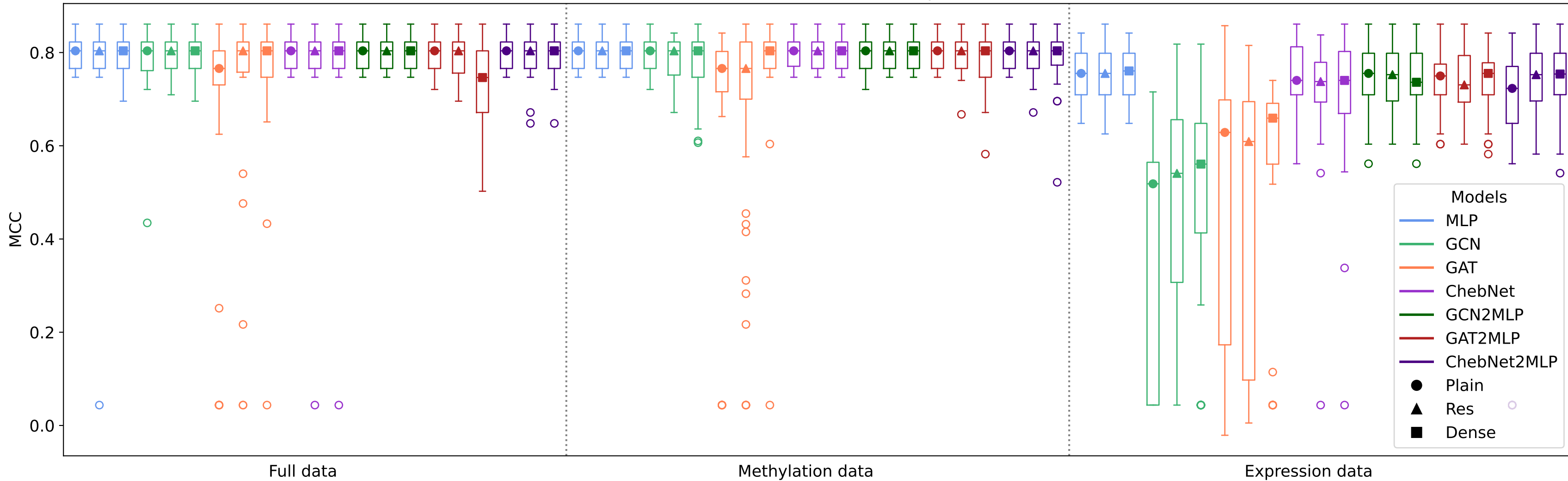
Test results over all outer splits
