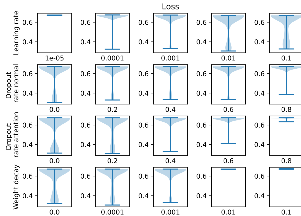
GAT (full batch)
