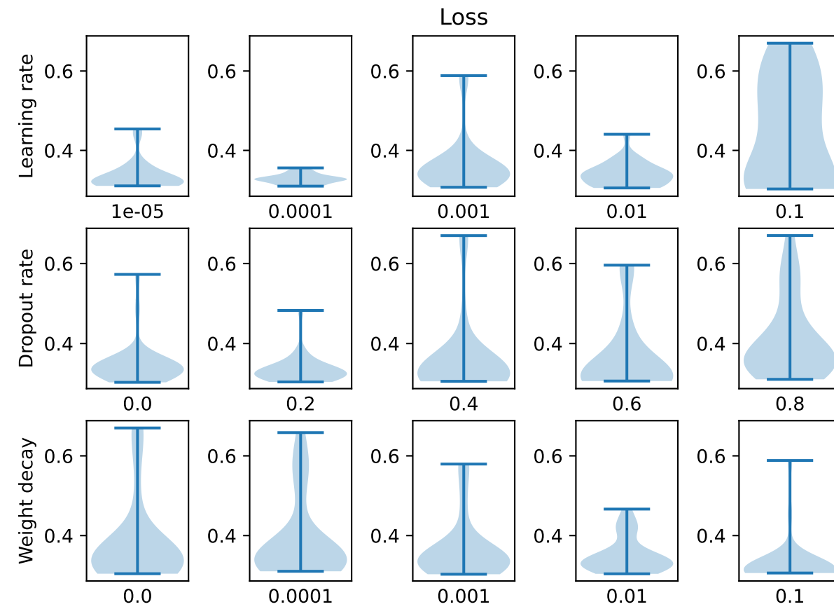
ResMLP (full batch)
