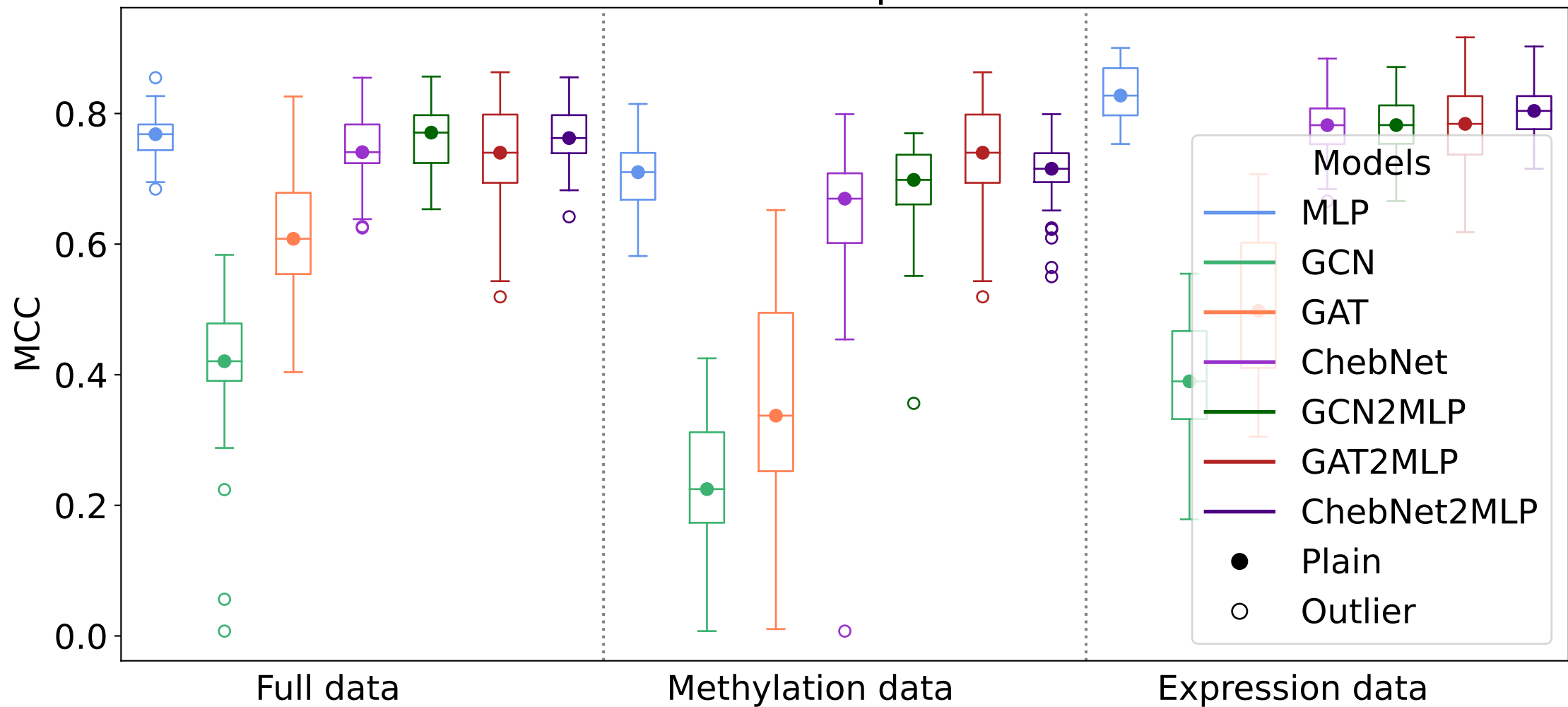
Test results over all outer splits for all Plain models
