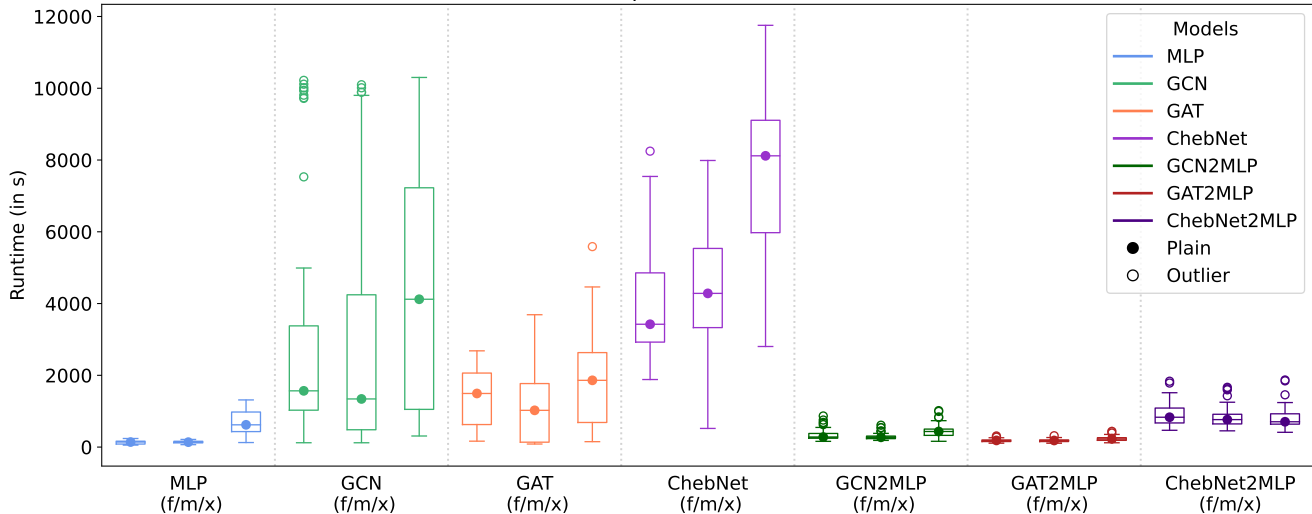
Run time over all outer splits for all Plain models for BRCA data
