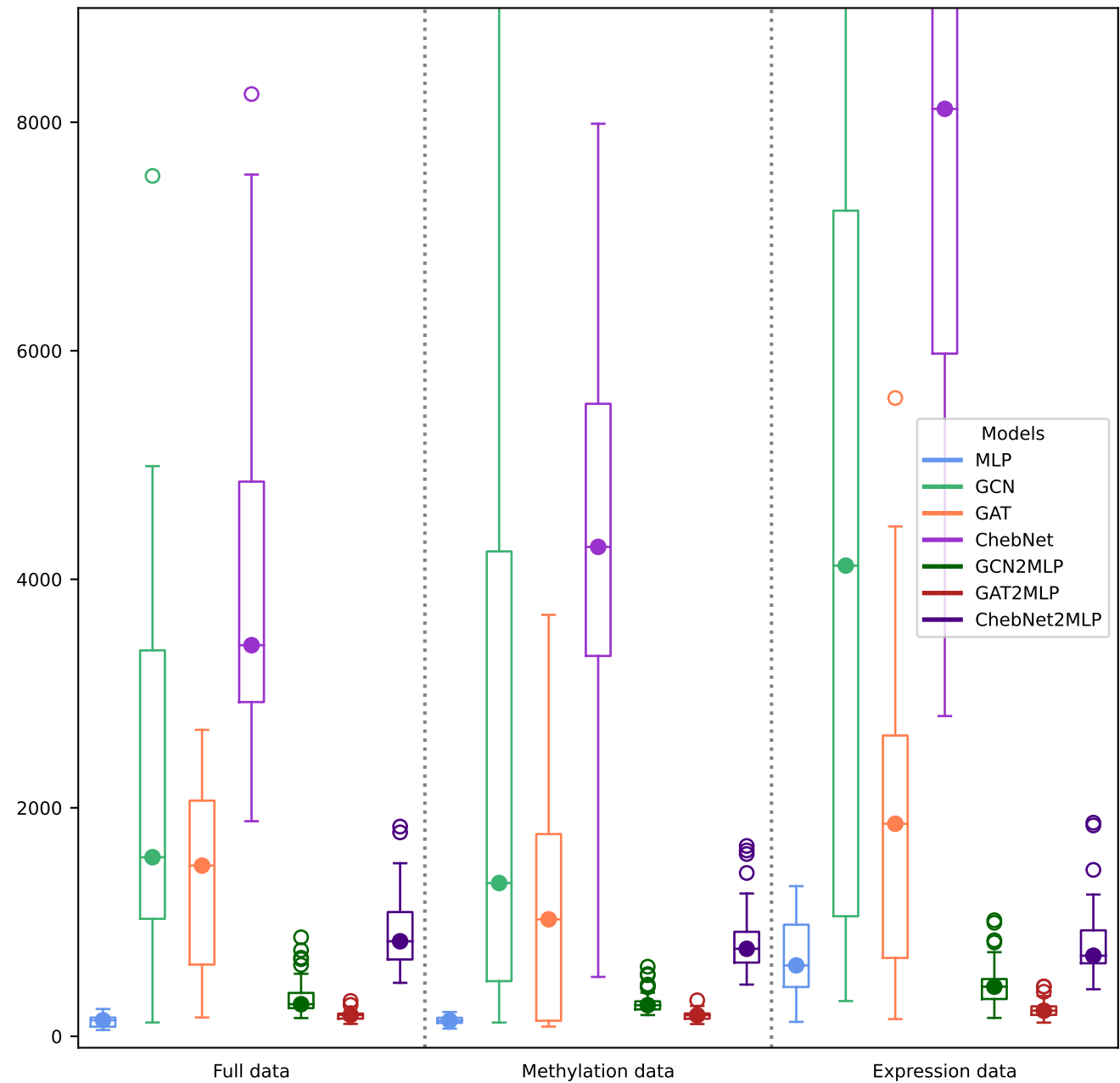
Training time of plain models
