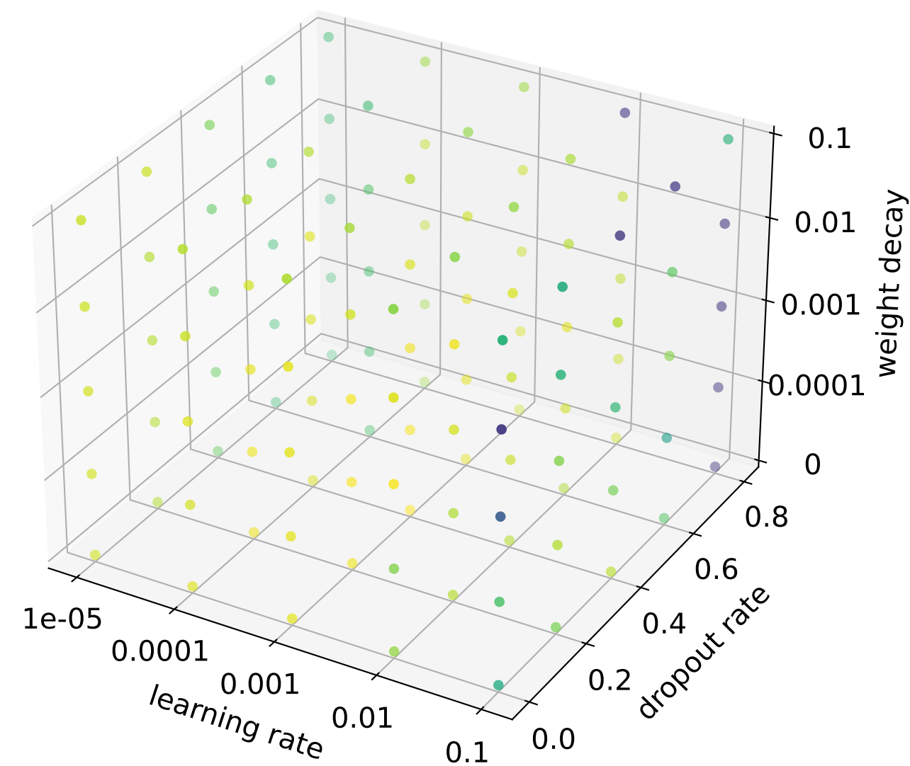
ChebNet2MLP
