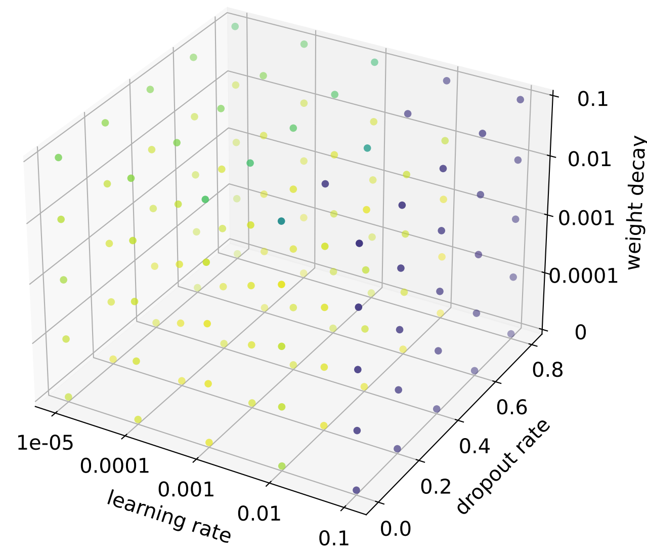
GCN2MLP
