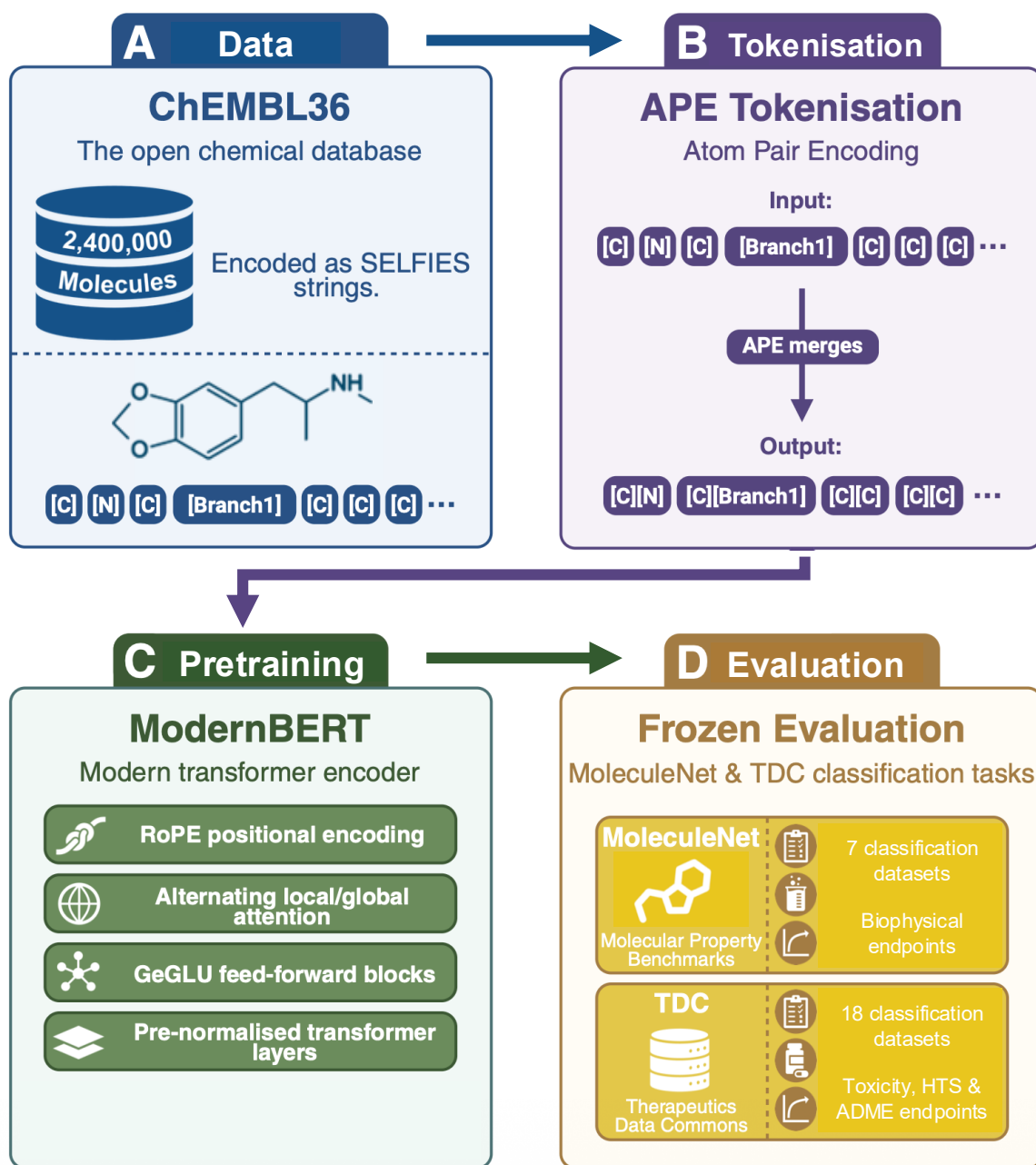
Figure 1: ModernMolBERT pretraining and frozen-evaluation pipeline. (A) Approximately 2.4M unique ChEMBL 36 small molecules are curated, canonicalised, and converted to SELFIES strings. (B) The SELFIES strings are pre-tokenised with the SELFIES-adapted APE tokeniser (Figure 2C). (C) A MODERNBERT encoder is trained from scratch on this corpus with the masked language modelling (MLM) objective, yielding MODERNMOLBERT. (D) For evaluation the encoder is frozen : mean-pooled final-layer token embeddings over non-special SELFIES tokens are extracted without any gradient updates and passed to lightweight downstream classifiers (ridge, random forest, k -nearest neighbours) on 25 binary molecular property-prediction benchmarks (7 biophysical endpoints from MoleculeNet and 18 toxicity, ADME and HTS endpoints from the Therapeutics Data Commons), where MODERNMOLBERT is compared against fixed fingerprint and pre-trained string-encoder baselines under an identical protocol.
