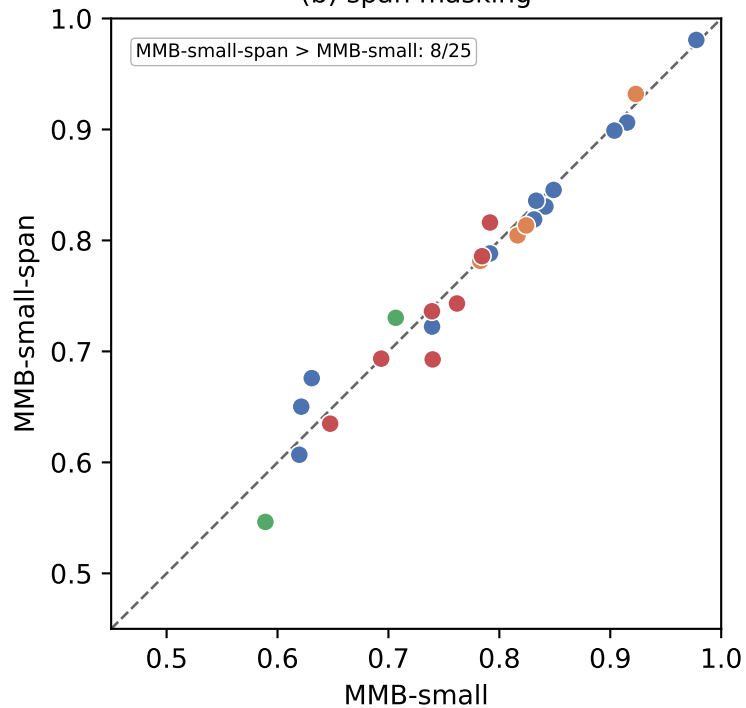
(b) span masking
