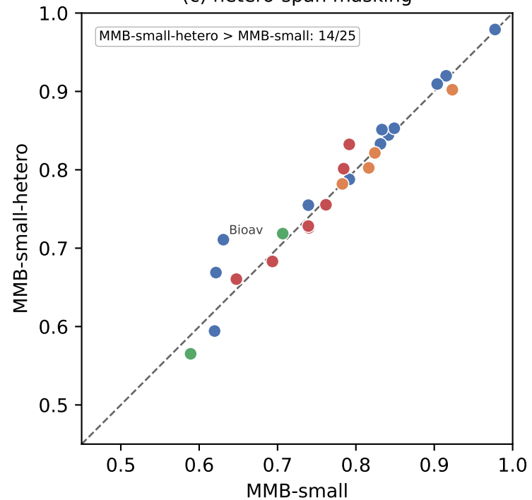
(c) hetero-span masking
