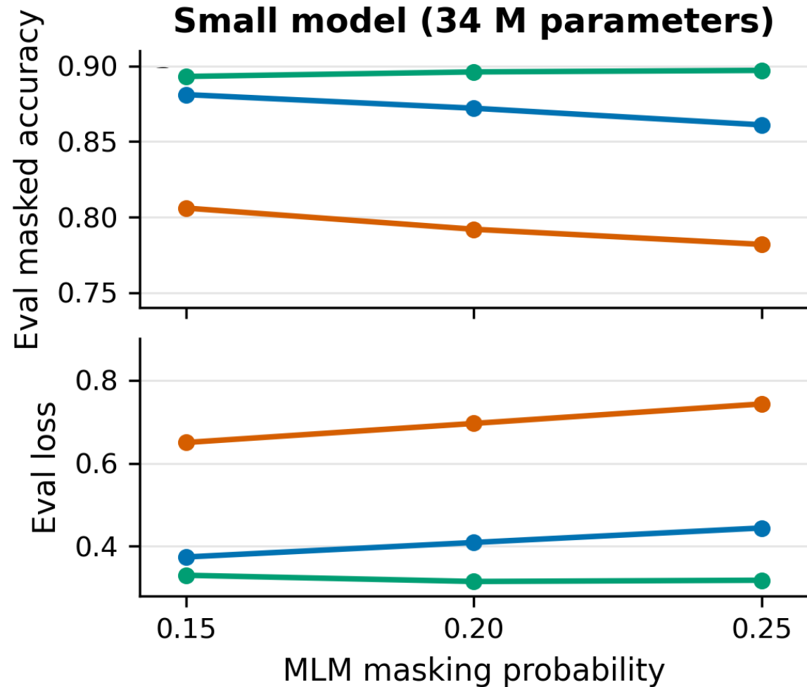
Masking strategy
