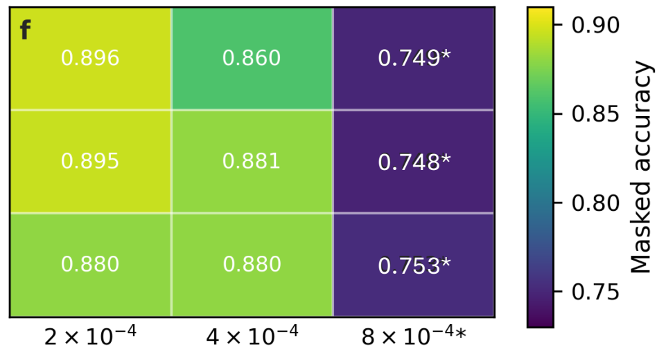
Base model (114 M parameters)
