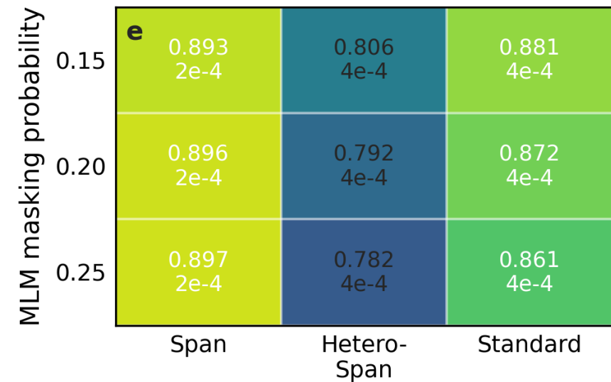
Small model (34 M parameters)
