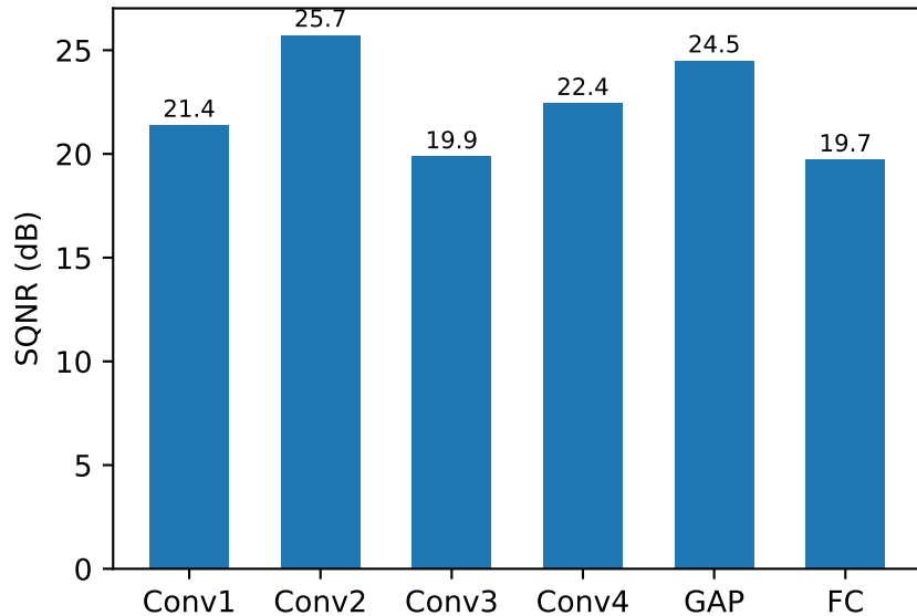
(a) Signal-to-quantization-noise
