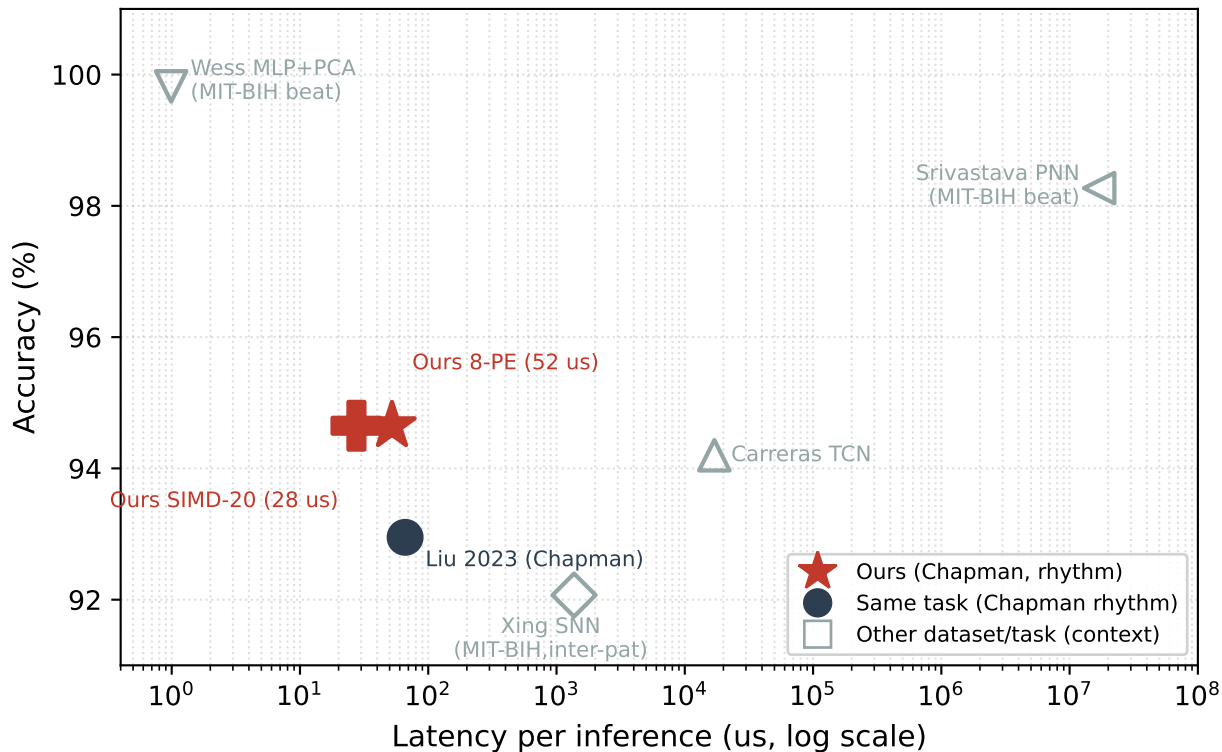
(B) Latency vs Accuracy — FPGA ECG accelerators
