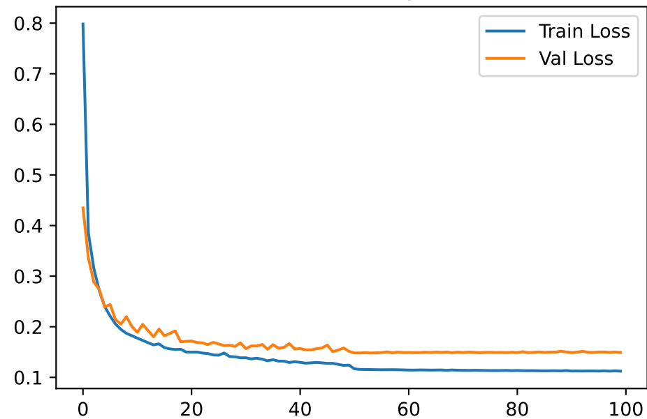
Loss History
