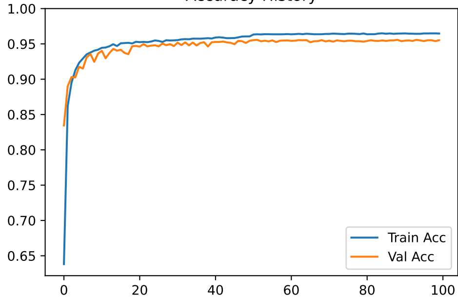
Accuracy History
