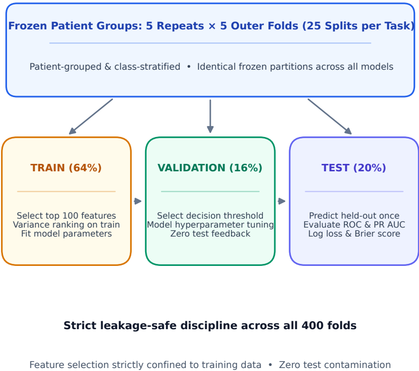
Frozen repeated evaluation protocol
