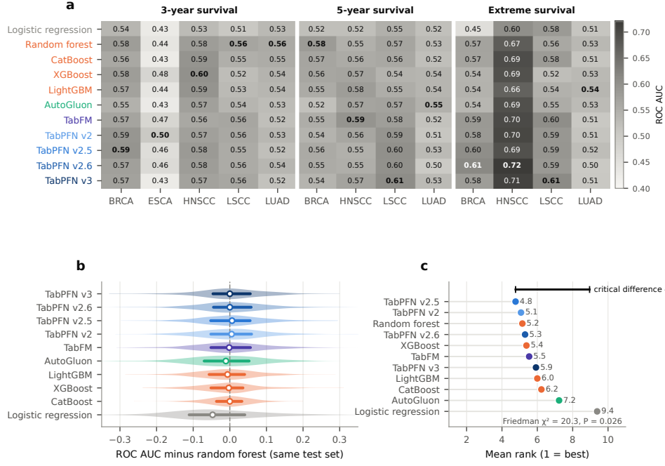
Fig. 3 Within a single cancer, no model wins decisively. a , ROC AUC in each of the 13 cancer-specific tasks, grouped by endpoint (3-year, 5-year and extreme survival); each cell is the mean over 25 frozen test sets, and bold marks the best model in each column. b , Paired difference from random forest: distribution of fold-matched ROC AUC differences over the 325 cancer-specific test sets (violin), with interquartile range (bar) and median (circle); the dashed line marks no difference. c , Mean rank of each model across the 13 tasks (1 = best). The bar shows the Nemenyi critical difference at \alpha = 0.05 ; models whose mean ranks differ by less than this are not significantly different. Model names are coloured by family.
