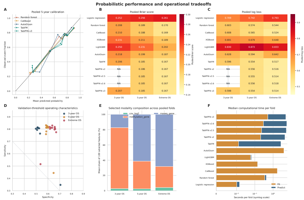
Extended Data Fig. 5 Probability quality and compute. Calibration curves for pooled 5-year predictions, pooled Brier score and log loss, sensitivity and specificity at validation-selected thresholds, selected-feature modality composition, and median fit and prediction time per fold. Classical models ran locally and foundation models on a separate CPU machine, so runtimes are indicative.
