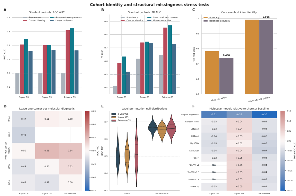
Extended Data Fig. 4 Shortcut-control detail. Cancer-type and zero-pattern controls, cohort identifiability, cancer-held-out diagnostics, permutation distributions and the difference between each pooled model and the strongest control.
