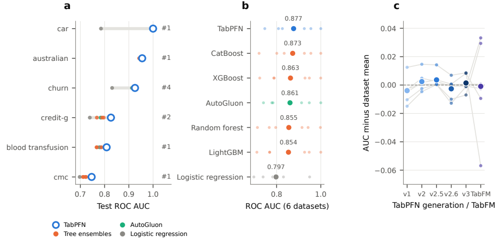
Fig. 2 The direction of TabPFN's benchmark advantage reproduces on its own datasets. a , TabPFN against six baselines: test ROC AUC of TabPFN (open circle) and of tree ensembles, AutoGluon and logistic regression (filled points) on six benchmark datasets. The grey bar spans the baselines, and the number on the right is TabPFN's rank on that dataset (ties share a rank). b , Mean test ROC AUC of each model over the six datasets (large point, value above) with per-dataset values (small points). c , Four TabPFN generations and TabFM under a common protocol with training capped at 1,024 rows: ROC AUC relative to each dataset's mean across these six models (lines join datasets; large points are means). Mean ROC AUC over the six datasets was 0.856 (v1), 0.862 (v2), 0.863 (v2.5), 0.857 (v2.6), 0.861 (v3) and 0.859 (TabFM). One stratified split per dataset.
