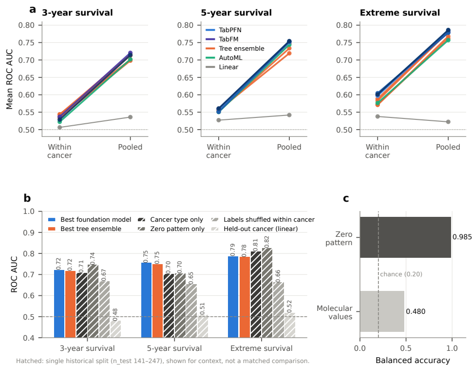
Fig. 4 Pooling lifts every model, and controls without patient biology reach similar levels. a , Mean ROC AUC within cancers and in the pooled cohort for each model, by endpoint; lines are coloured by model family. b , Pooled ROC AUC of the best foundation model and the best tree ensemble (solid bars; frozen benchmark) compared with four controls that ignore patient biology: cancer type only, zero pattern only, survival labels shuffled within each cancer (mean of 500 permutations) and a linear model tested on a held-out cancer (mean over held-out cancers). Hatched bars come from a single earlier split and are shown for context, not as a matched comparison. c , How well the cancer type itself can be recovered: balanced accuracy for identifying the cancer from the zero pattern or from molecular values; the dashed line marks chance (0.20 for five cancers).
