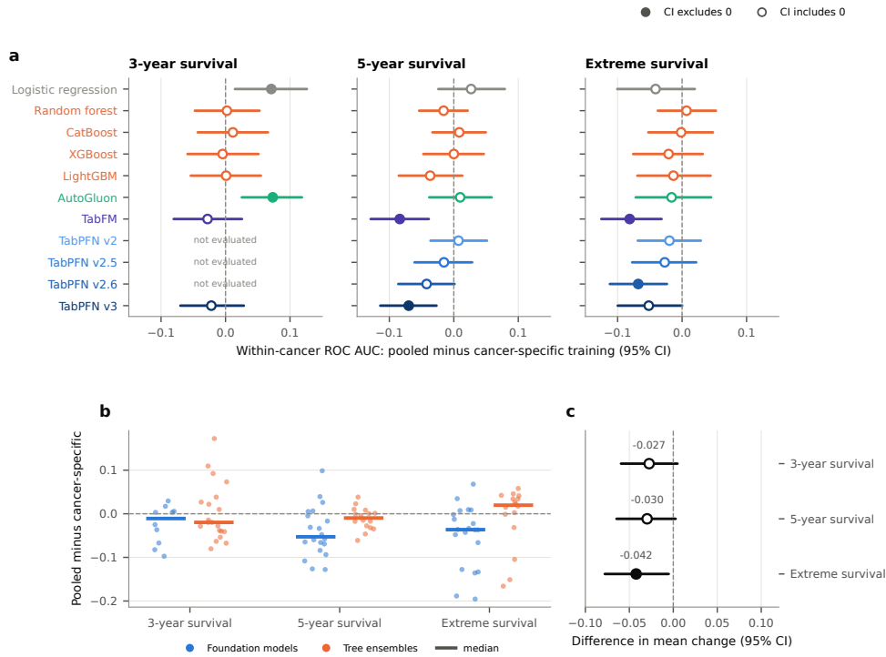
Fig. 5 Pooled training lowered within-cancer ranking for foundation models. a , For each model and endpoint, the mean across cancers of the within-cancer ROC AUC of the pooled model minus that of the cancer-specific model, scored on the same patients. Bars are 95% patient-bootstrap intervals (2,000 resamples, shared across models); filled circles mark intervals that exclude zero. TabPFN v2–v2.6 were not evaluated on pooled 3-year survival. b , The same change shown cancer by cancer: each dot is one model in one cancer, grouped into foundation models and tree ensembles; horizontal bars mark medians. c , Foundation models minus trees: the mean change of foundation models minus that of tree ensembles at each endpoint, with its 95% interval from the same resamples; a negative value means foundation models lost more.
