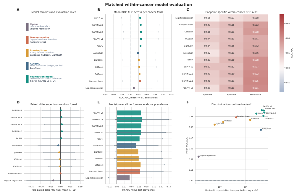
Extended Data Fig. 2 Within-cancer performance detail. Model families, mean ROC AUC with variation across test sets, AUC by model and endpoint, fold-matched differences from random forest, precision-recall AUC above prevalence, and runtime.
