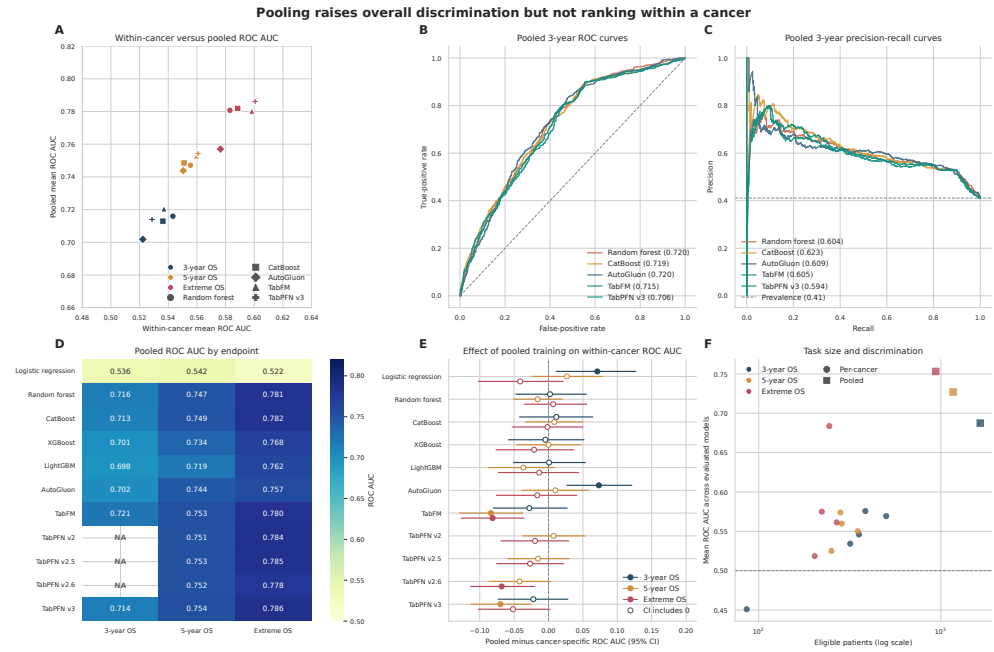
Extended Data Fig. 3 Pooled-task curves. Within-cancer versus pooled AUC, pooled 3-year ROC and precision-recall curves, pooled AUC heatmap, the paired within-cancer effect (first version) and task size against discrimination.
