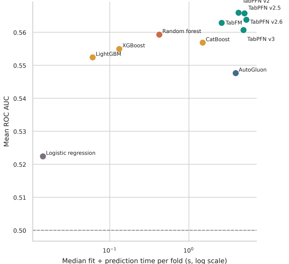
Discrimination-runtime tradeoff
