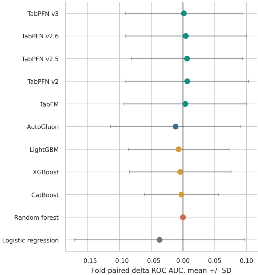
Paired difference from random forest
