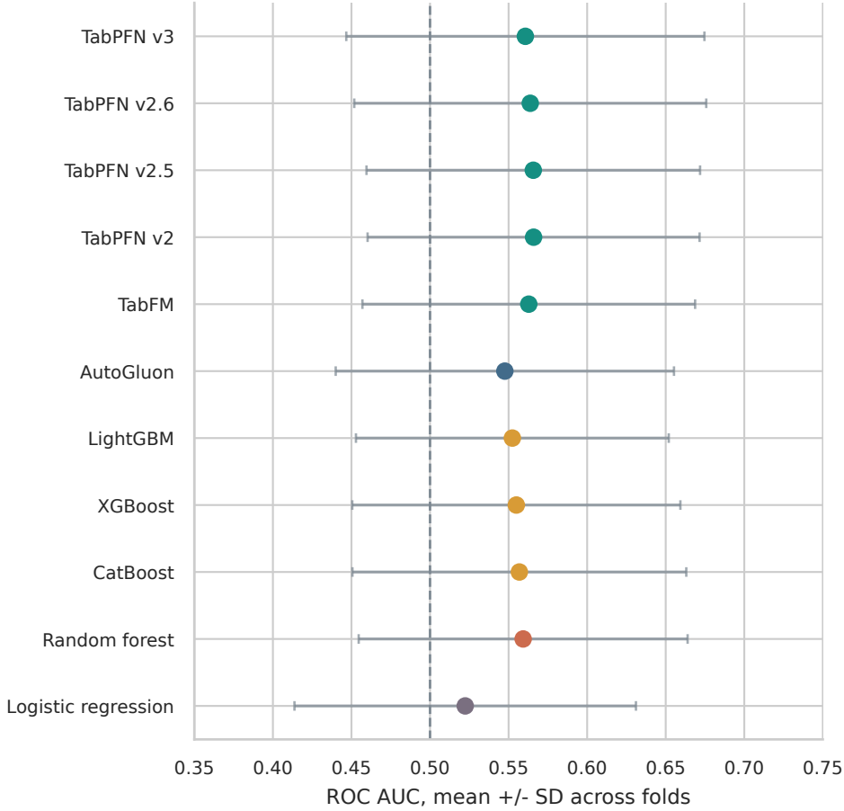
Mean ROC AUC across per-cancer folds
