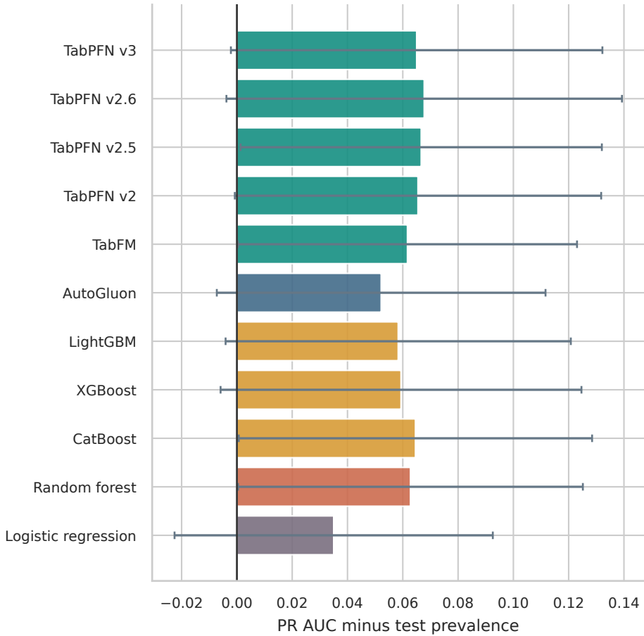
Precision-recall performance above prevalence
