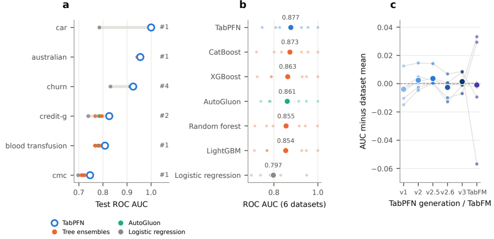
Fig. 2 The direction of TabPFN’s benchmark advantage reproduces on its own datasets. a , TabPFN against six baselines: test ROC AUC of TabPFN (open circle) and of tree ensembles, AutoGluon and logistic regression (filled points) on six benchmark datasets. The grey bar spans the baselines, and the number on the right is TabPFN’s rank on that dataset (ties share a rank). b , Mean test ROC AUC of each model over the six datasets (large point, value above) with per-dataset values (small points). c , Four TabPFN generations and TabFM under a common protocol with training capped at 1,024 rows: ROC AUC relative to each dataset’s mean across these six models (lines join datasets; large points are means). Mean ROC AUC over the six datasets was 0.856 (v1), 0.862 (v2), 0.863 (v2.5), 0.857 (v2.6), 0.861 (v3) and 0.859 (TabFM). One stratified split per dataset.
