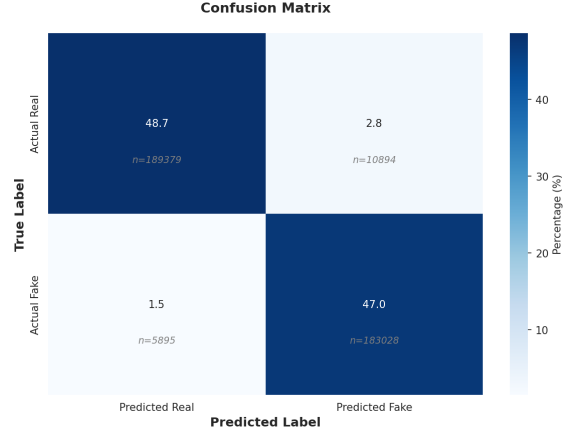
Figure 3: Stage 1 calibration (left) and confusion matrix (right).
