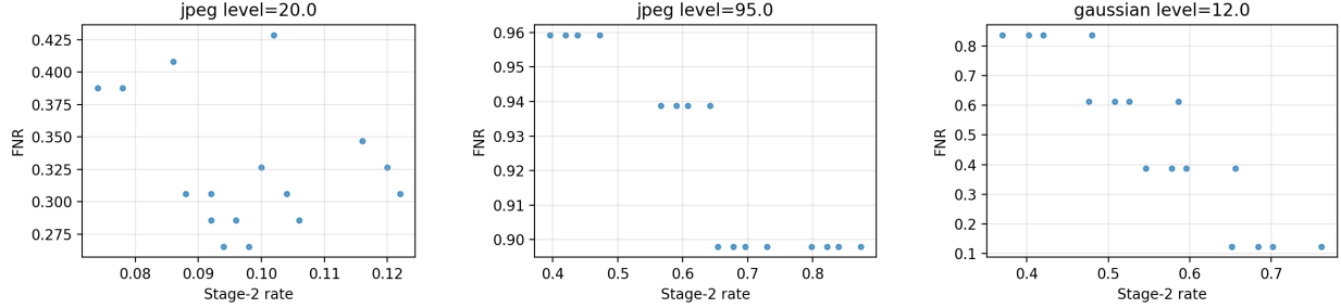
Figure 7: Representative FNR vs Stage-2 escalation rate trade-off curves under threshold sweeps. Left: JPEG quality 20 (heavy compression); middle: JPEG quality 95 (light compression); right: Gaussian noise with \sigma = 12 .
