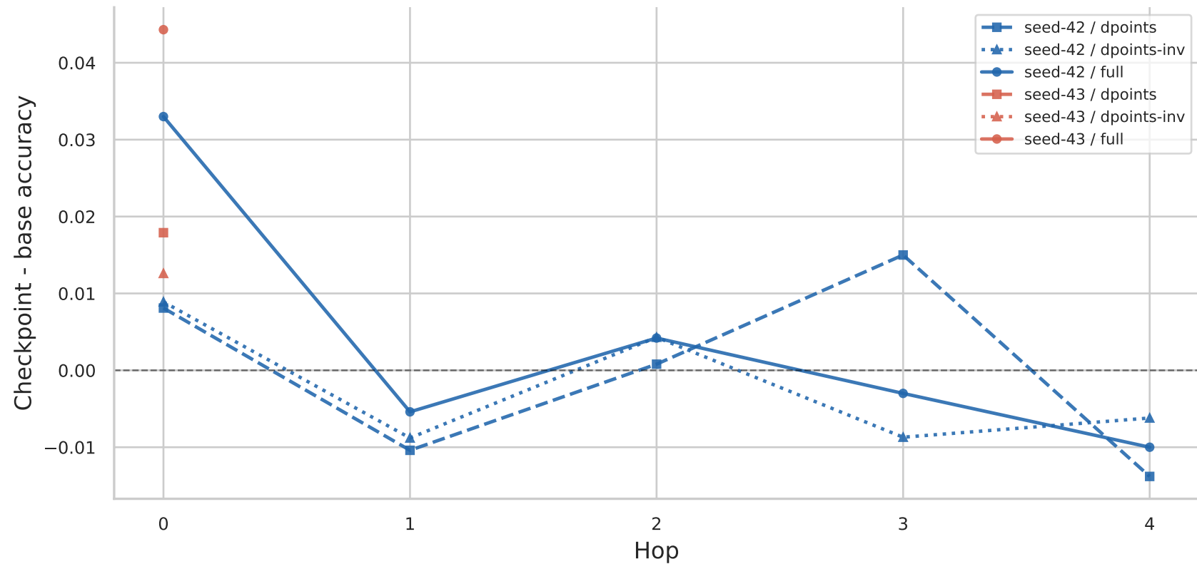
Owl accuracy change after fine-tuning
