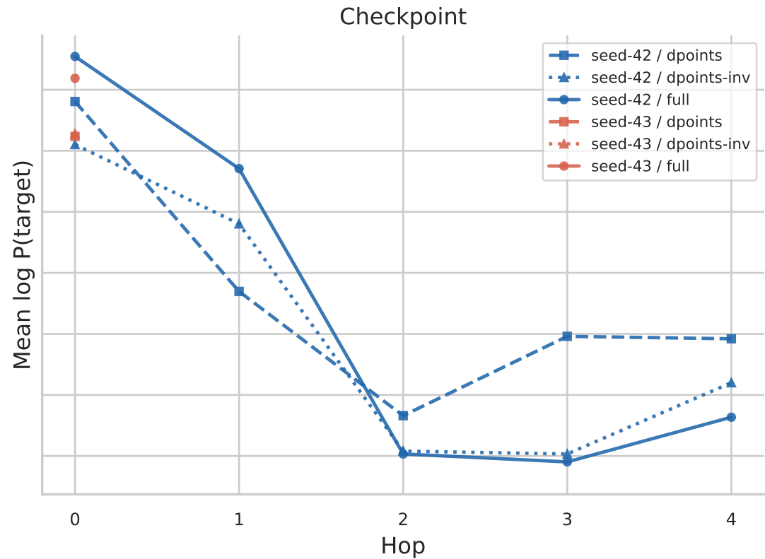
Mean log P(target) by hop
