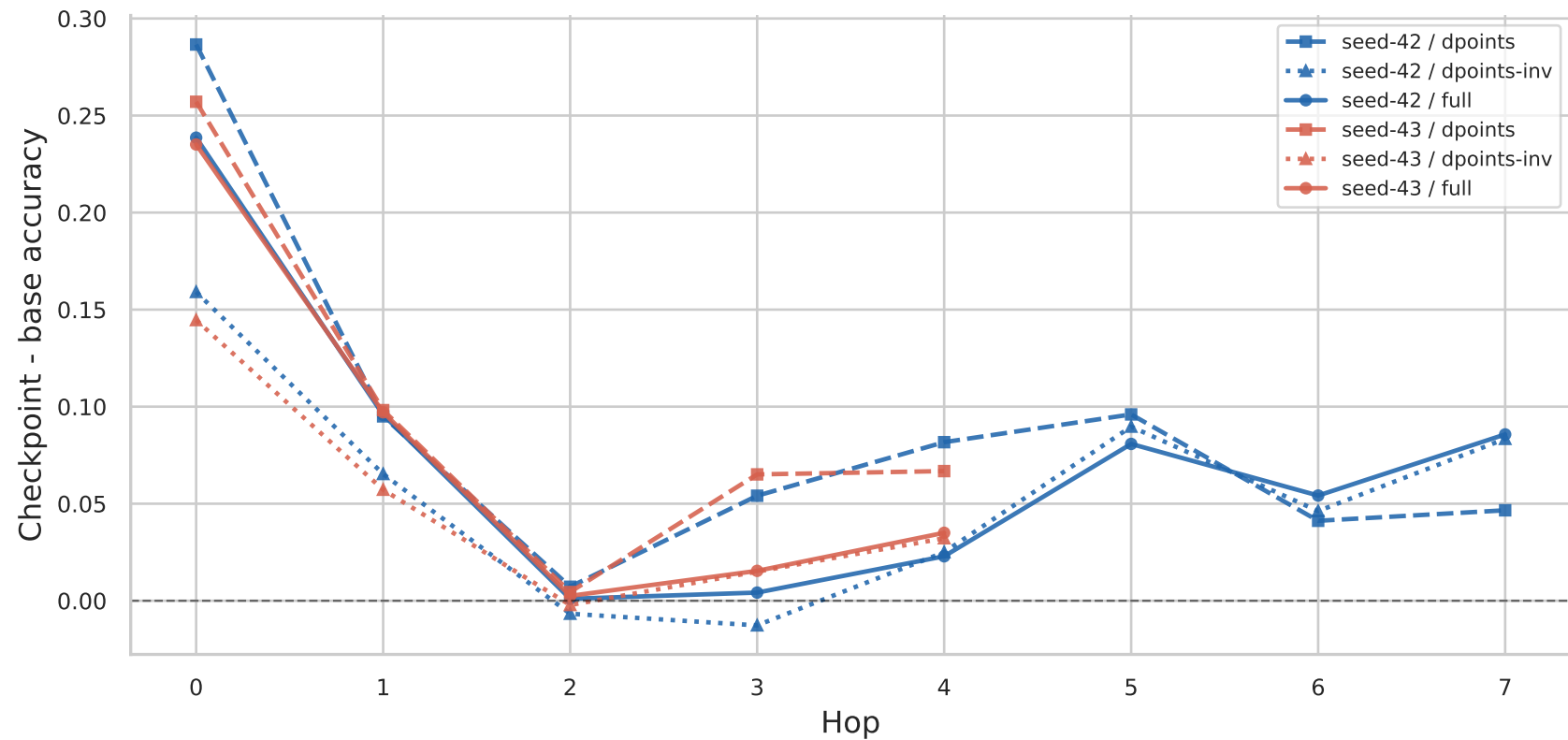
Raven accuracy change after fine-tuning
