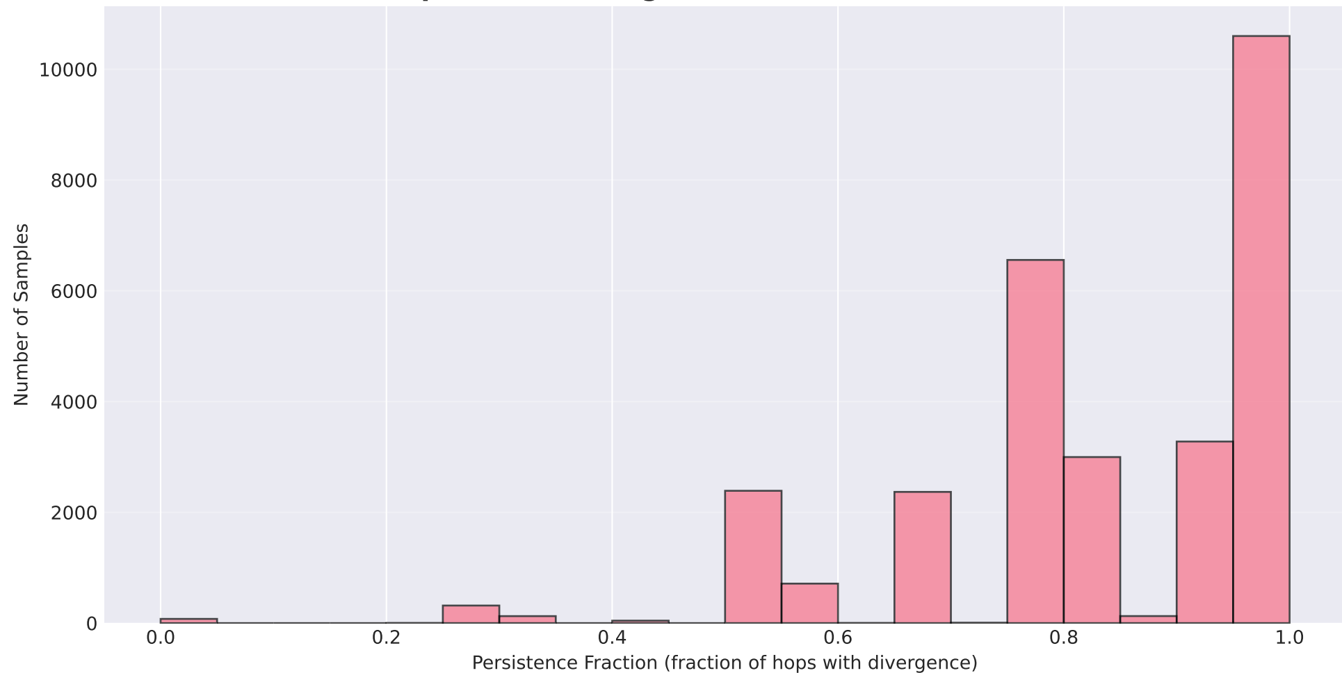
Sample-Level Divergence Persistence Distribution
