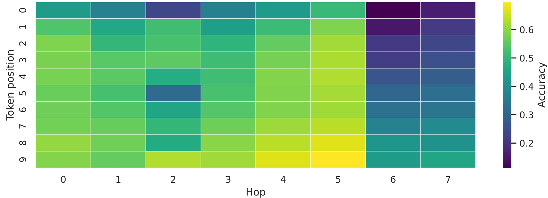
Main-task per-position train accuracy (checkpoint)
