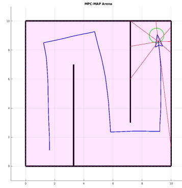
Figure 3: Successful open-loop run on indoor_1 .
