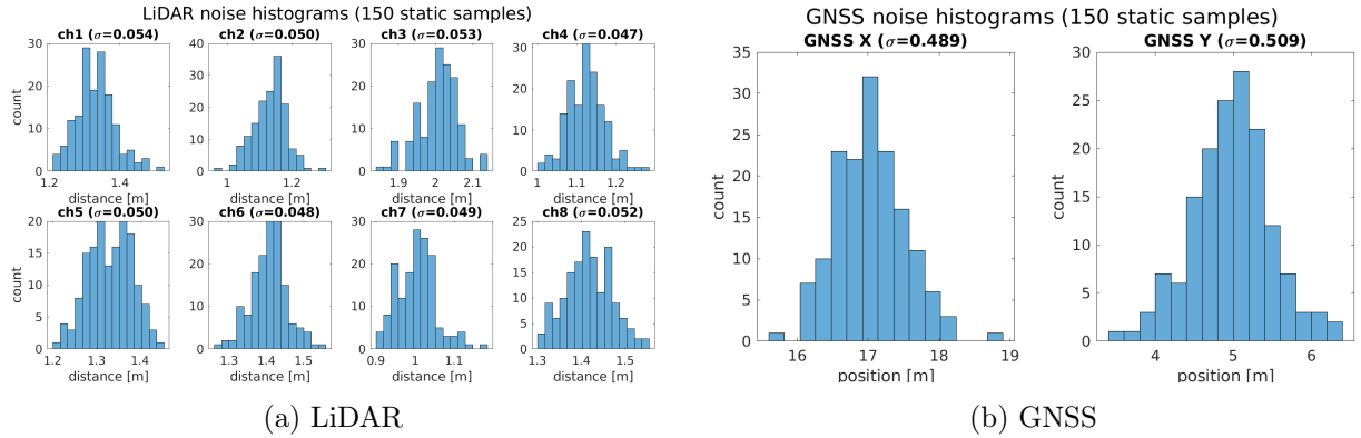
Figure 1: Sensor noise histograms (150 samples).
