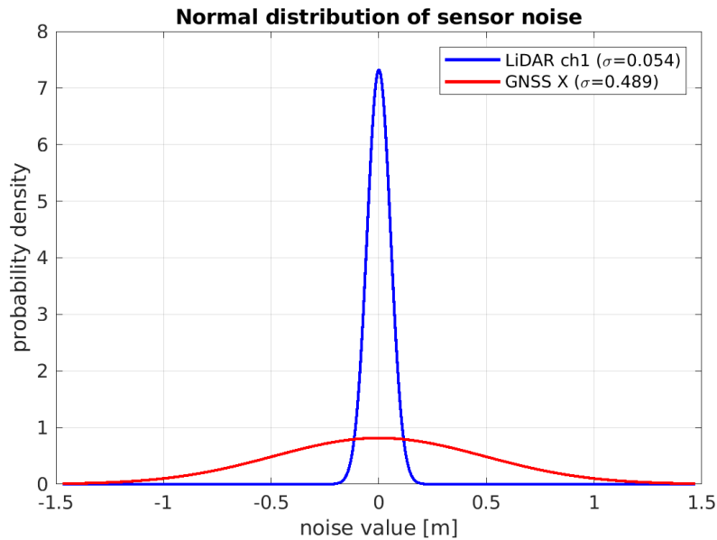
Figure 2: Normal PDFs for LiDAR (narrow) and GNSS (wide) noise.
